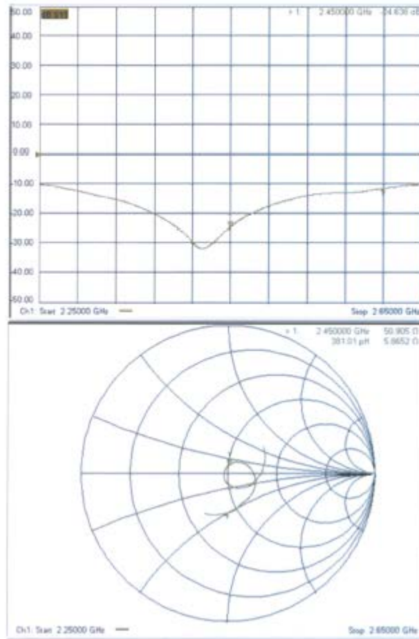
Impedance Measurement Plot for Body TSL
