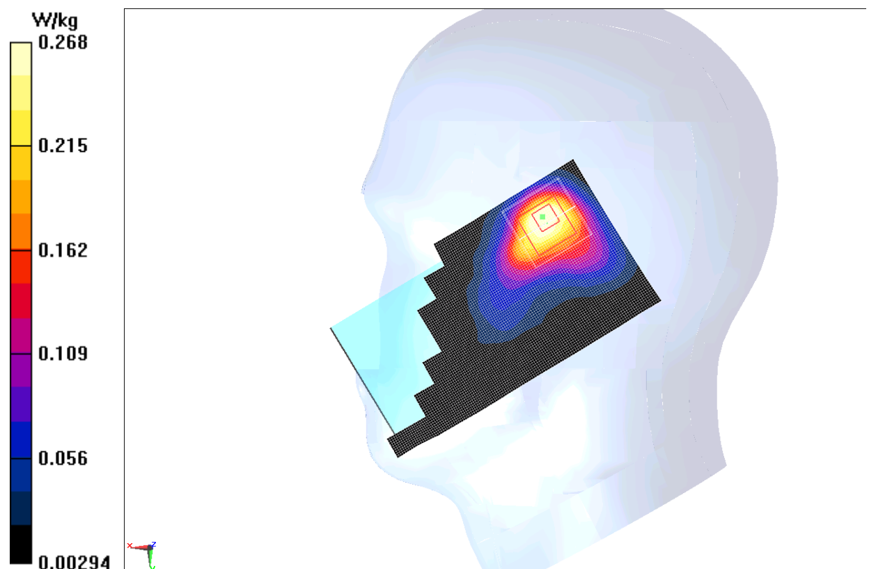
Fig.9 2450 MHz CH6
