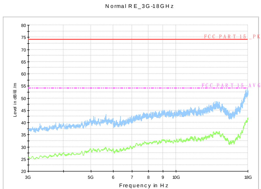
Fig.A.7.2.4 Radiated Spurious Emission (802.11b, Ch1, 3 GHz-18 GHz)
