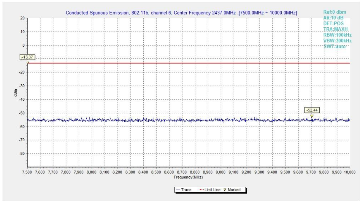
Fig.A.7.1.13 Conducted Spurious Emission (802.11b, Ch6, 7.5 GHz-10 GHz)
