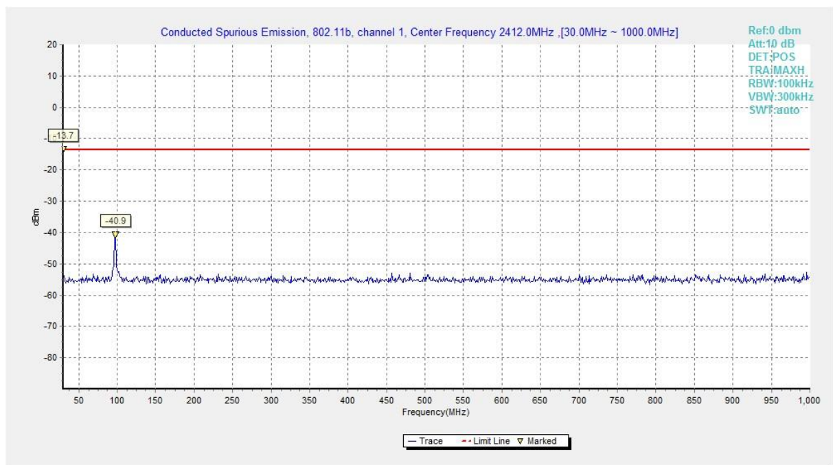
Fig.A.7.1.2 Conducted Spurious Emission (802.11b, Ch1, 30 MHz-1 GHz)
