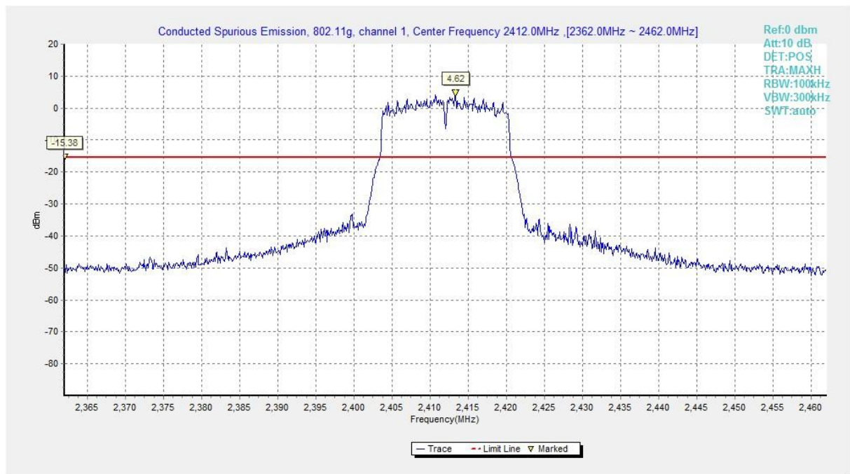
Fig.A.7.1.25 Conducted Spurious Emission (802.11g, Ch1, Center Frequency)
