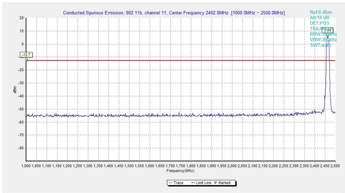
Fig.A.7.1.19 Conducted Spurious Emission (802.11b, Ch11, 1 GHz-2.5 GHz)
