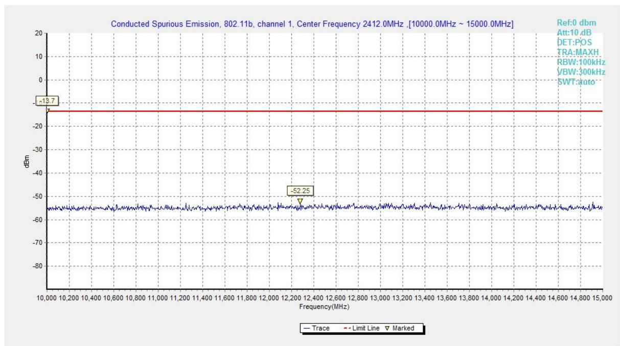
Fig.A.7.1.6 Conducted Spurious Emission (802.11b, Ch1, 10 GHz-15 GHz)
