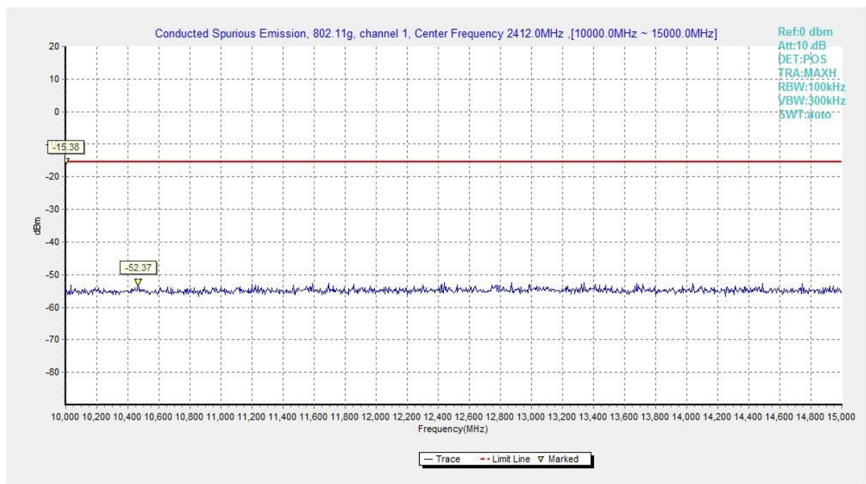
Fig.A.7.1.30 Conducted Spurious Emission (802.11g, Ch1, 10 GHz-15 GHz)
