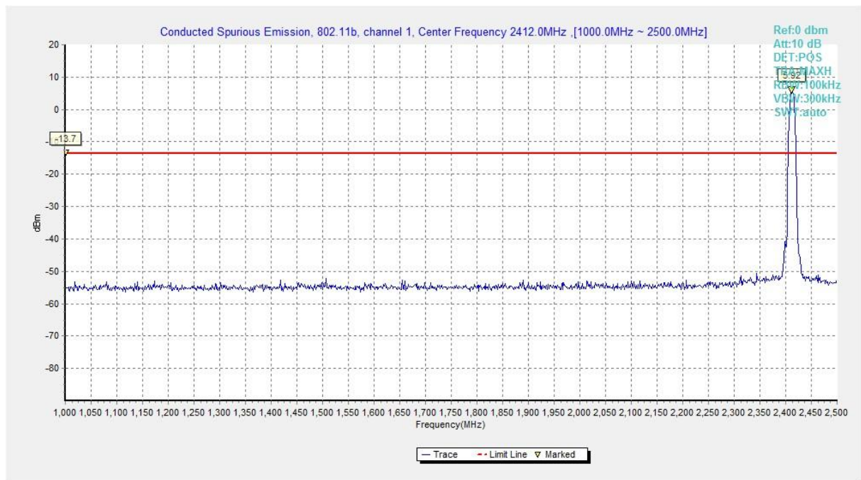
Fig.A.7.1.3 Conducted Spurious Emission (802.11b, Ch1, 1 GHz-2.5 GHz)
