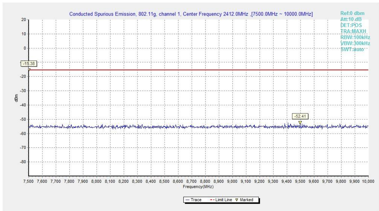
Fig.A.7.1.29 Conducted Spurious Emission (802.11g, Ch1, 7.5 GHz-10 GHz)
