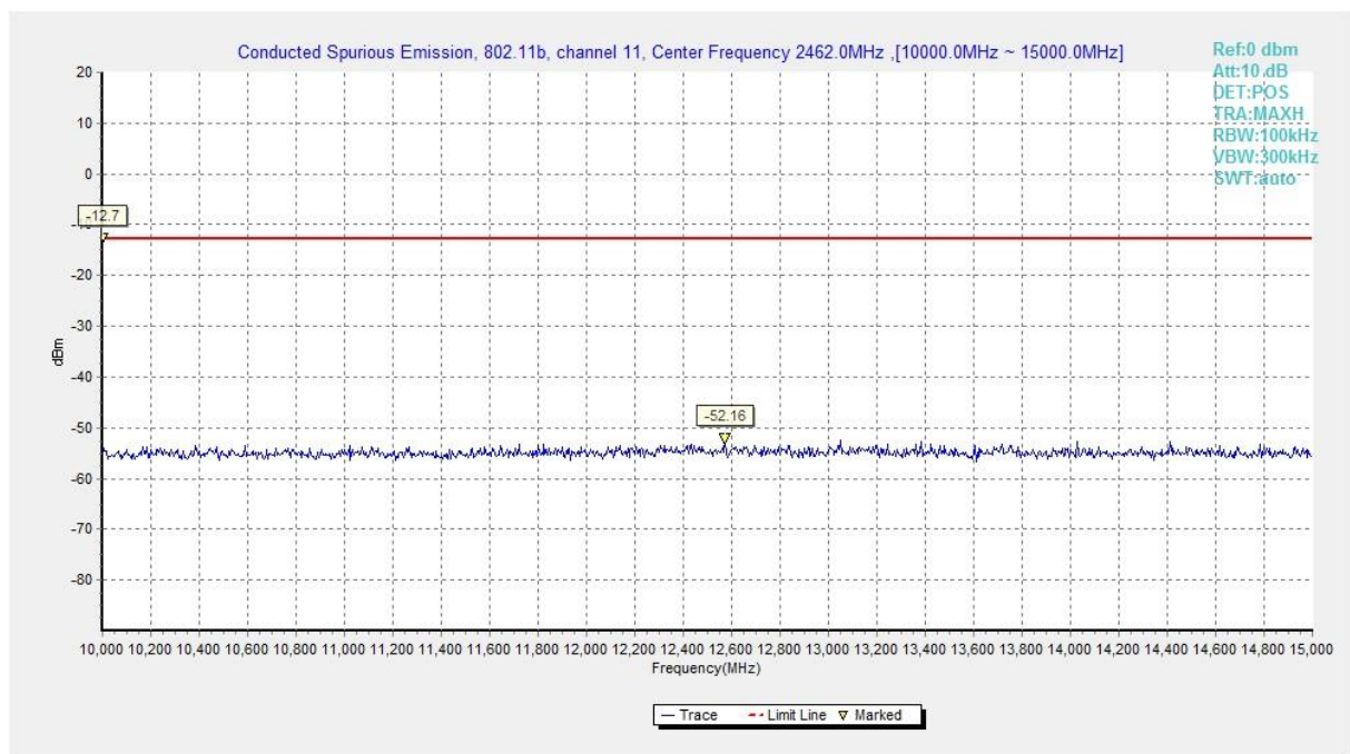
Fig.A.7.1.22 Conducted Spurious Emission (802.11b, Ch11, 10 GHz-15 GHz)
