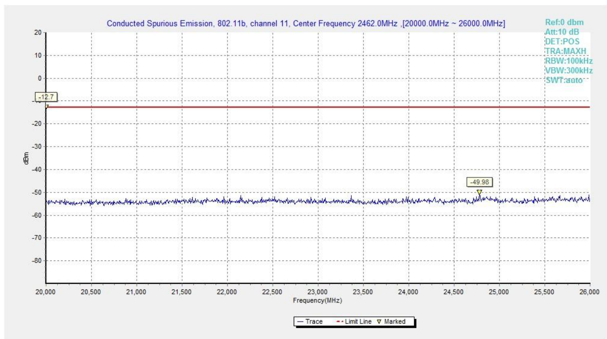
Fig.A.7.1.24 Conducted Spurious Emission (802.11b, Ch11, 20 GHz-26 GHz)
