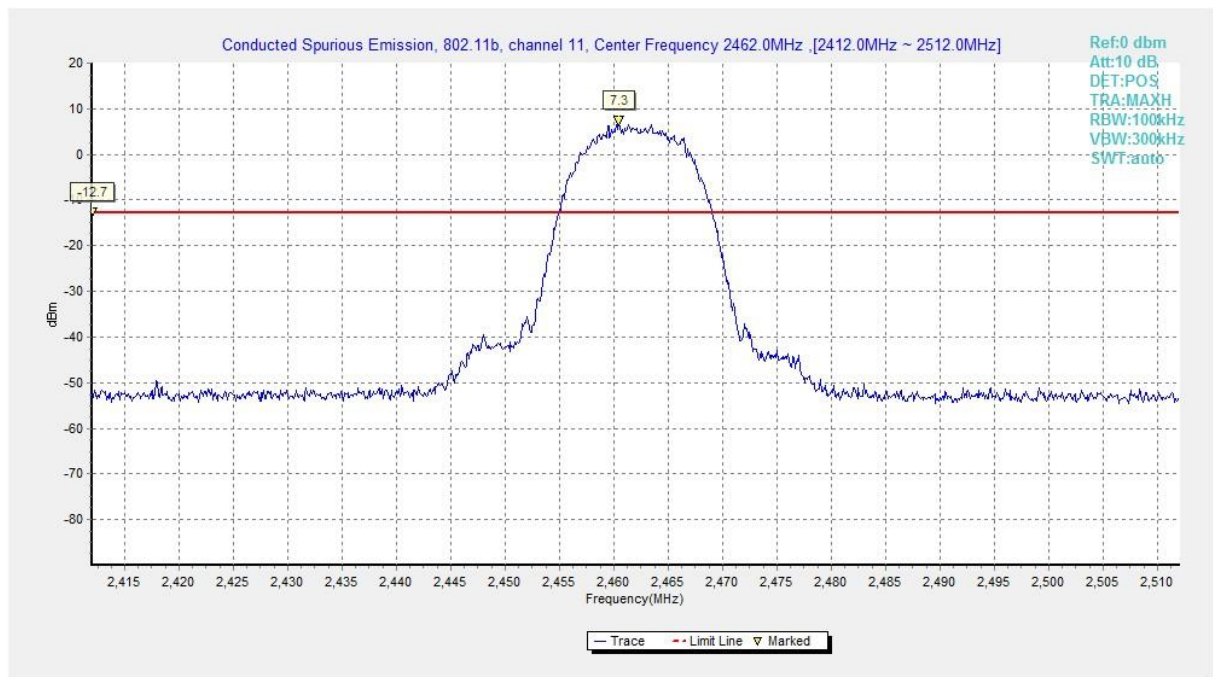
Fig.A.7.1.17 Conducted Spurious Emission (802.11b, Ch11, Center Frequency)
