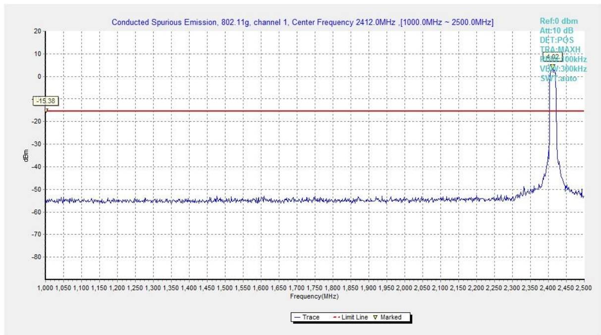
Fig.A.7.1.27 Conducted Spurious Emission (802.11g, Ch1, 1 GHz-2.5 GHz)
