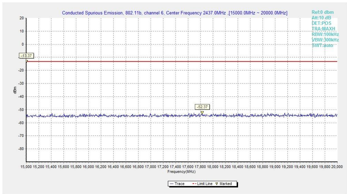
Fig.A.7.1.15 Conducted Spurious Emission (802.11b, Ch6, 15 GHz-20 GHz)
