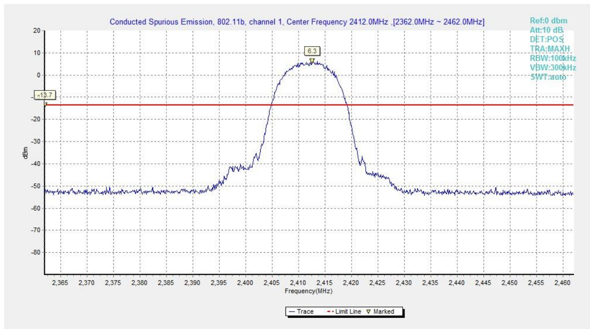
Fig.A.7.1.1 Conducted Spurious Emission (802.11b, Ch1, Center Frequency)
