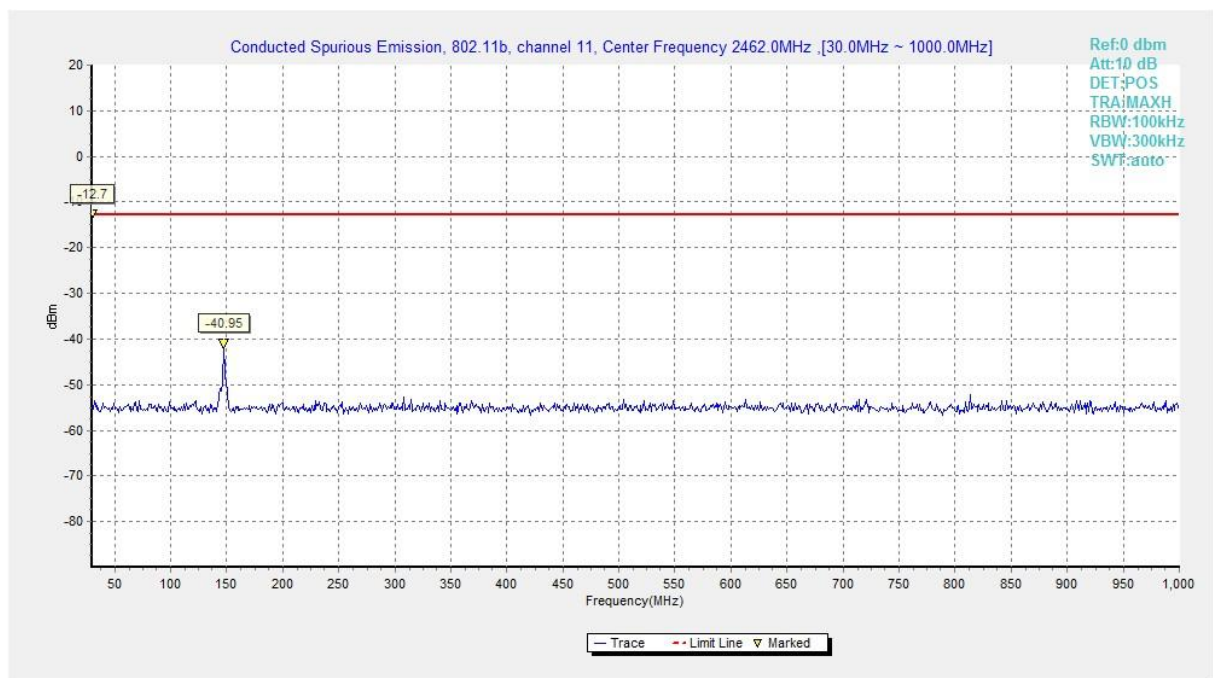
Fig.A.7.1.18 Conducted Spurious Emission (802.11b, Ch11, 30 MHz-1 GHz)
