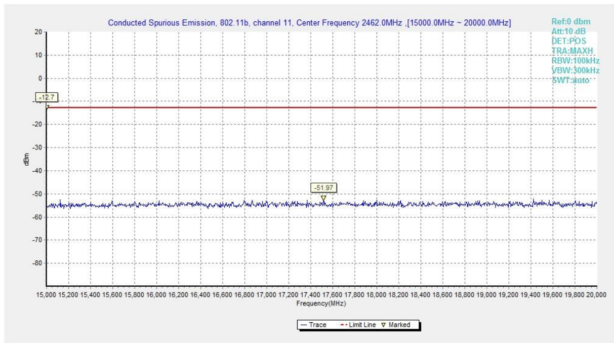
Fig.A.7.1.23 Conducted Spurious Emission (802.11b, Ch11, 15 GHz-20 GHz)
