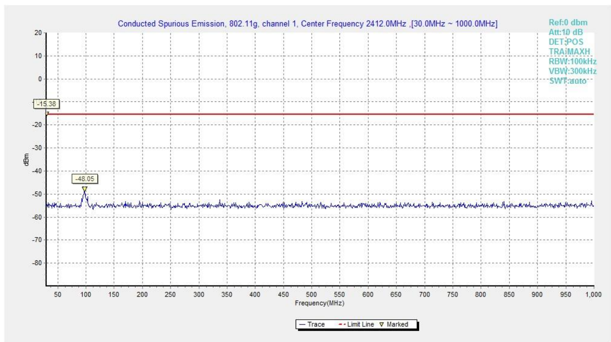
Fig.A.7.1.26 Conducted Spurious Emission (802.11g, Ch1, 30 MHz-1 GHz)
