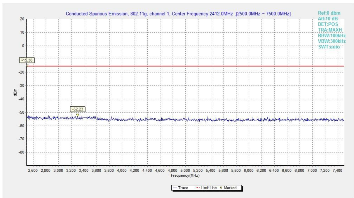
Fig.A.7.1.28 Conducted Spurious Emission (802.11g, Ch1, 2.5 GHz-7.5 GHz)
