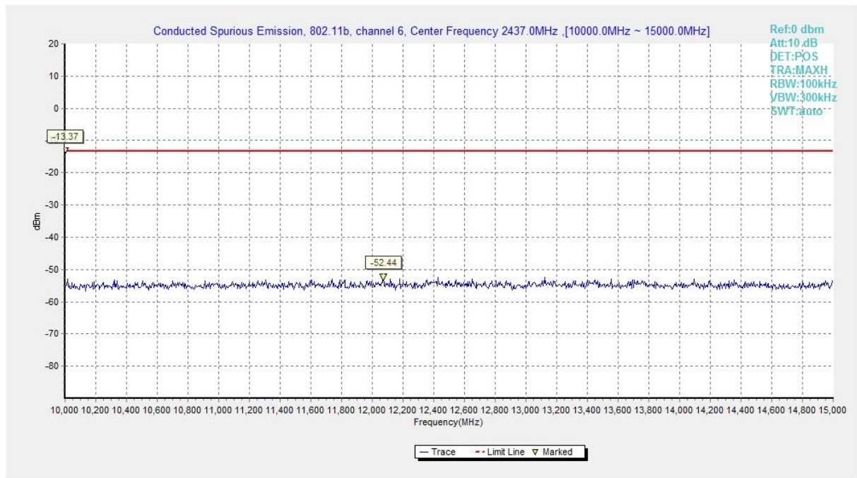
Fig.A.7.1.14 Conducted Spurious Emission (802.11b, Ch6, 10 GHz-15 GHz)
