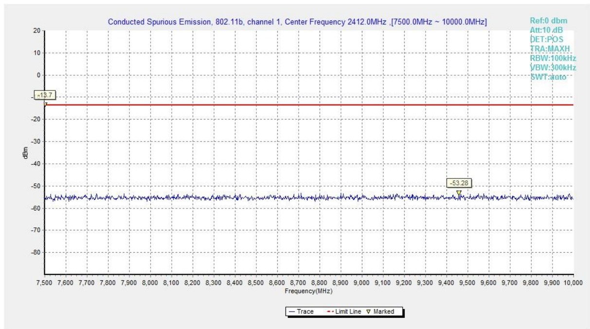
Fig.A.7.1.5 Conducted Spurious Emission (802.11b, Ch1, 7.5 GHz-10 GHz)
