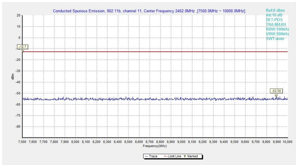
Fig.A.7.1.21 Conducted Spurious Emission (802.11b, Ch11, 7.5 GHz-10 GHz)
