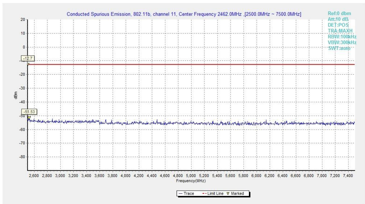
Fig.A.7.1.20 Conducted Spurious Emission (802.11b, Ch11, 2.5 GHz-7.5 GHz)
