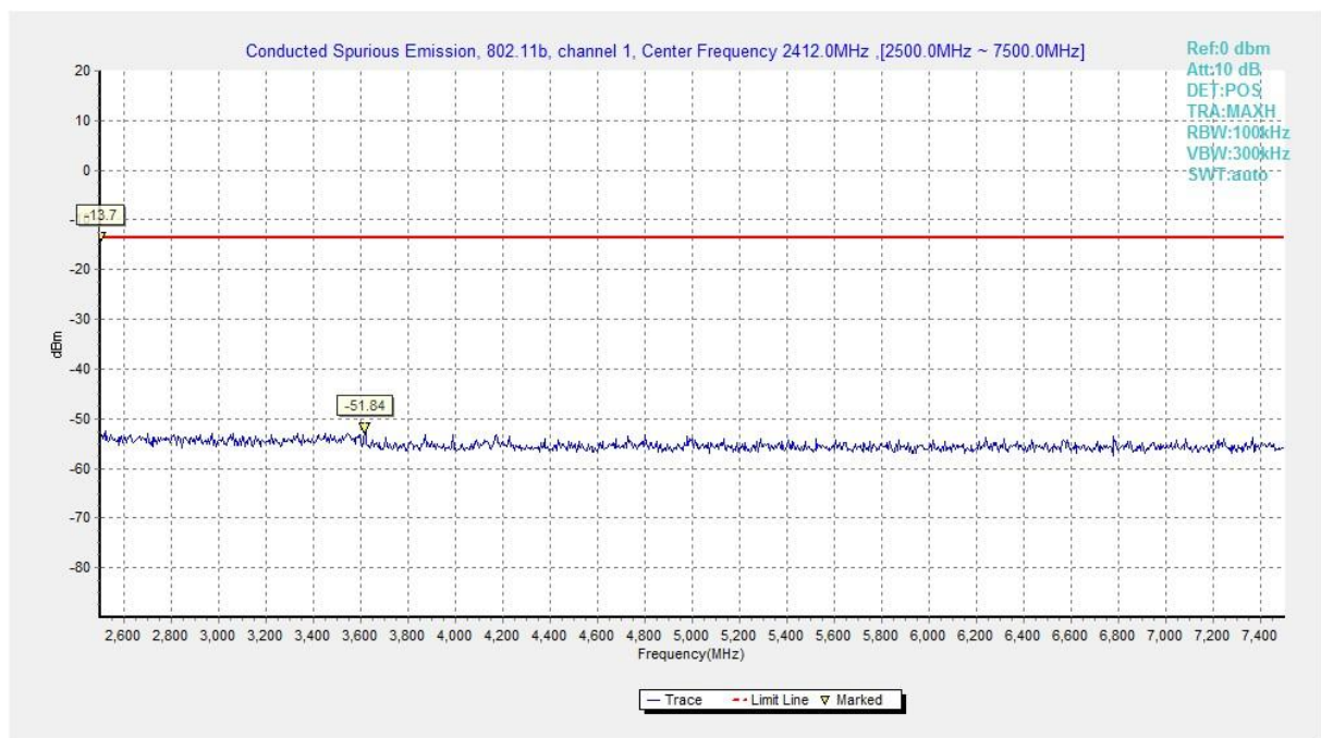
Fig.A.7.1.4 Conducted Spurious Emission (802.11b, Ch1, 2.5 GHz-7.5 GHz)
