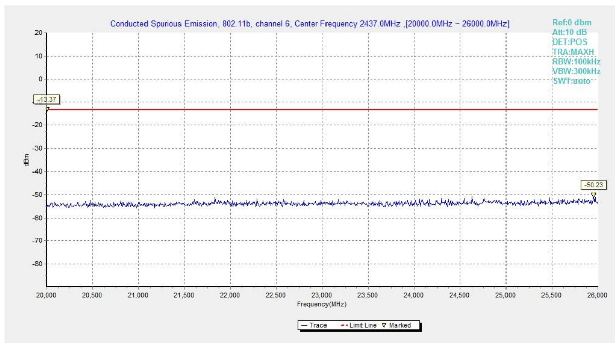
Fig.A.7.1.16 Conducted Spurious Emission (802.11b, Ch6, 20 GHz-26 GHz)
