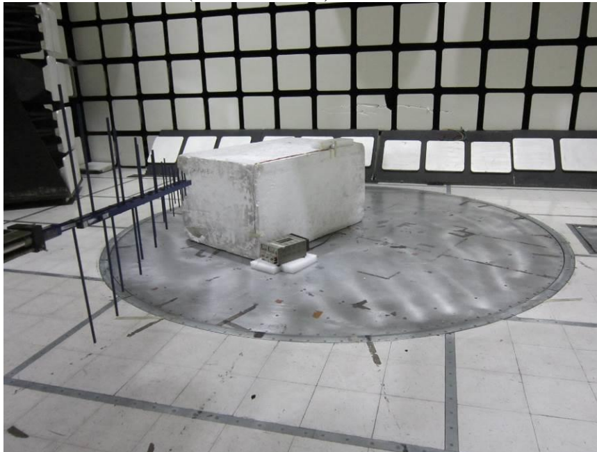
RADIATED PHOTO (BELOW 1 GHz) 3m – Wired
