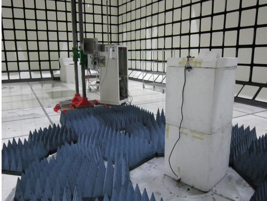
RADIATED PHOTO (ABOVE 1 GHz) – Dimmer2 and Bypass2
