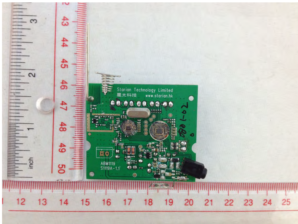
RX BOARD TOP VIEW 2
