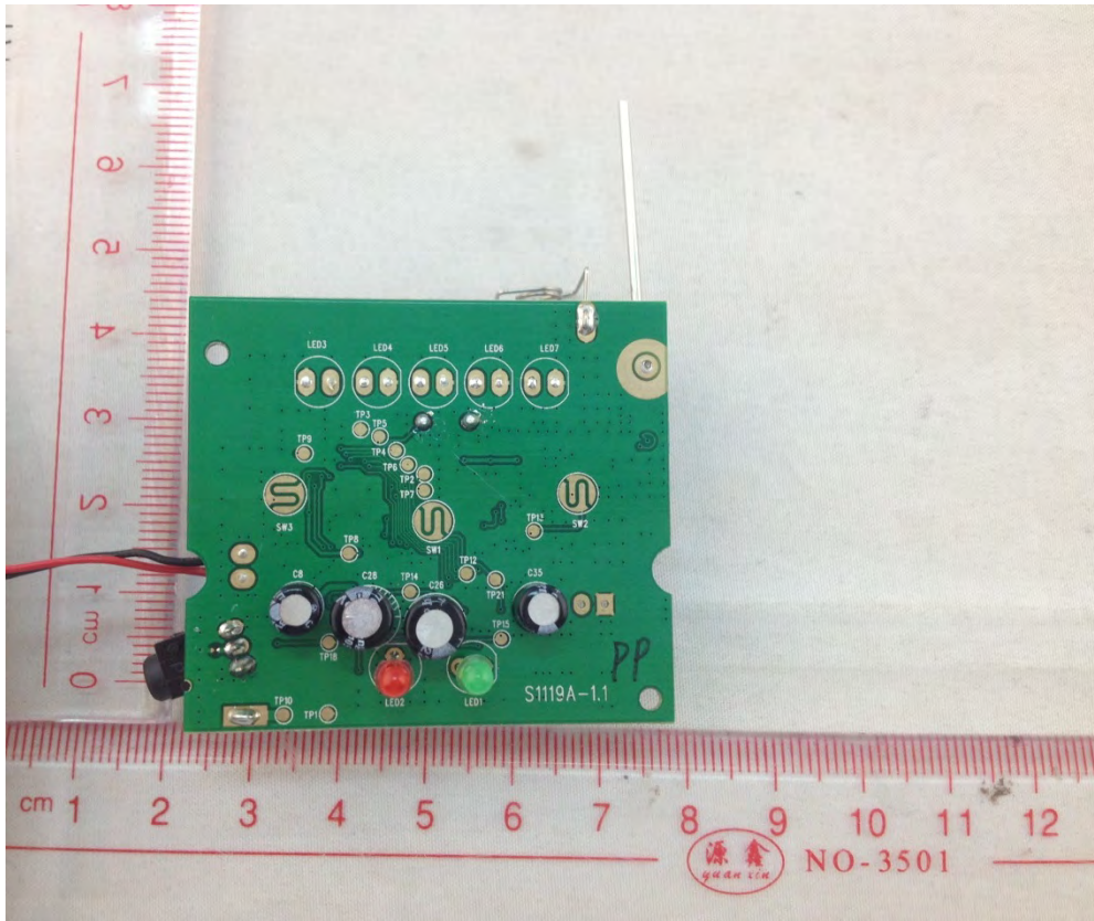
RX BOARD BACK VIEW
