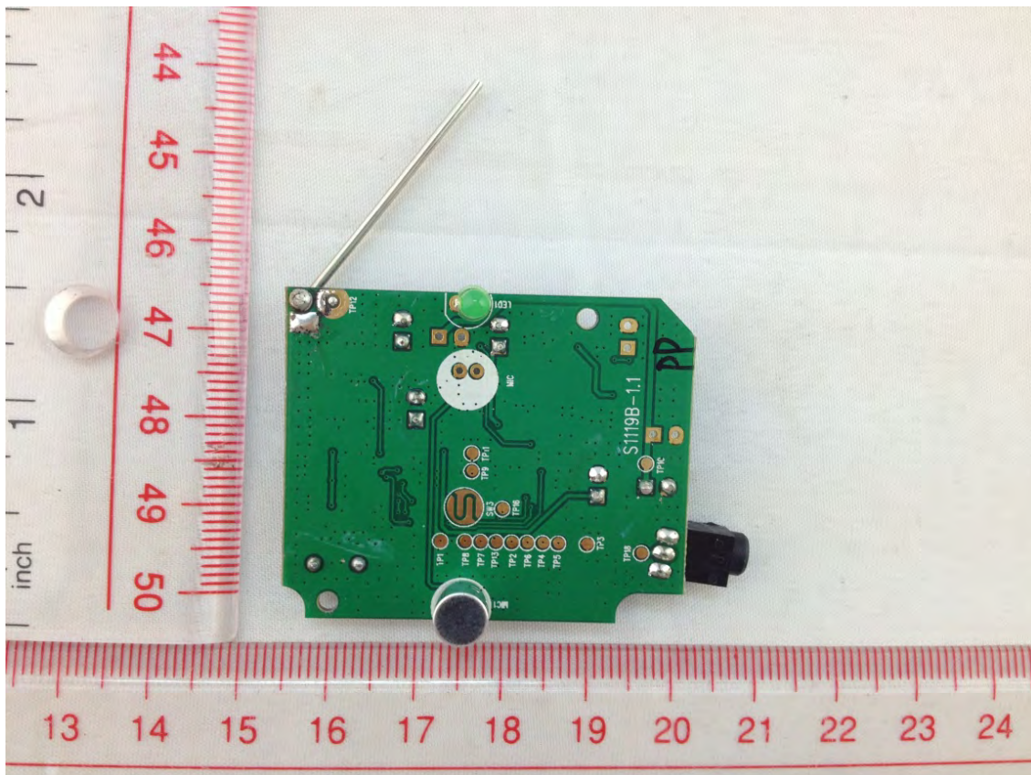
TX BOARD BACK VIEW
