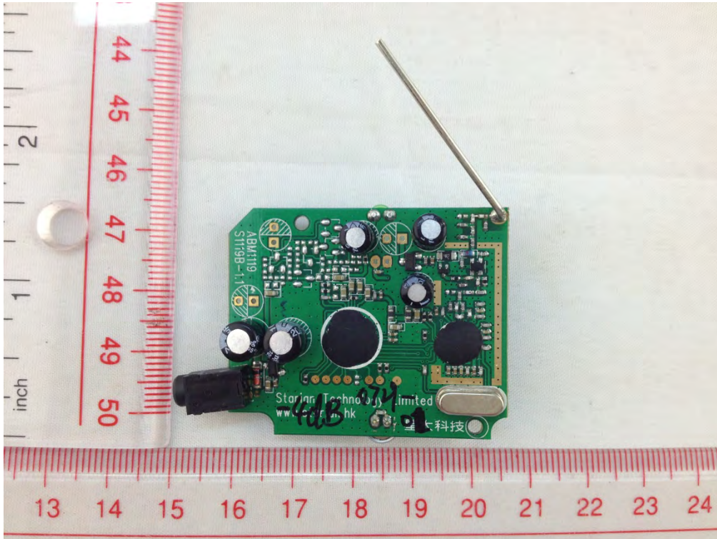
TX BOARD TOP VIEW 1
