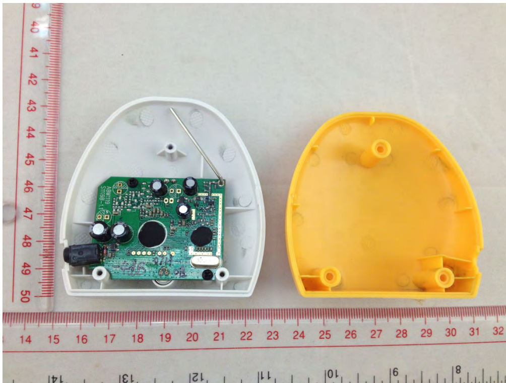
TX UNCOVER VIEW
