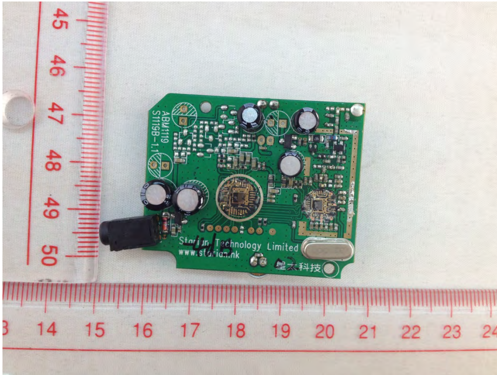
TX BOARD TOP VIEW 2
