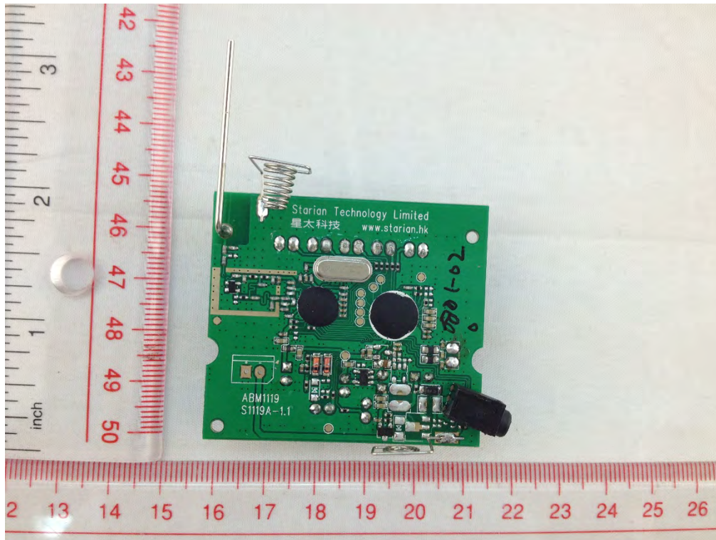
RX BOARD TOP VIEW 1
