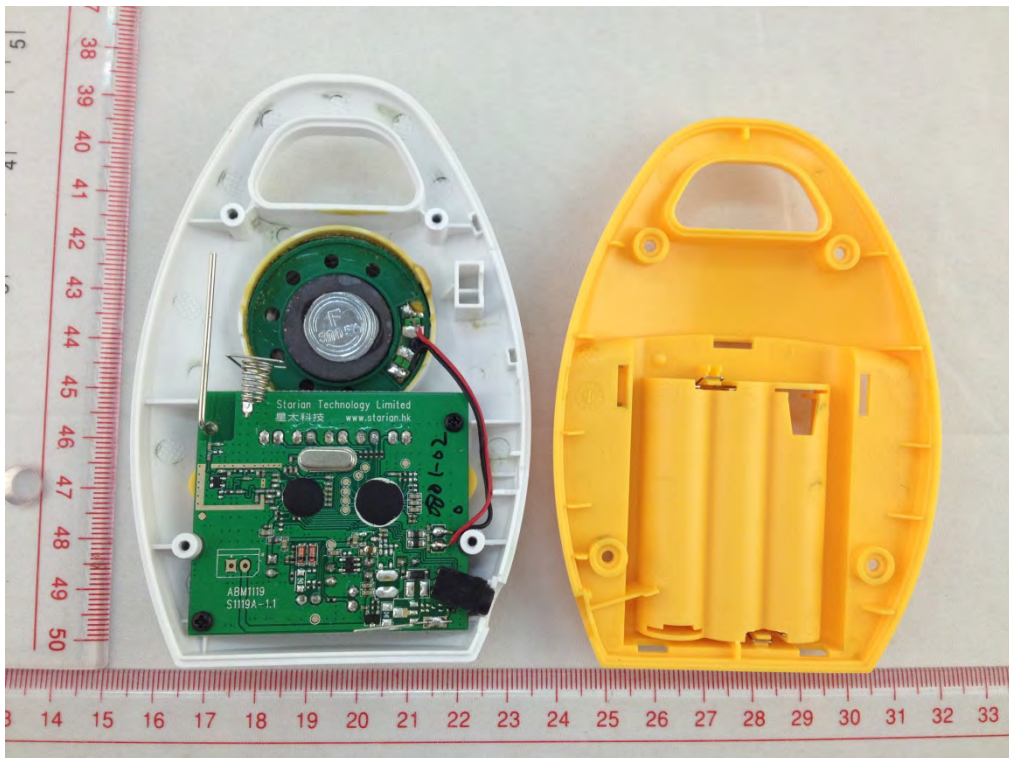
RX UNCOVER VIEW (2)
