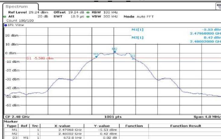
BLE_1M_Ant1_2480
