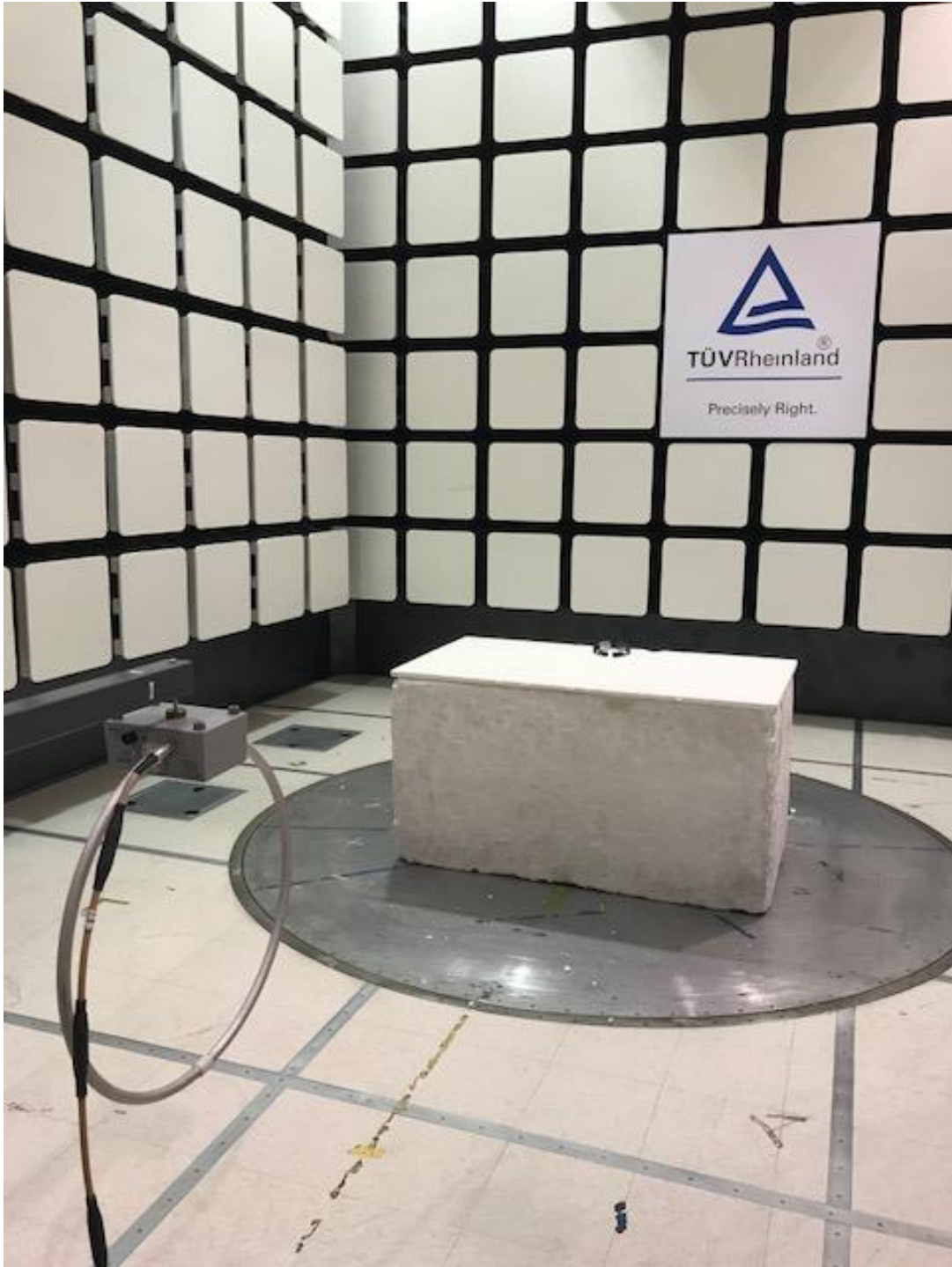
Radiated emissions 9k to 30 MHz front vertical
