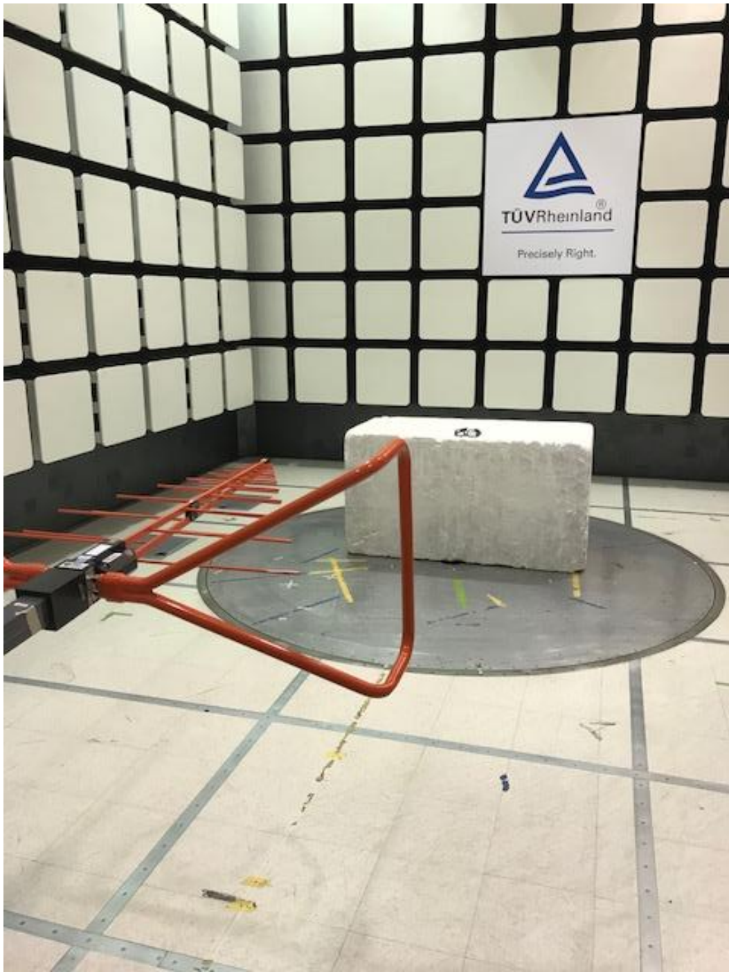
Radiated Emissions 30-1000 MHz. front
