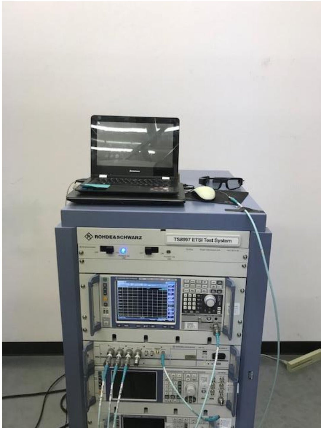
Conducted Test Setup
