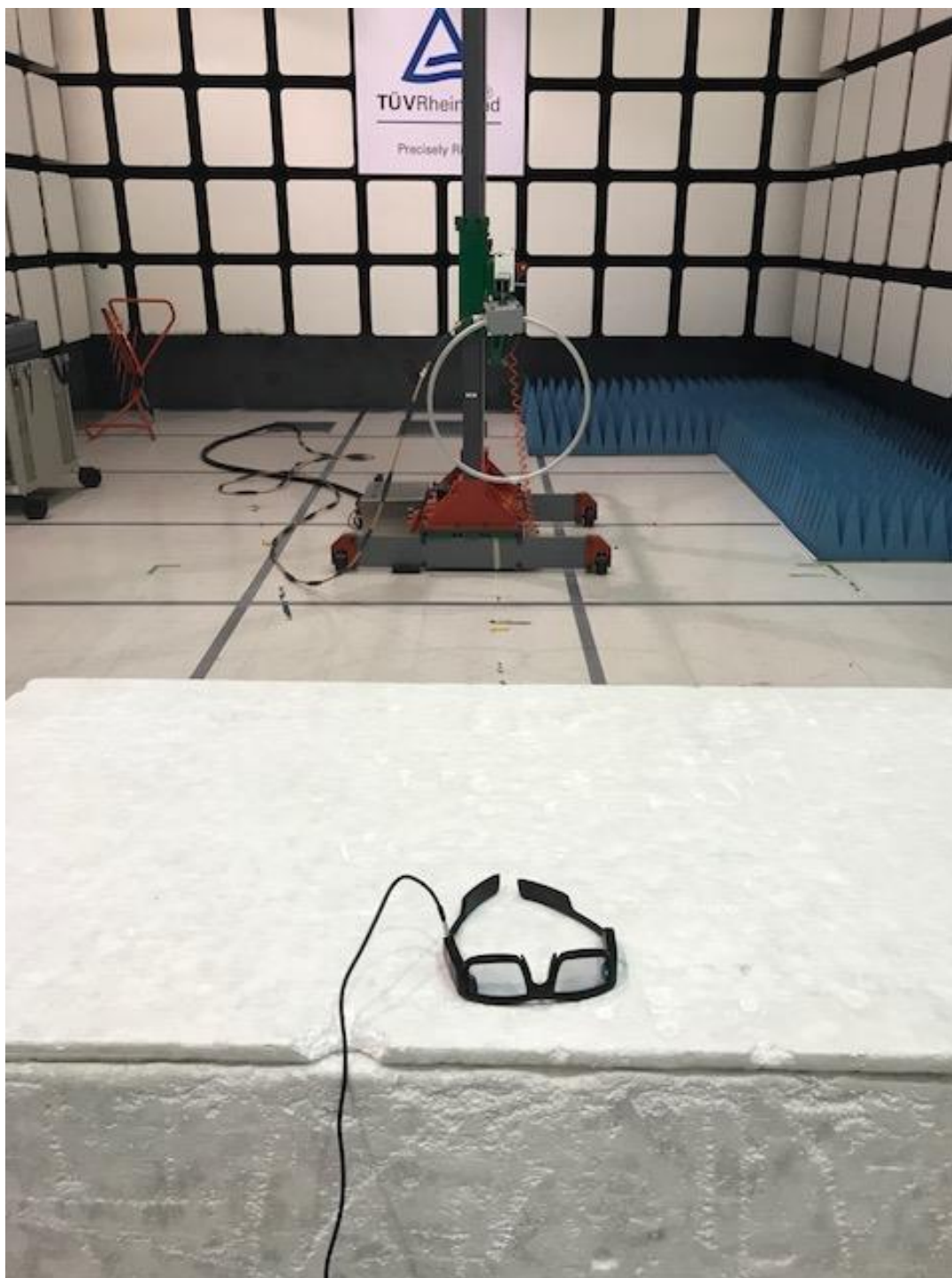
Radiated emissions 9k to 30 MHz rear horizontal
