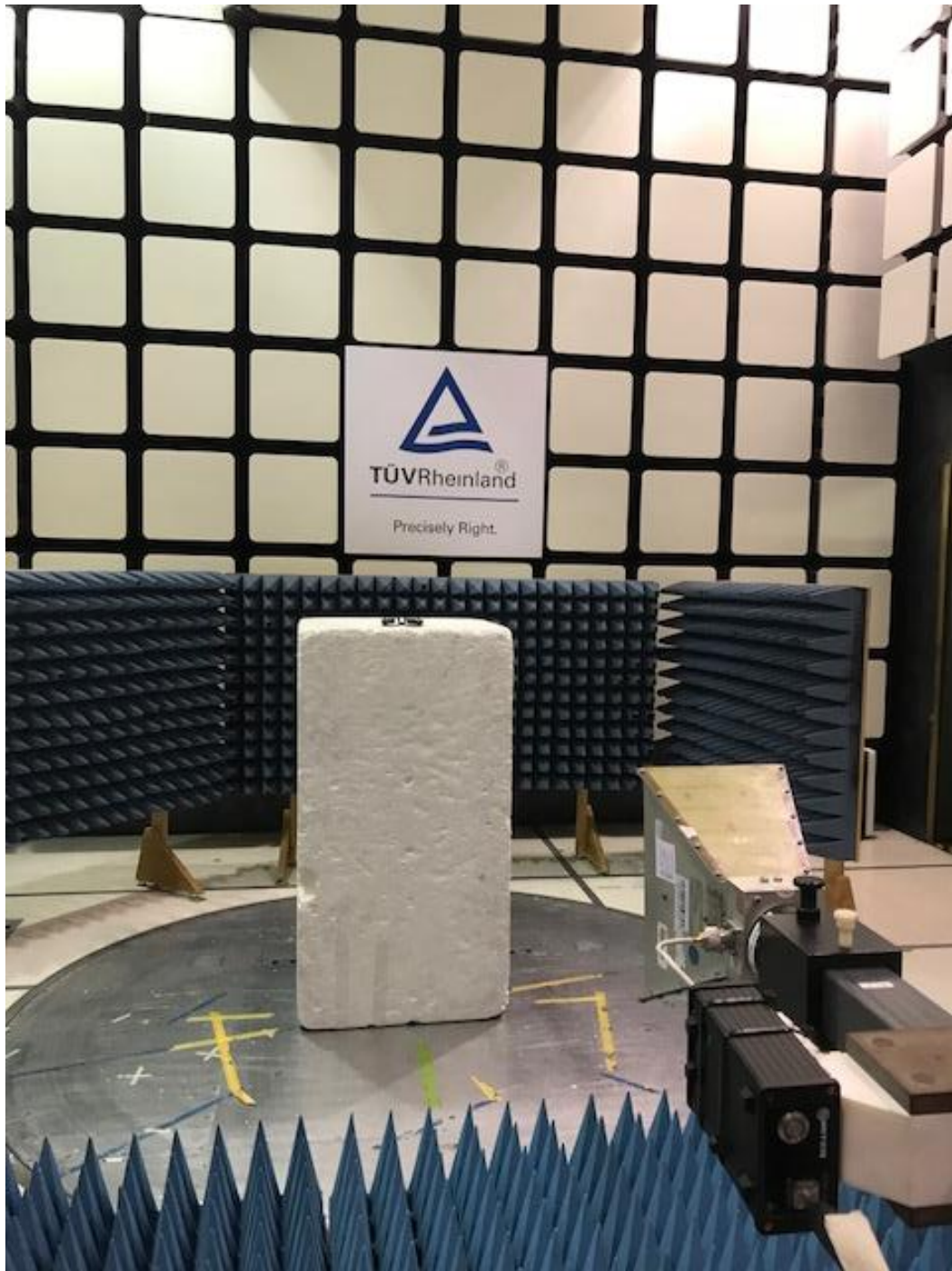
Radiated Emissions 1-18 GHz front
