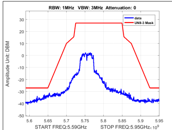
Plot 131. Undesirable Emissions, MIMO, Emissions Mask, Bandwidth 40M, Ch. 5755, ac mode
