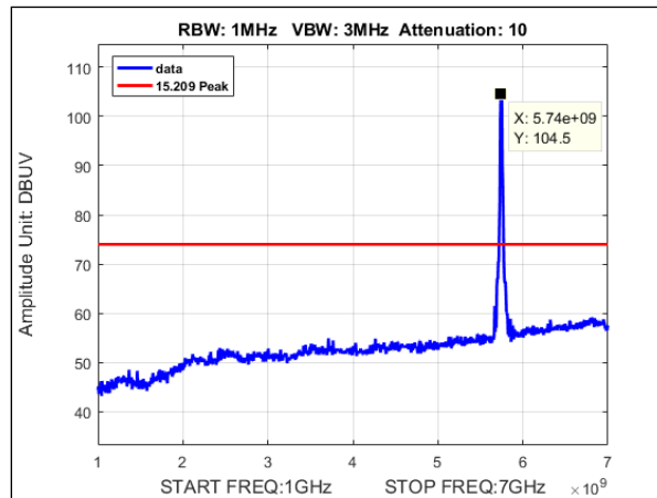
Plot 154. Undesirable Emissions, Peak Radiated Spurious Emissions, MIMO, Bandwidth 20M, Ch. 5745, a mode, 1-7GHz
