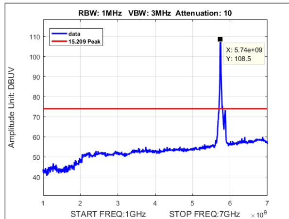
Plot 157. Undesirable Emissions, Peak Radiated Spurious Emissions, MIMO, Bandwidth 20M, Ch. 5745, ac mode, 1-7GHz
