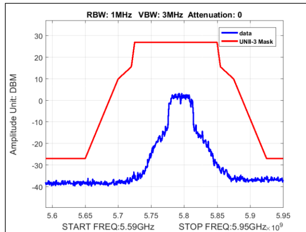
Plot 137. Undesirable Emissions, MIMO, Emissions Mask, Bandwidth 40M, Ch. 5795, n mode
