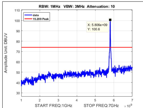
Plot 166. Undesirable Emissions, Peak Radiated Spurious Emissions, MIMO, Bandwidth 20M, Ch. 5805, n mode, 1-7GHz
