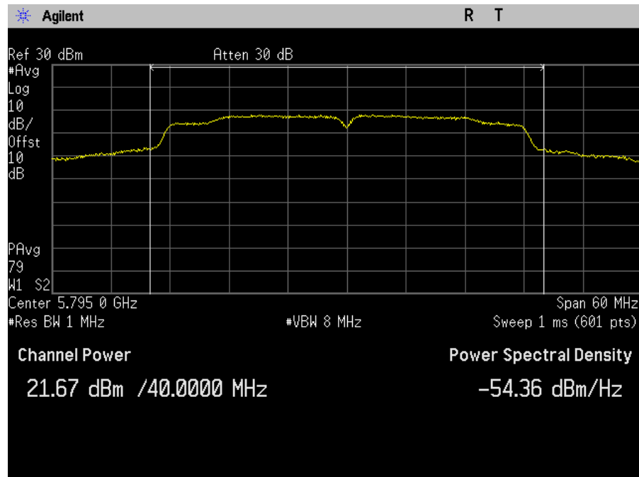
Plot 68. Maximum Conducted Output Power, MIMO, Bandwidth 40M, Ch. 5795M, n mode, port b
