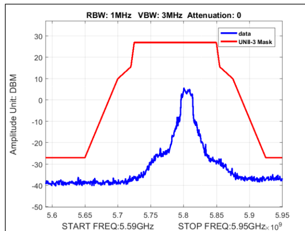
Plot 138. Undesirable Emissions, MIMO, Emissions Mask, Bandwidth 20M, Ch. 5805, n mode
