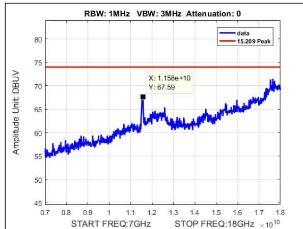
Plot 163. Undesirable Emissions, Peak Radiated Spurious Emissions, MIMO, Bandwidth 80M, Ch. 5775, ac mode, 7-18GHz
