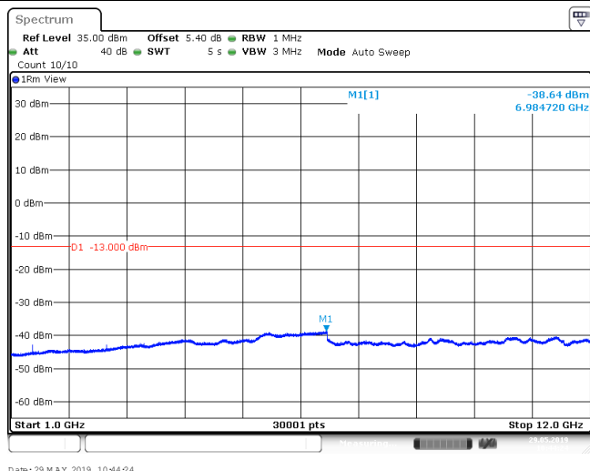
Band12_10MHz_QPSK_23130_1RB#0
