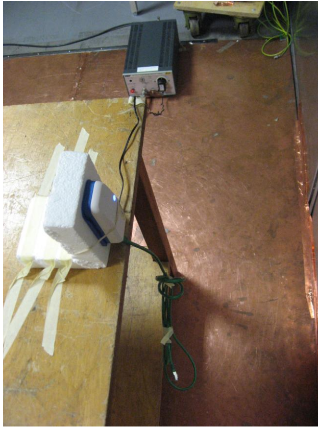
Set up for conducted disturbances
