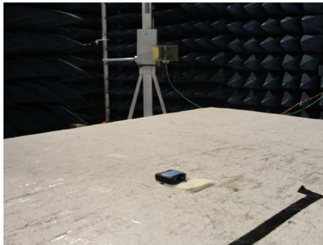
Transmitter Radiated Spurious Emissions Test Setup
