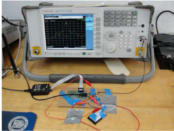
Conducted RF Test Setup
