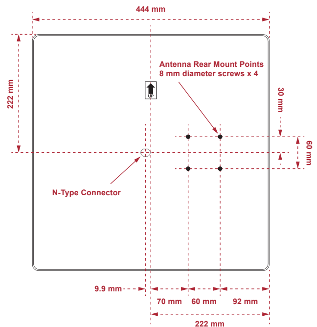
Mounting Diagram
