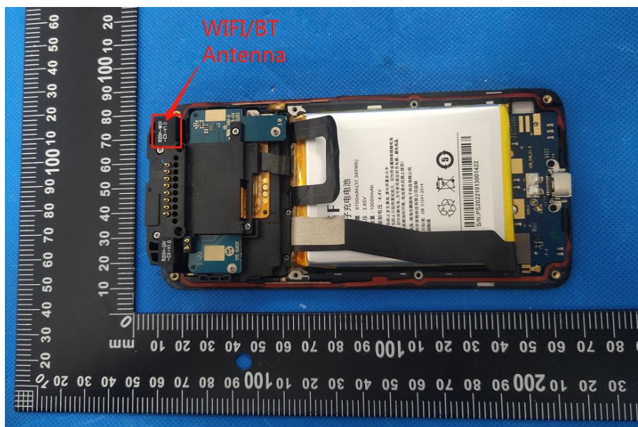
Antenna View (WIFI)
