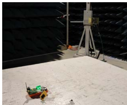
Spurious Emissions Test Setup
