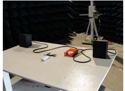
Xmtr & Rx Emissions Setup, Close-up with Different Antenna
