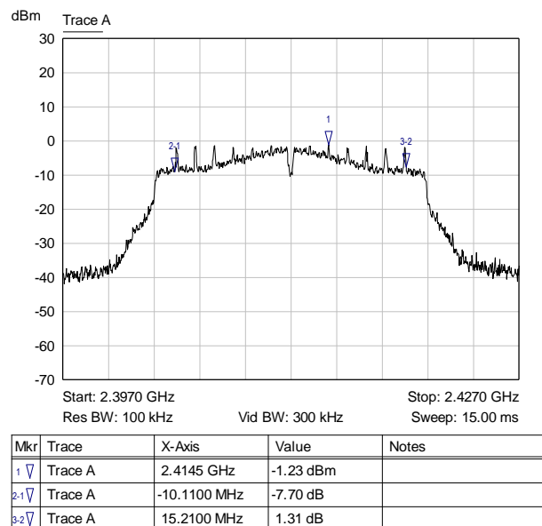
Graph 27: Lowest Channel Bandwidth
