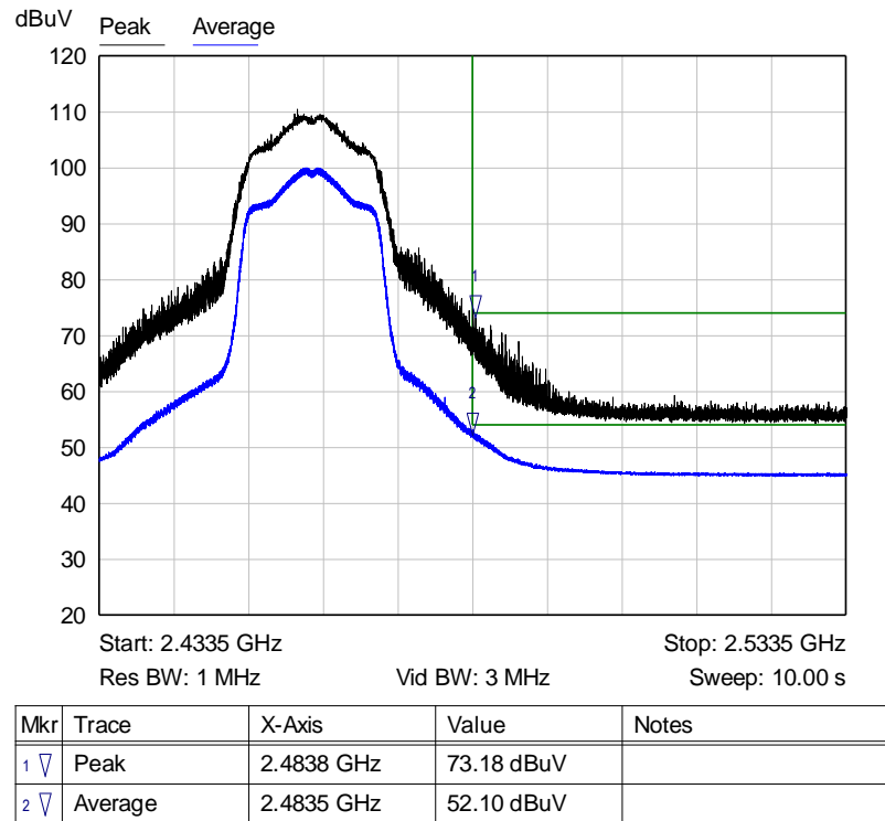
Graph 36: Radiated Upper Band Edge Plot
