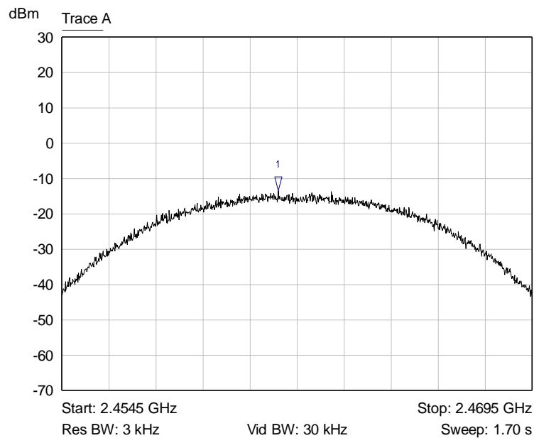
Graph 12: Middle Channel 3 kHz PSD Plot
