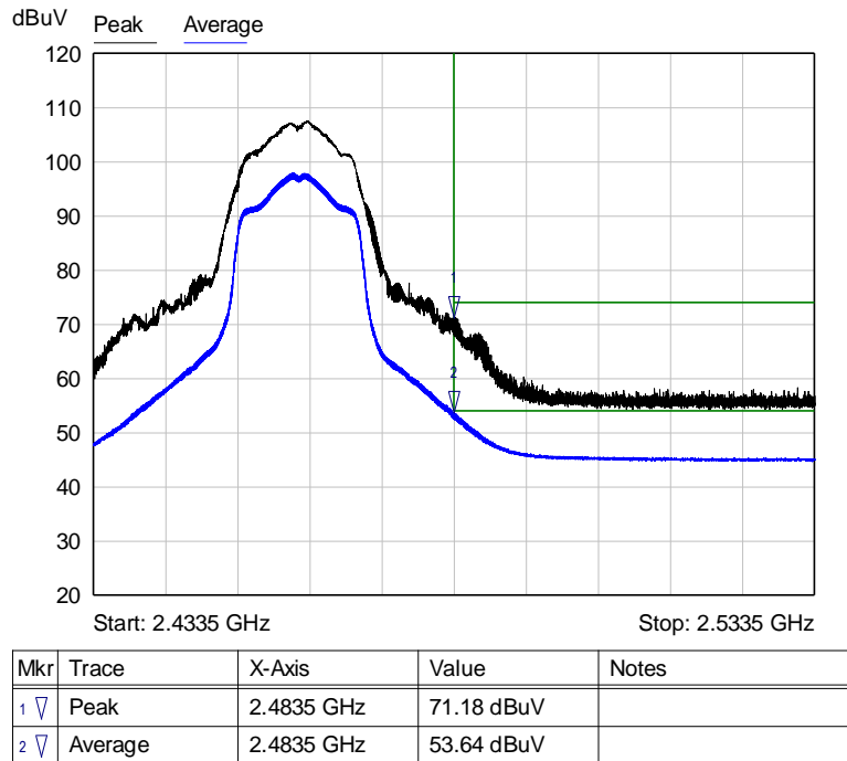
Graph 23: Radiated Upper Band Edge Plot
