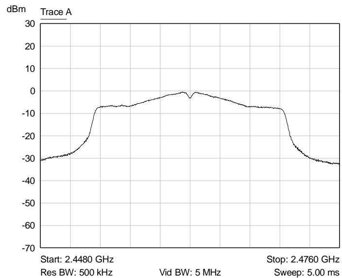
Graph 31: Middle Channel Output Power
