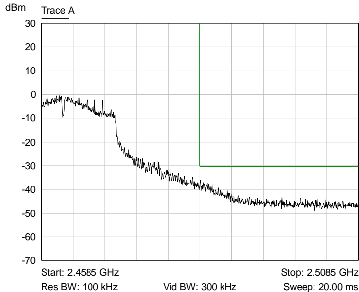
Graph 21: Upper Band Edge Plot
