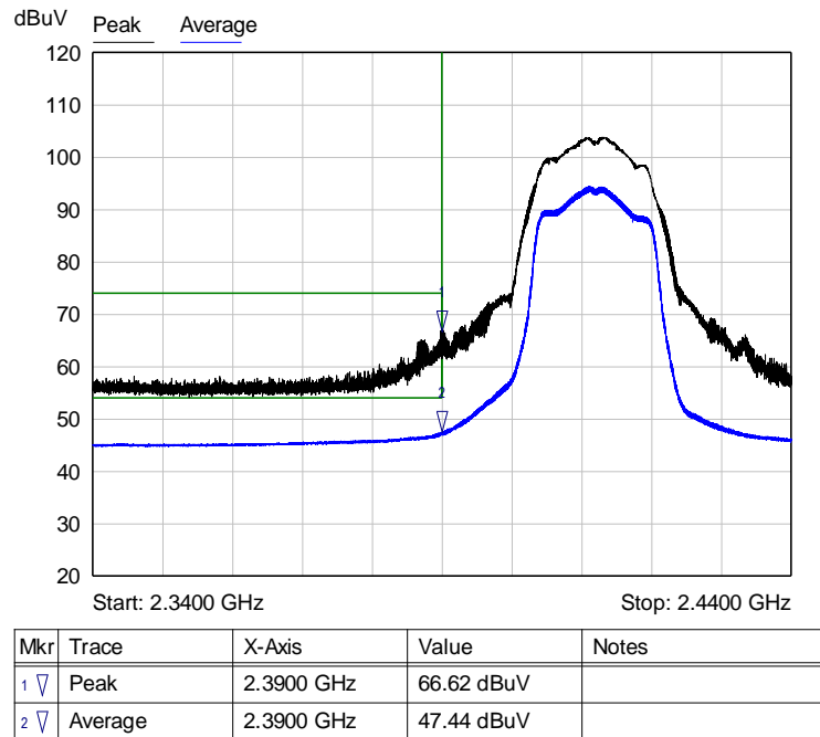
Graph 22: Radiated Lower Band Edge Plot
