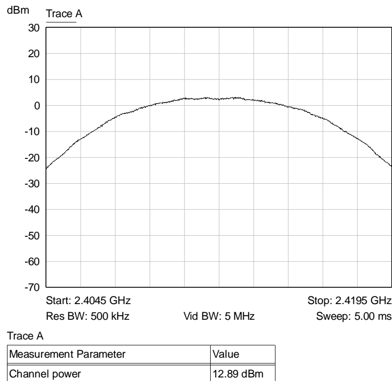
Graph 4: Lowest Channel Output Power Plot
