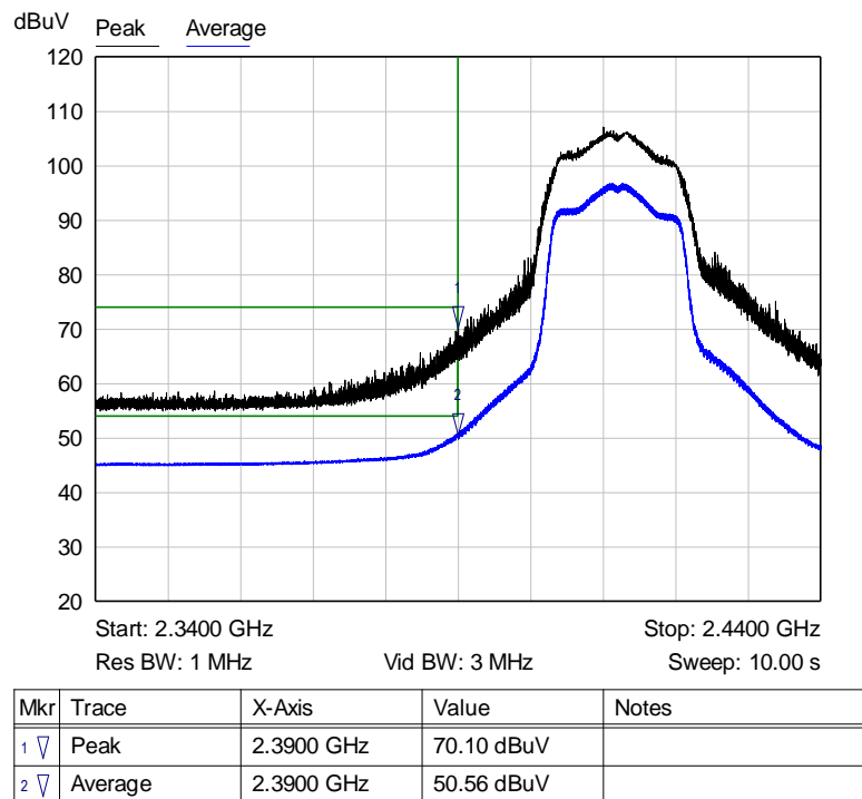
Graph 35: Radiated Lower Band Edge Plot
