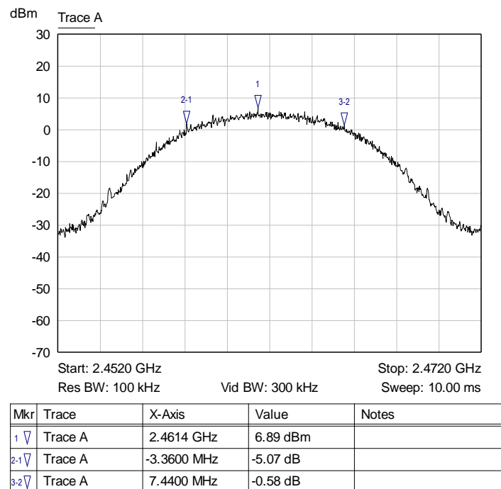
Graph 3: Highest Channel Bandwidth
