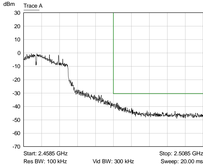
Graph 34: Upper Band Edge Plot
