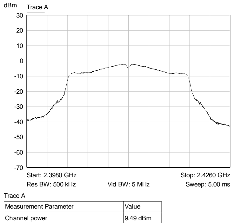
Graph 17: Lowest Channel Output Power Plot
