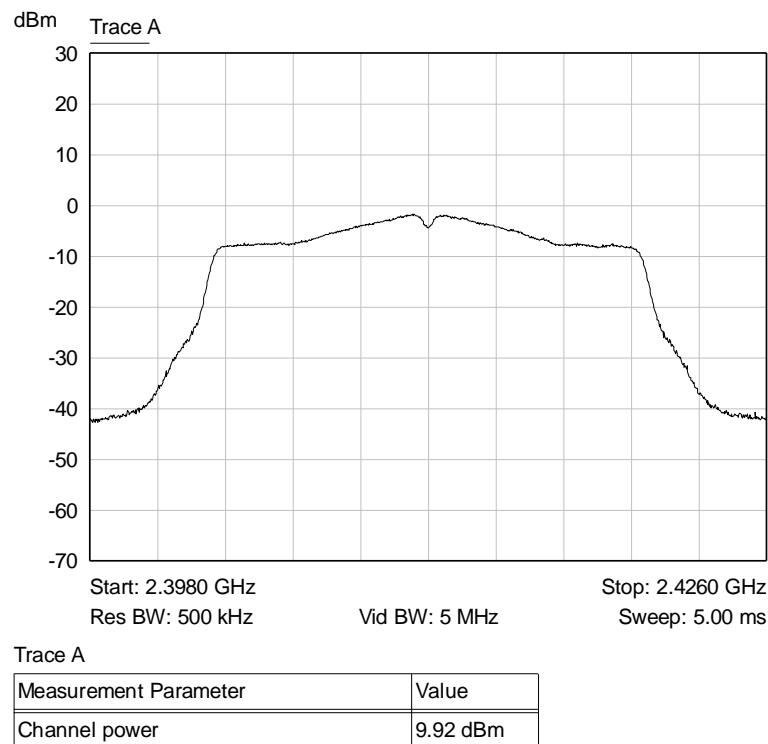
Graph 30: Lowest Channel Output Power Plot
