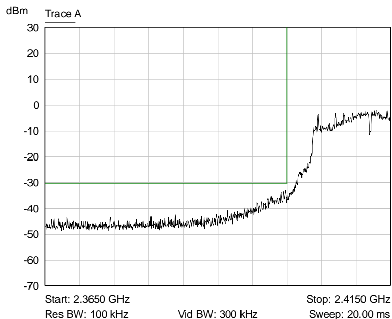
Graph 20: Lower Band Edge Plot
