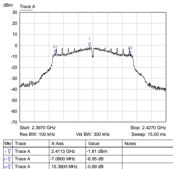
Graph 14: Lowest Channel Bandwidth
