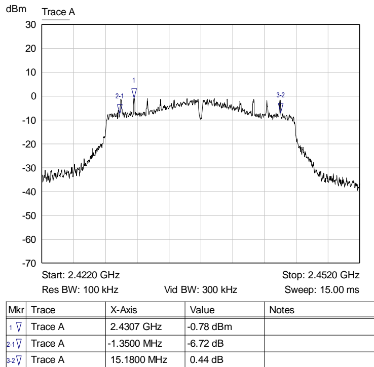
Graph 28: Middle Channel Bandwidth
