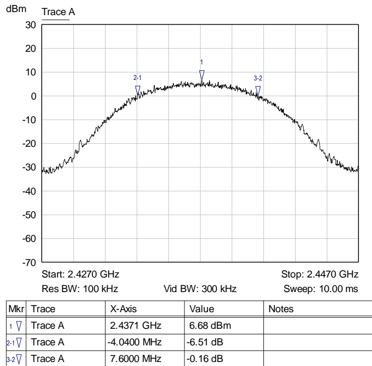
Graph 2: Middle Channel Bandwidth
