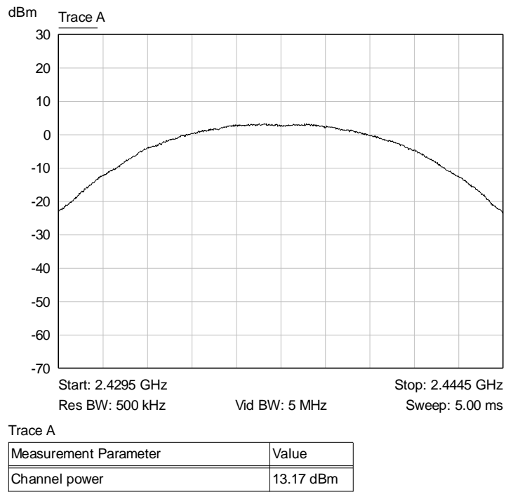
Graph 5: Middle Channel Output Power
