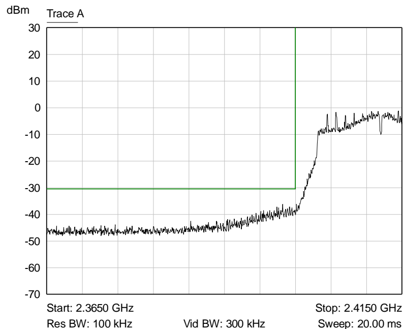
Graph 33: Lower Band Edge Plot
