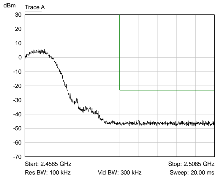
Graph 8: Upper Band Edge Plot
