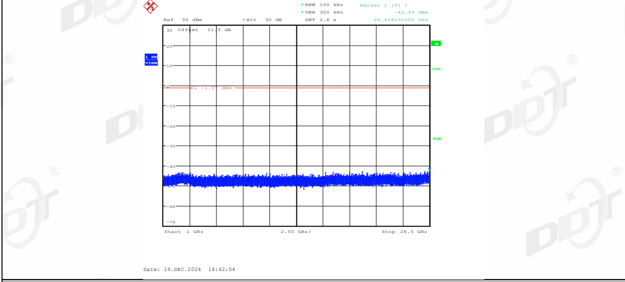
GFSK_Ant1_919.8_0~Reference
