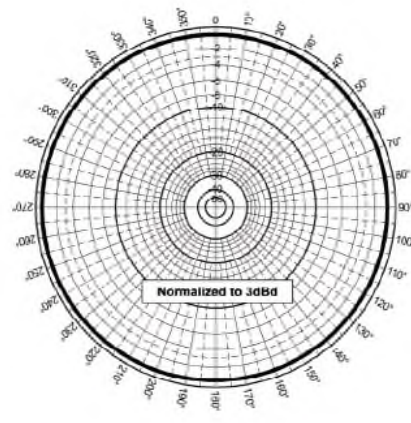
Azimuthal Pattern (Y, Z, or E-plane)
