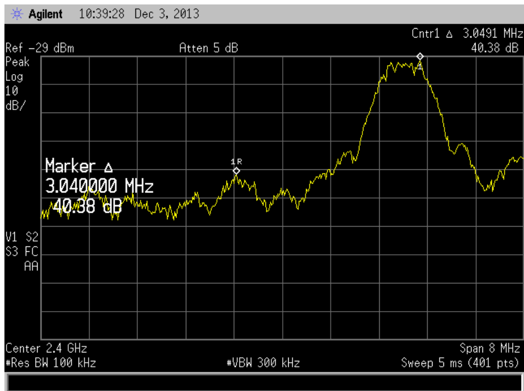
Figure 8. Radiated Band Edge – Low Channel Delta
