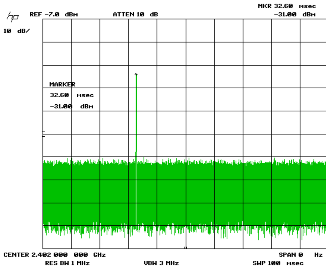
Figure 3. Transmitter Pulse Width (100ms)
