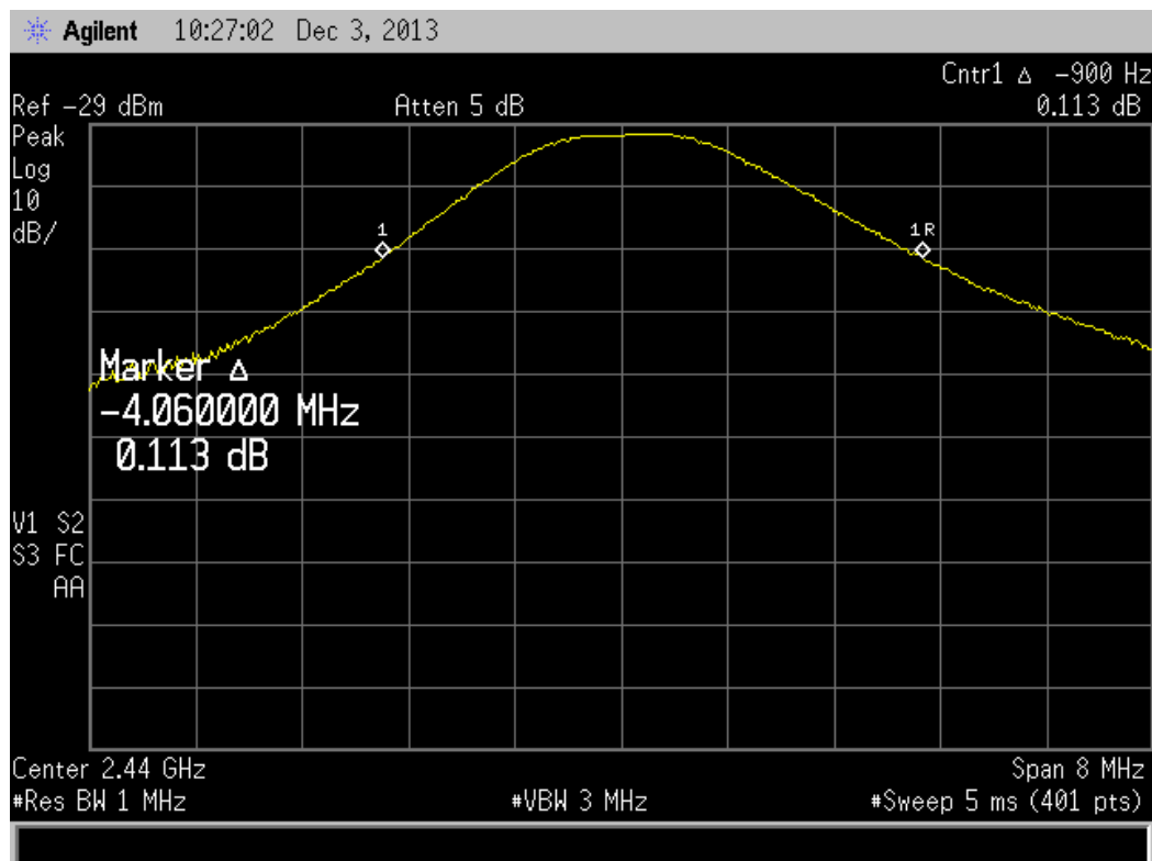
Figure 5. Mid Ch Bandwidth
