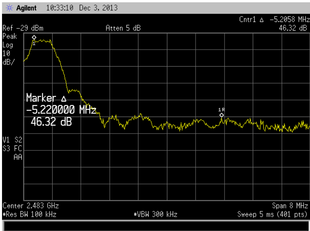
Figure 7. Radiated Band Edge – High Channel Delta
