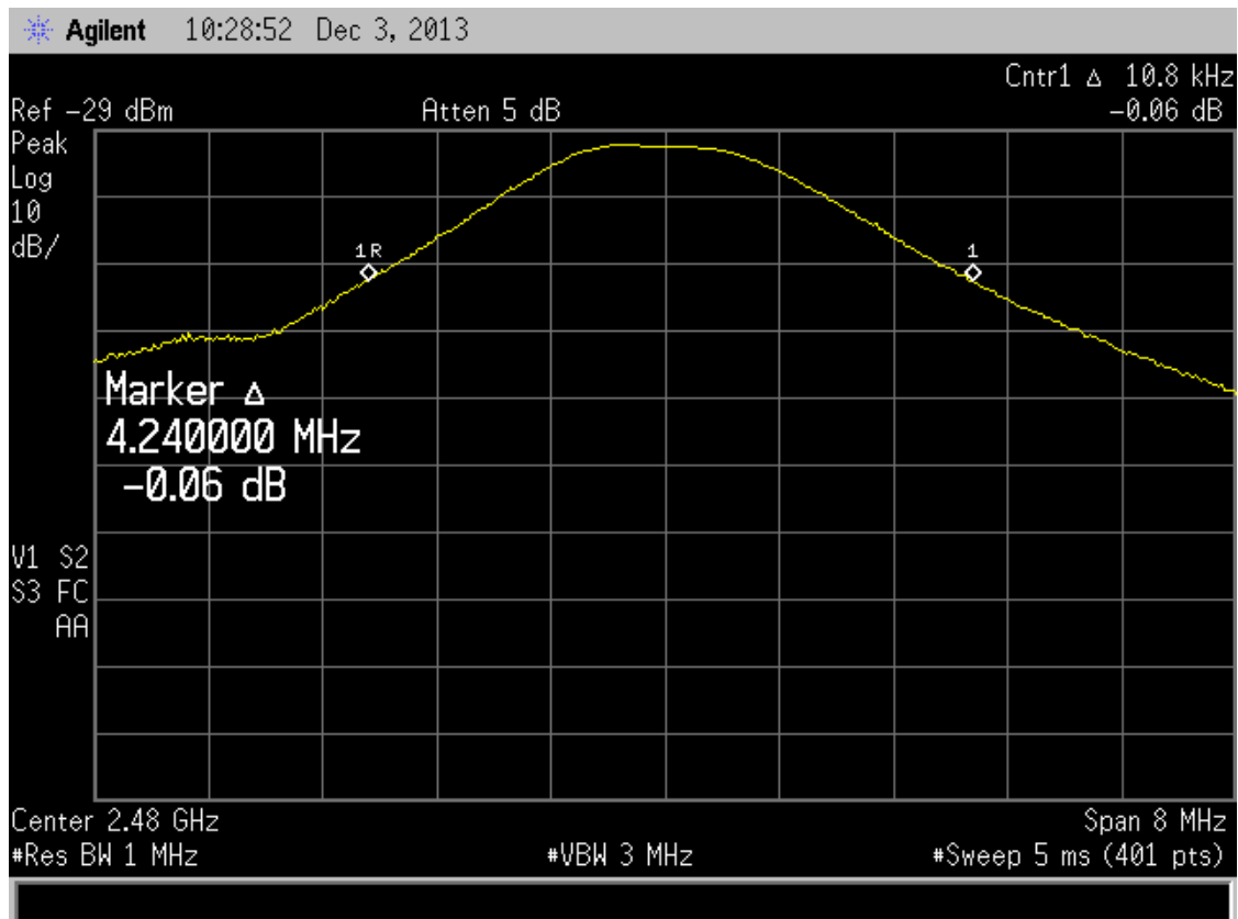
Figure 6. High Ch Bandwidth
