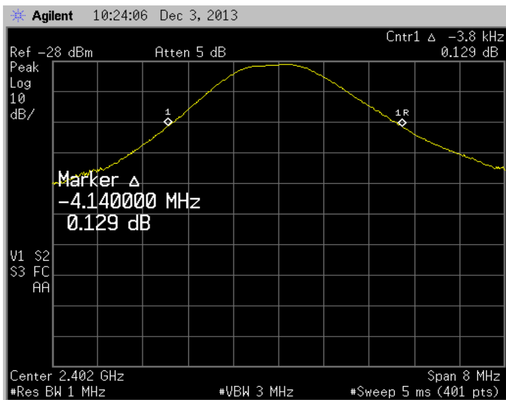
Figure 4. Low Ch Bandwidth
