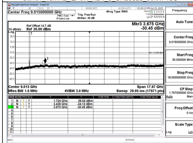
Band4 20MHz QPSK RB1 0 CH20175 below 18G
