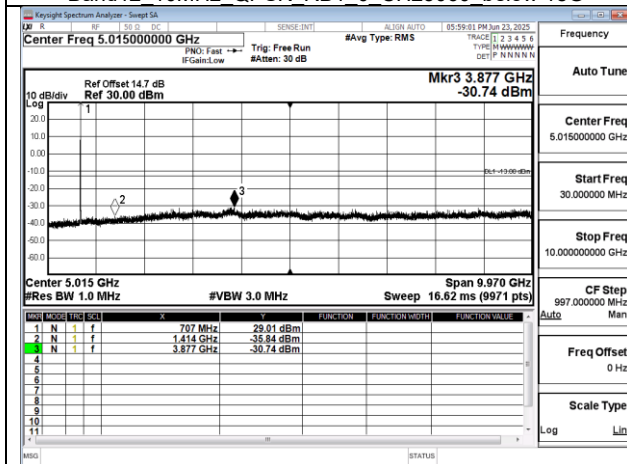
Band12_10MHz_QPSK_RB1_0_CH23130 below 18G
