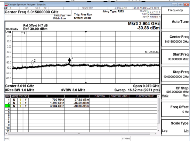
Band12 5MHz QPSK RB1 0 CH23035 below 18G
