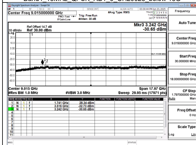
Band4 15MHz QPSK RB1 0 CH20325 below 18G
