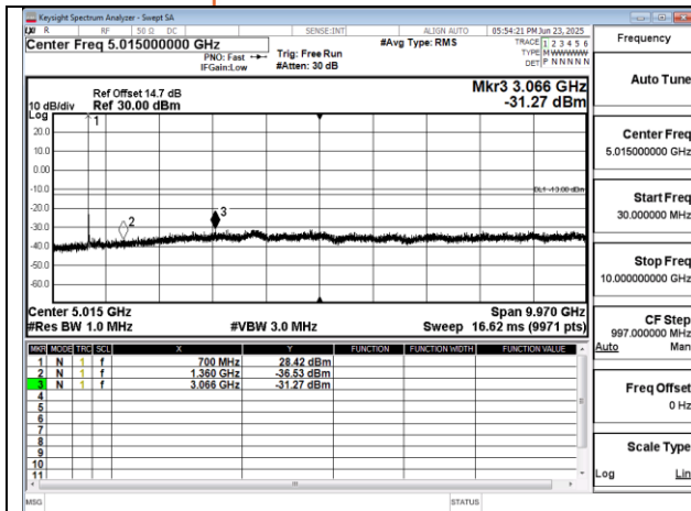
Band12_10MHz_QPSK_RB1_0_CH23060 below 18G
