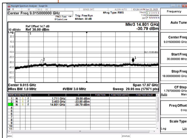
Band4 15MHz QPSK RB1 0 CH20025 below 18G
