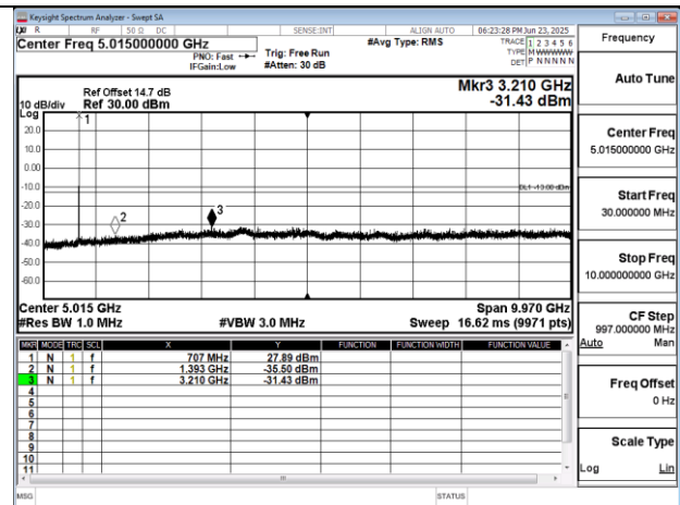
Band12 1.4MHz QPSK RB1 0 CH23095 below 18G
