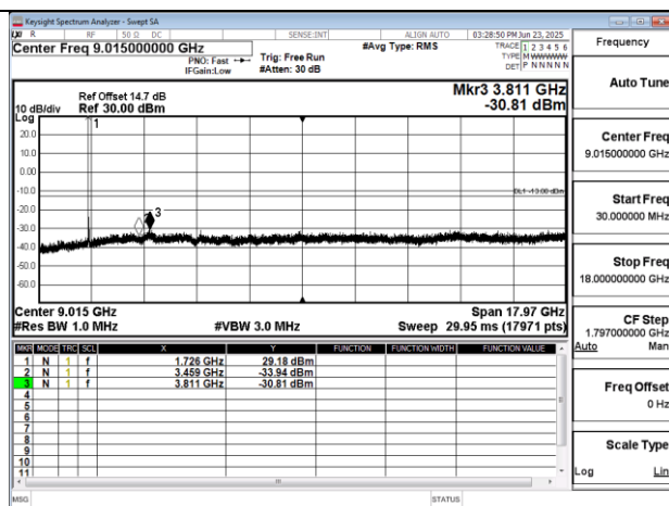
Band4 15MHz QPSK RB1 0 CH20175 below 18G
