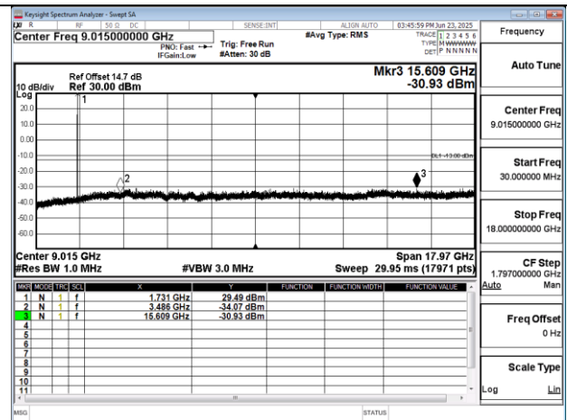
Band4 5MHz QPSK RB1 0 CH20175 below 18G
