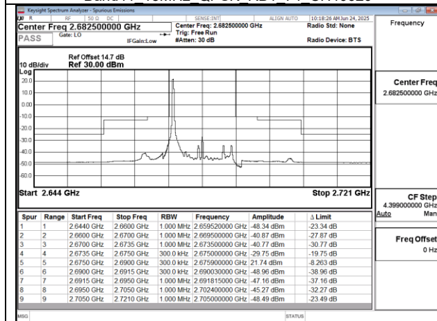
Band41 15MHz QPSK RB1 0 CH41515
