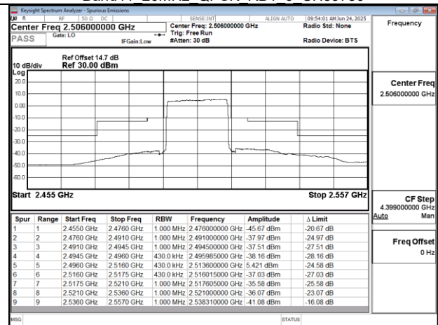
Band41 20MHz QPSK RB100 0 CH39750
