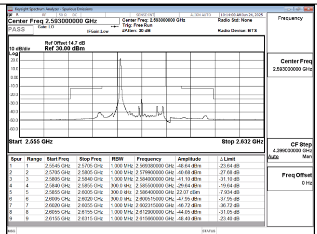
Band41 15MHz QPSK RB1 0 CH40620
