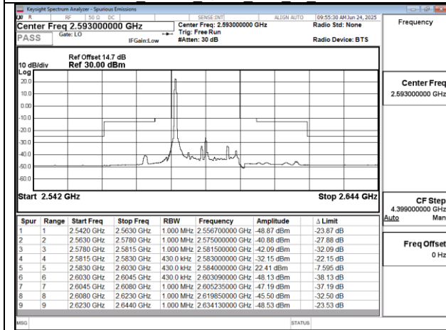
Band41 20MHz QPSK RB1 0 CH40620
