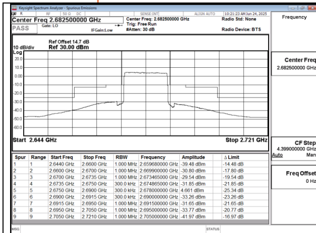
Band41 15MHz QPSK RB75 0 CH41515
