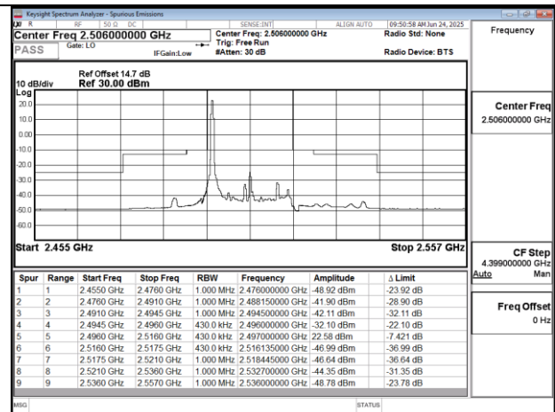
Band41 20MHz QPSK RB1 0 CH39750
