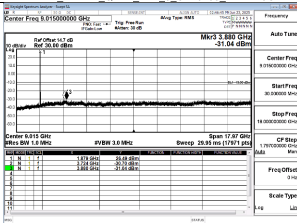
Band2 3MHz QPSK RB1 0 CH18900 below 18G
