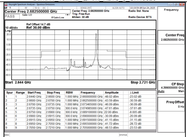
Band41 15MHz QPSK RB1 74 CH41515
