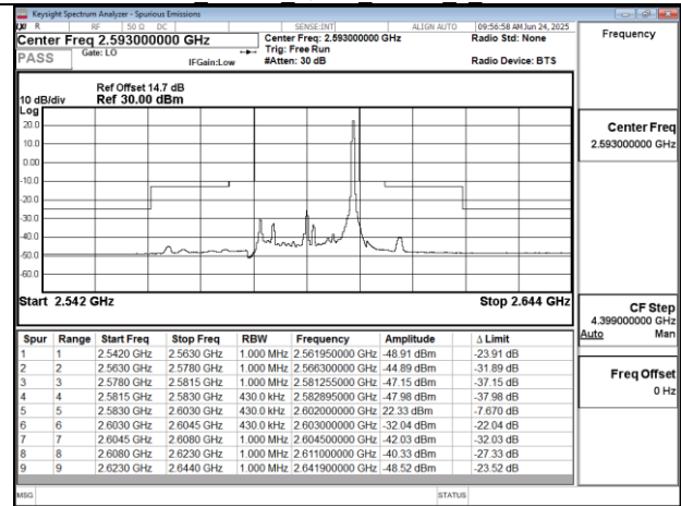
Band41 20MHz QPSK RB1 99 CH40620
