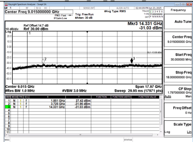
Band2 3MHz QPSK RB1 0 CH18615 below 18G
