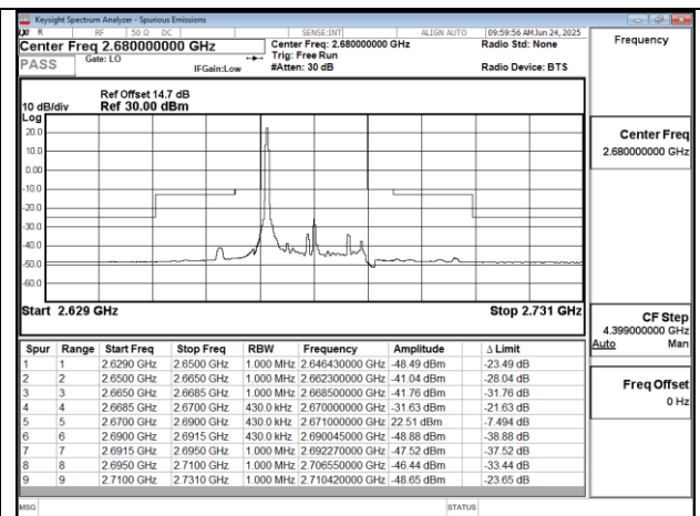
Band41 20MHz QPSK RB1 0 CH41490
