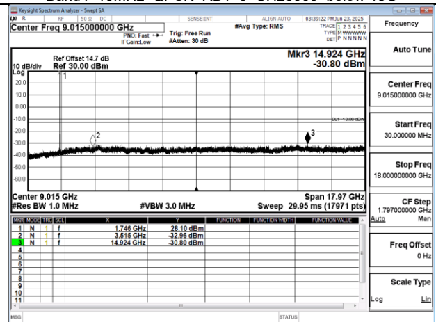
Band4 10MHz QPSK RB1 0 CH20350 below 18G
