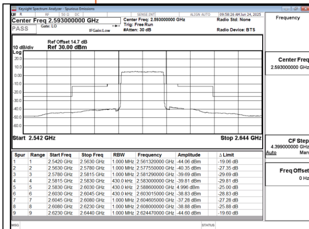
Band41 20MHz QPSK RB100 0 CH40620
