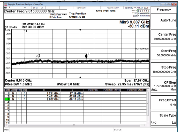
Band4 10MHz QPSK RB1 0 CH20000 below 18G
