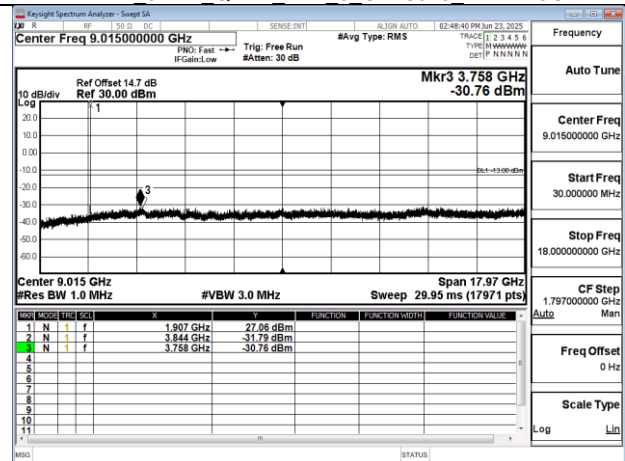
Band2 3MHz QPSK RB1 0 CH19185 below 18G
