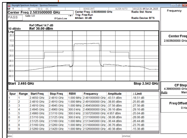
Band41 15MHz QPSK RB75 0 CH39725
