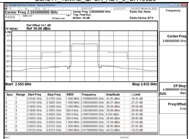
Band41 15MHz QPSK RB75 0 CH40620
