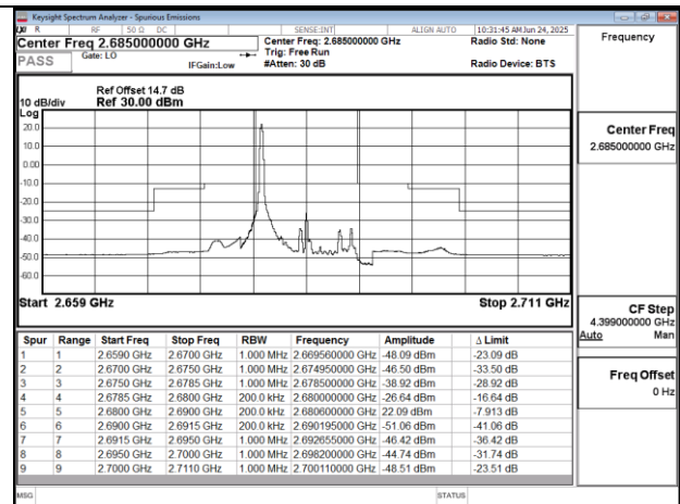
Band41 10MHz QPSK RB1 0 CH41540
