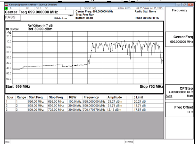
Band12 3MHz QPSK RB15 0 CH23025
