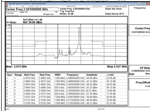
Band41 10MHz QPSK RB1 49 CH39700
