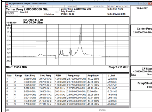
Band41 10MHz QPSK RB1 49 CH41540
