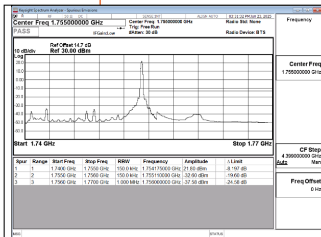
Band4 15MHz QPSK RB1 74 CH20325
