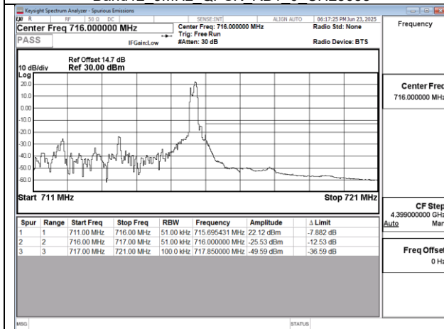
Band12 5MHz QPSK RB1 24 CH23155
