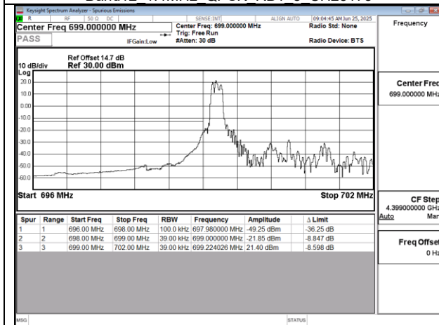
Band12 3MHz QPSK RB1 0 CH23025
