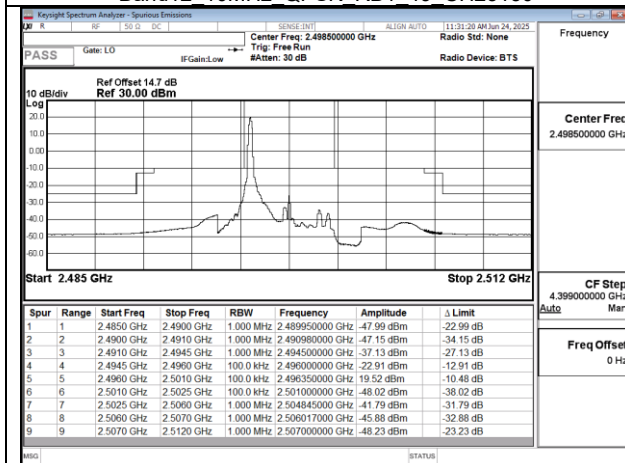
Band41 5MHz QPSK RB1 0 CH39675
