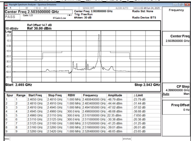
Band41 15MHz QPSK RB1 74 CH39725
