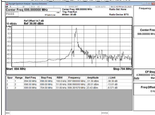
Band12 5MHz QPSK RB1 0 CH23035
