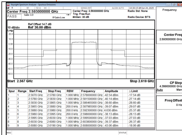
Band41 10MHz QPSK RB50 0 CH40620
