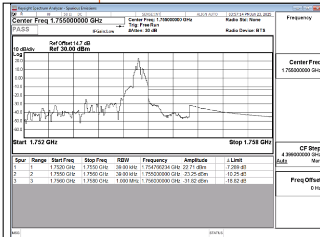
Band4 3MHz QPSK RB1 14 CH20385
