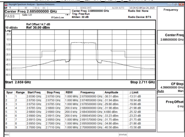
Band41 10MHz QPSK RB50 0 CH41540
