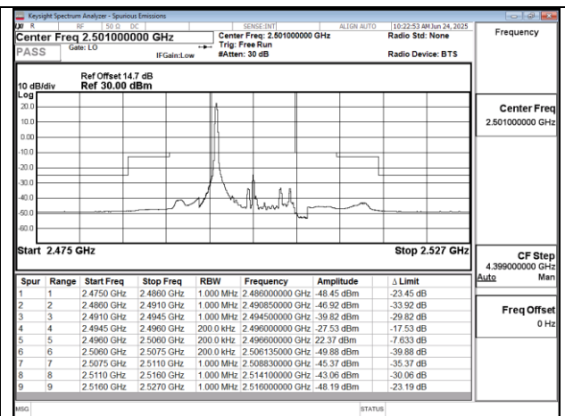
Band41 10MHz QPSK RB1 0 CH39700
