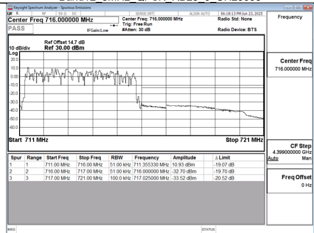
Band12 5MHz QPSK RB25 0 CH23155
