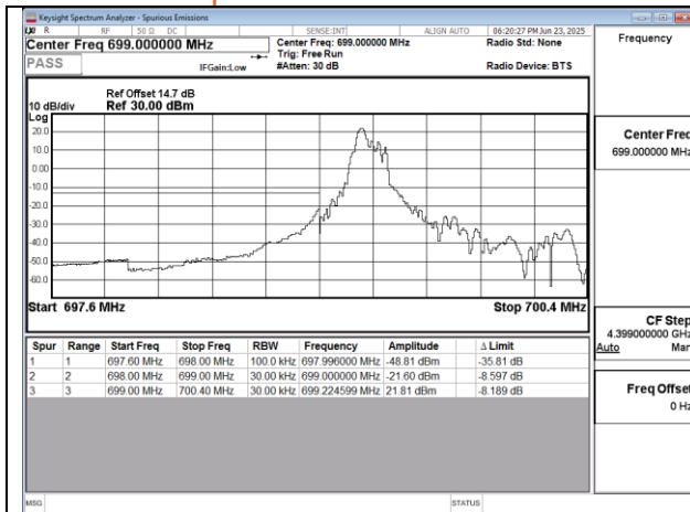
Band12 1.4MHz QPSK RB1 0 CH23017
