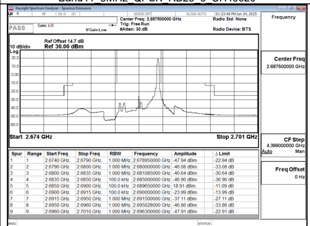
Band41 5MHz QPSK RB1 24 CH41565
