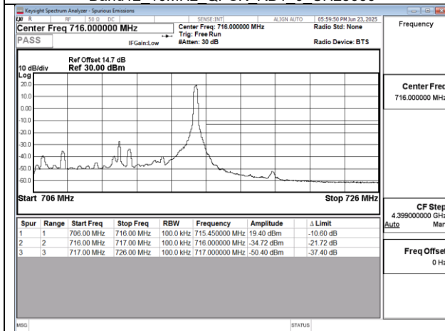
Band12 10MHz QPSK RB1 49 CH23130
