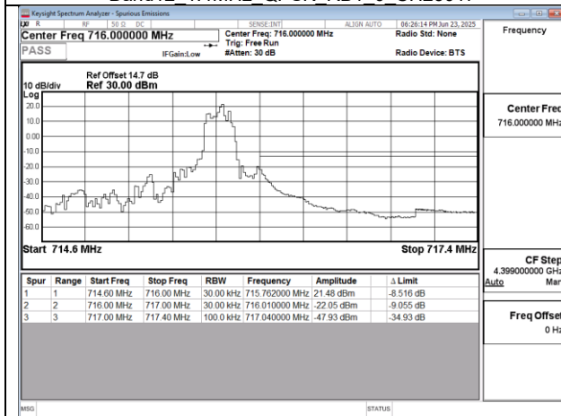
Band12 1.4MHz QPSK RB1 5 CH23173
