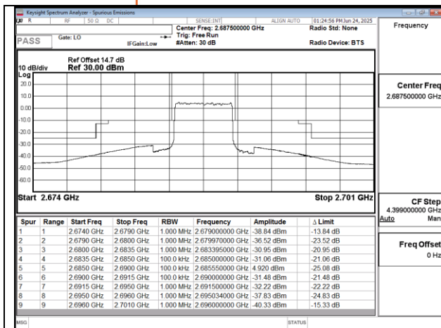
Band41 5MHz QPSK RB25 0 CH41565
