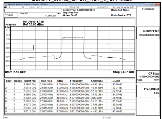
Band41 5MHz QPSK RB25 0 CH40620
