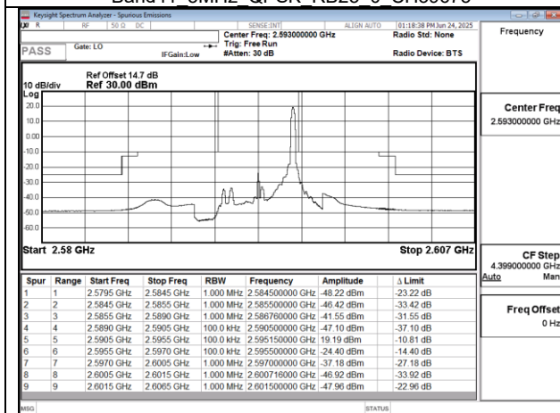
Band41 5MHz QPSK RB1 24 CH40620
