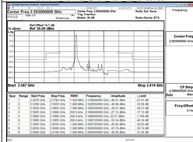
Band41 10MHz QPSK RB1 0 CH40620
