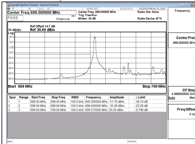
Band12 10MHz QPSK RB1 0 CH23060
