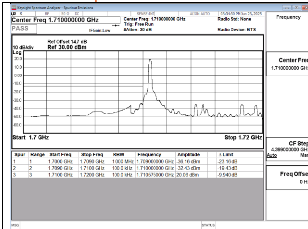
Band4 10MHz QPSK RB1 0 CH20000
