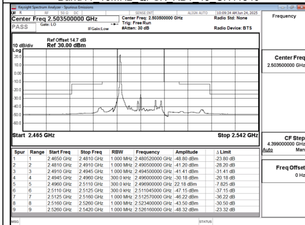
Band41 15MHz QPSK RB1 0 CH39725
