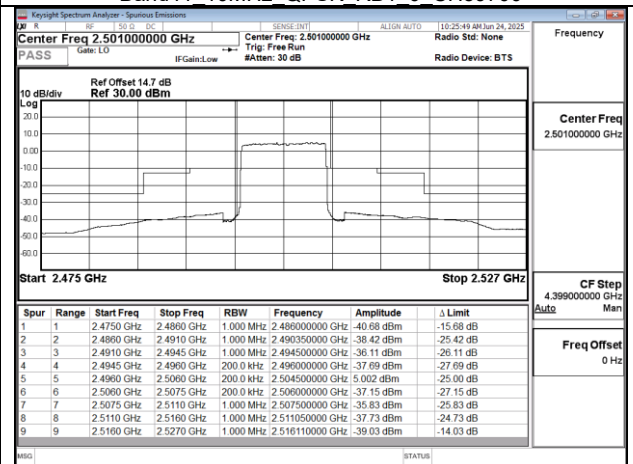
Band41 10MHz QPSK RB50 0 CH39700
