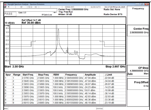
Band41 5MHz QPSK RB1 0 CH40620
