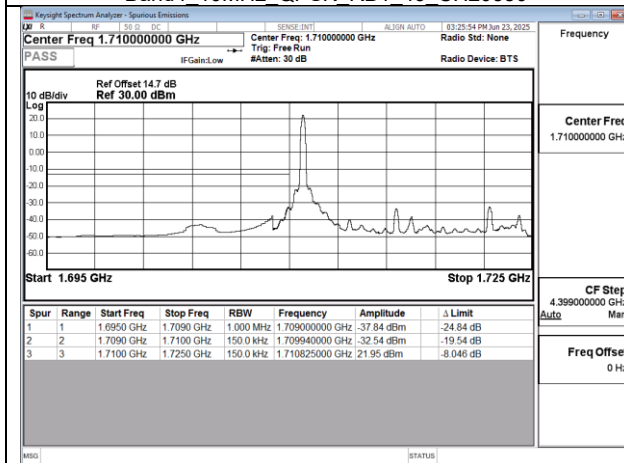
Band4 15MHz QPSK RB1 0 CH20025
