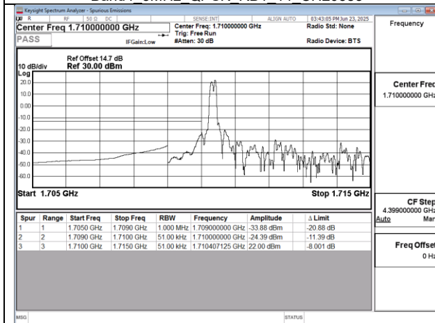
Band4 5MHz QPSK RB1 0 CH19975
