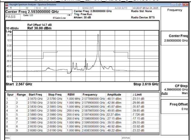
Band41 10MHz QPSK RB1 49 CH40620
