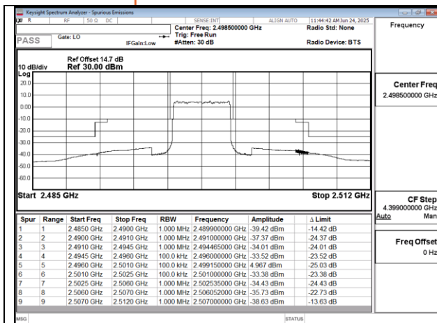
Band41 5MHz QPSK RB25 0 CH39675
