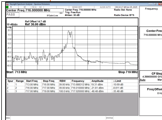
Band12 3MHz QPSK RB1 14 CH23165
