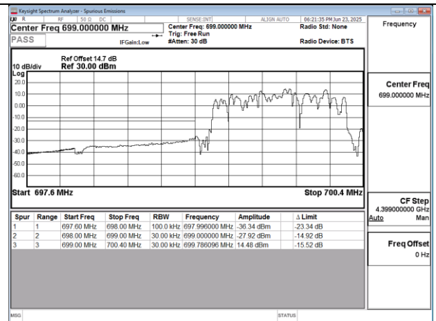
Band12 1.4MHz QPSK RB6 0 CH23017
