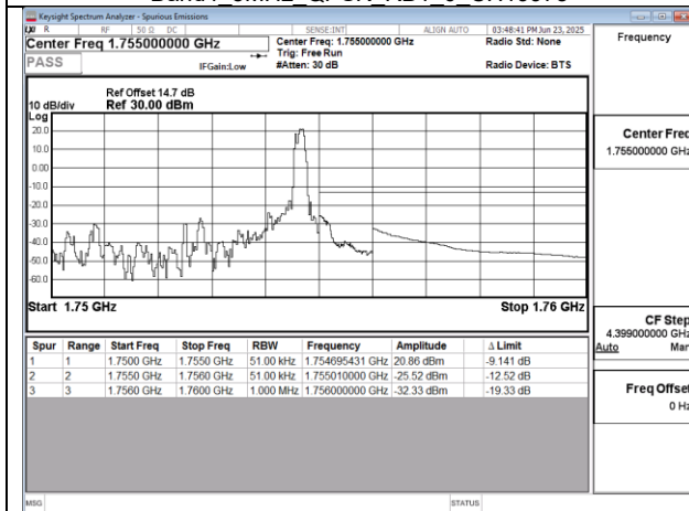
Band4 5MHz QPSK RB1 24 CH20375
