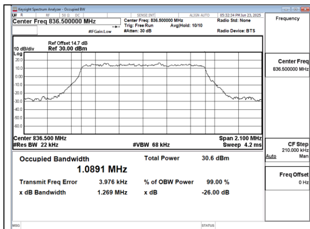
Band5 1.4MHz 16QAM RB6 0 CH20525
