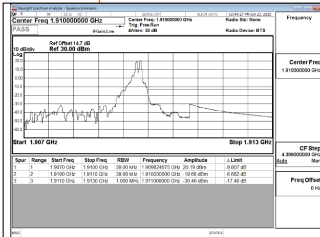
Band2 3MHz QPSK RB1 14 CH19185
