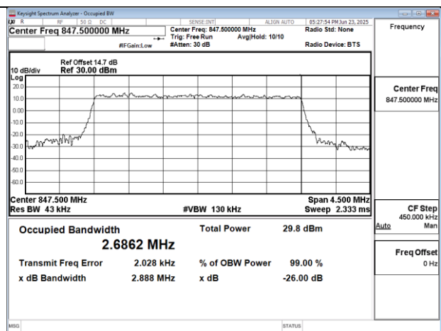
Band5 3MHz 64QAM RB15 0 CH20635
