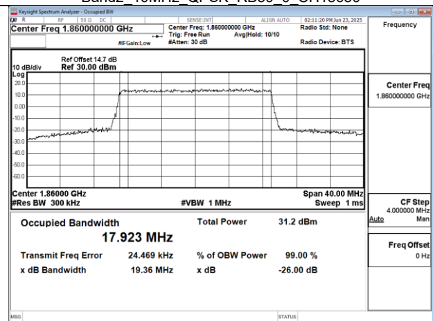
Band2 20MHz 16QAM RB100 0 CH18700
