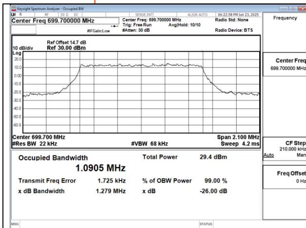
Band12 1.4MHz 64QAM RB6 0 CH23017
