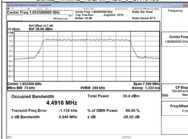
Band2 5MHz 64QAM RB25 0 CH18625
