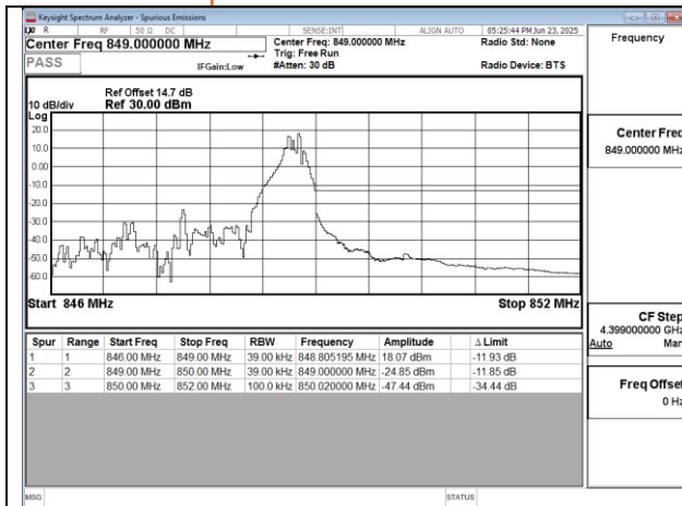
Band5 3MHz QPSK RB1 14 CH20635
