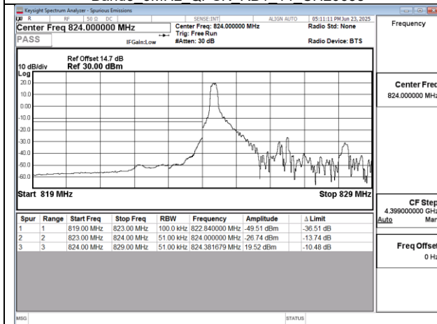
Band5 5MHz QPSK RB1 0 CH20425
