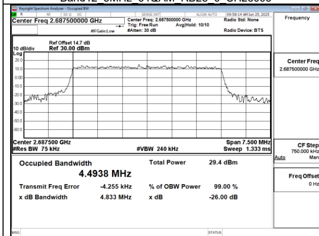
Band41 5MHz 64QAM RB25 0 CH41565
