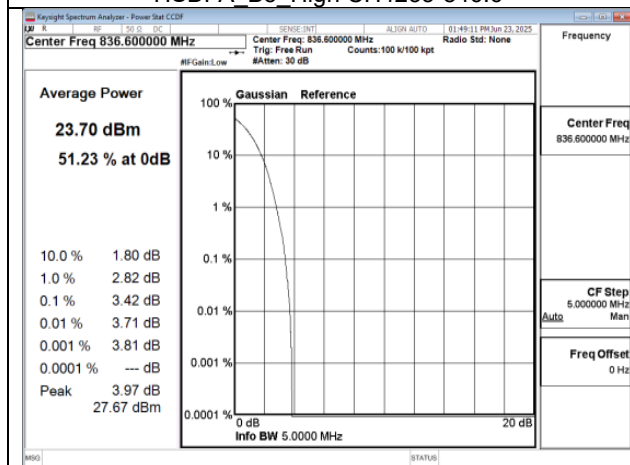
HSUPA_B5_Mid CH4183-836.6
