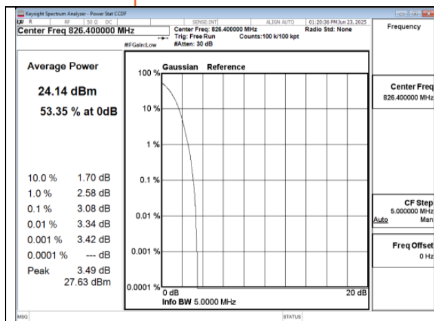
HSDPA_B5_Low CH4132-826.4
