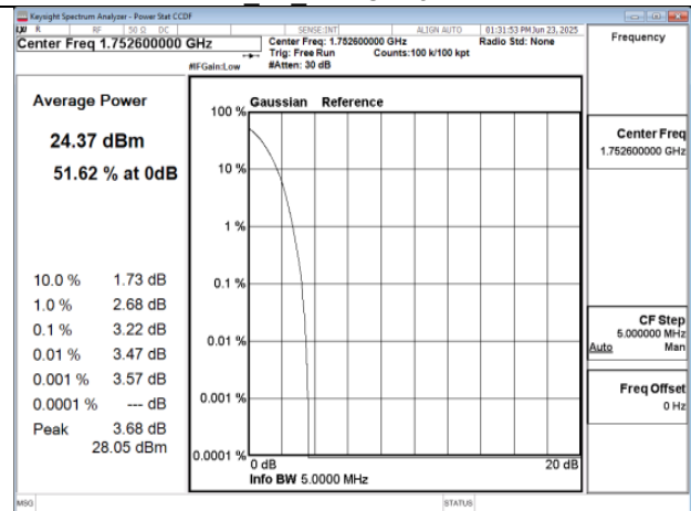
HSDPA B4 High CH1513-1752.6
