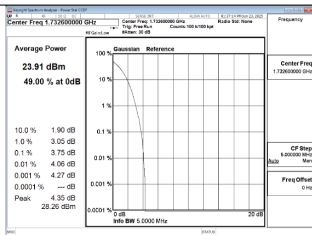
HSPA B4 Mid CH1413-1732.6
