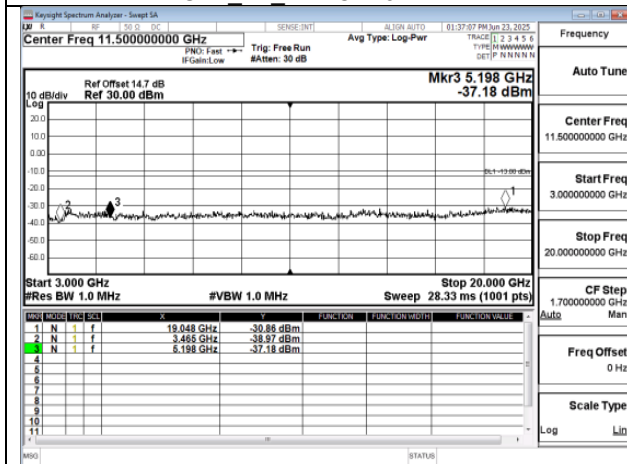
HSPA B4 Mid CH1413-1732.6
