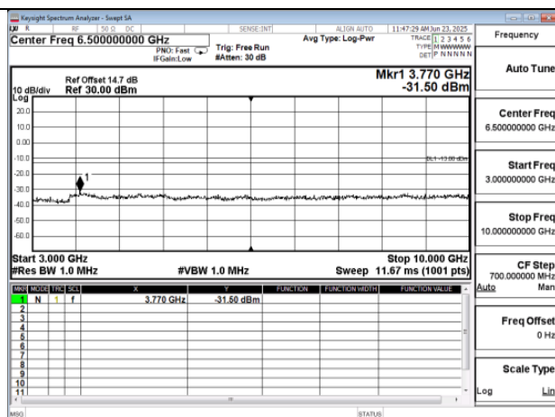
WCDMA_B5_Mid_CH4183-836.6
