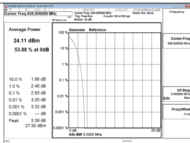
HSDPA_B5_Mid CH4183-836.6
