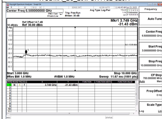
WCDMA_B5_High_CH4233-846.6
