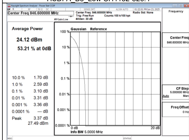
HSDPA_B5_High CH4233-846.6
