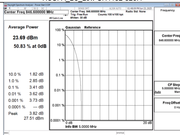
HSUPA_B5_High CH4233-846.6
