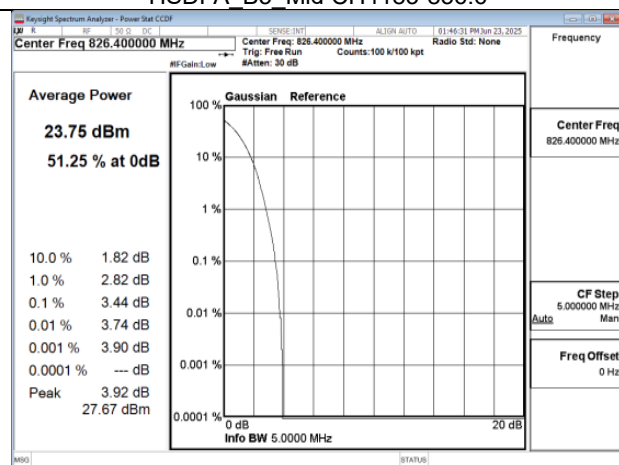
HSUPA_B5_Low CH4132-826.4
