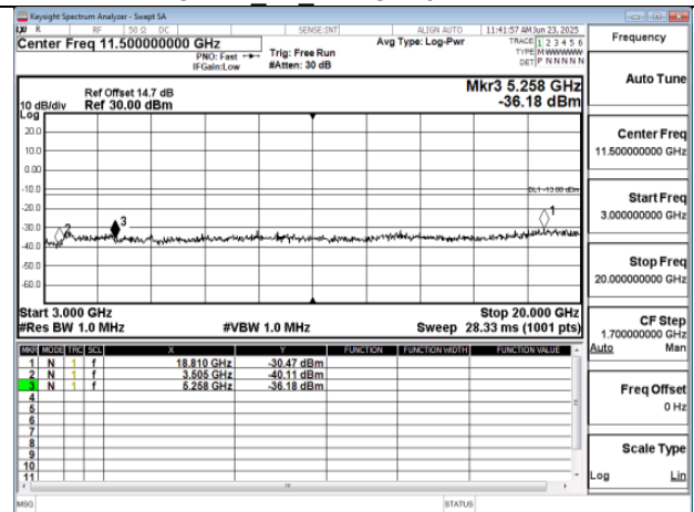
WCDMA B4 High CH1513-1752.6
