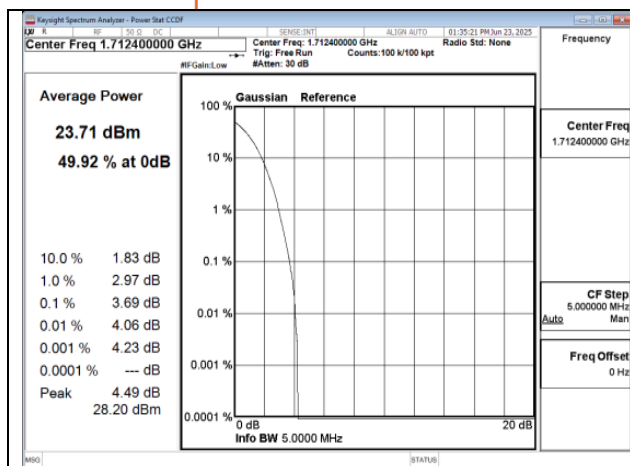
HSPA B4 Low CH1312-1712.4
