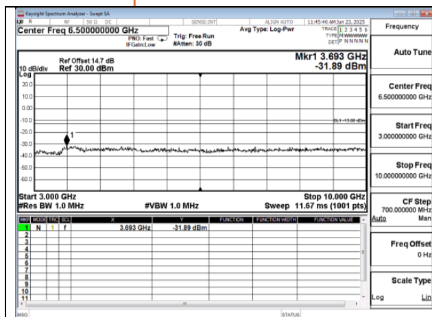
WCDMA_B5_Low_CH4132-826.4
