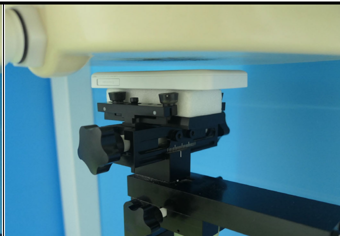
Rear Face of EUT Tested at 10 mm
