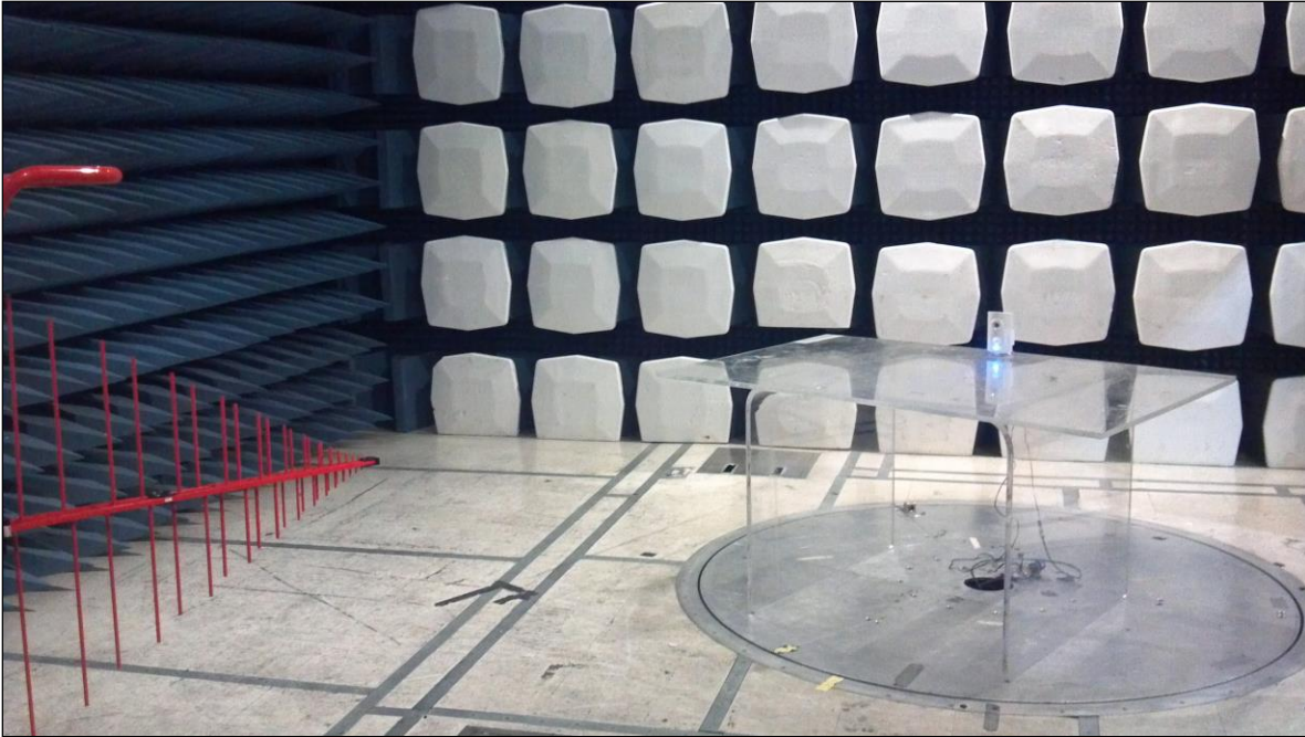
Photograph 4. Radiated Spurious Emissions, Test Setup, 30 MHz – 1 GHz
