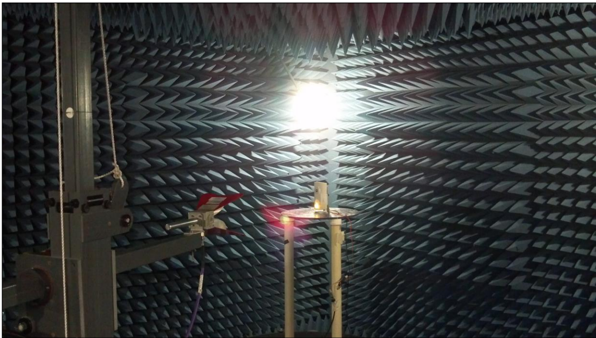
Photograph 5. Radiated Spurious Emissions, Test Setup, Above 1 GHz
