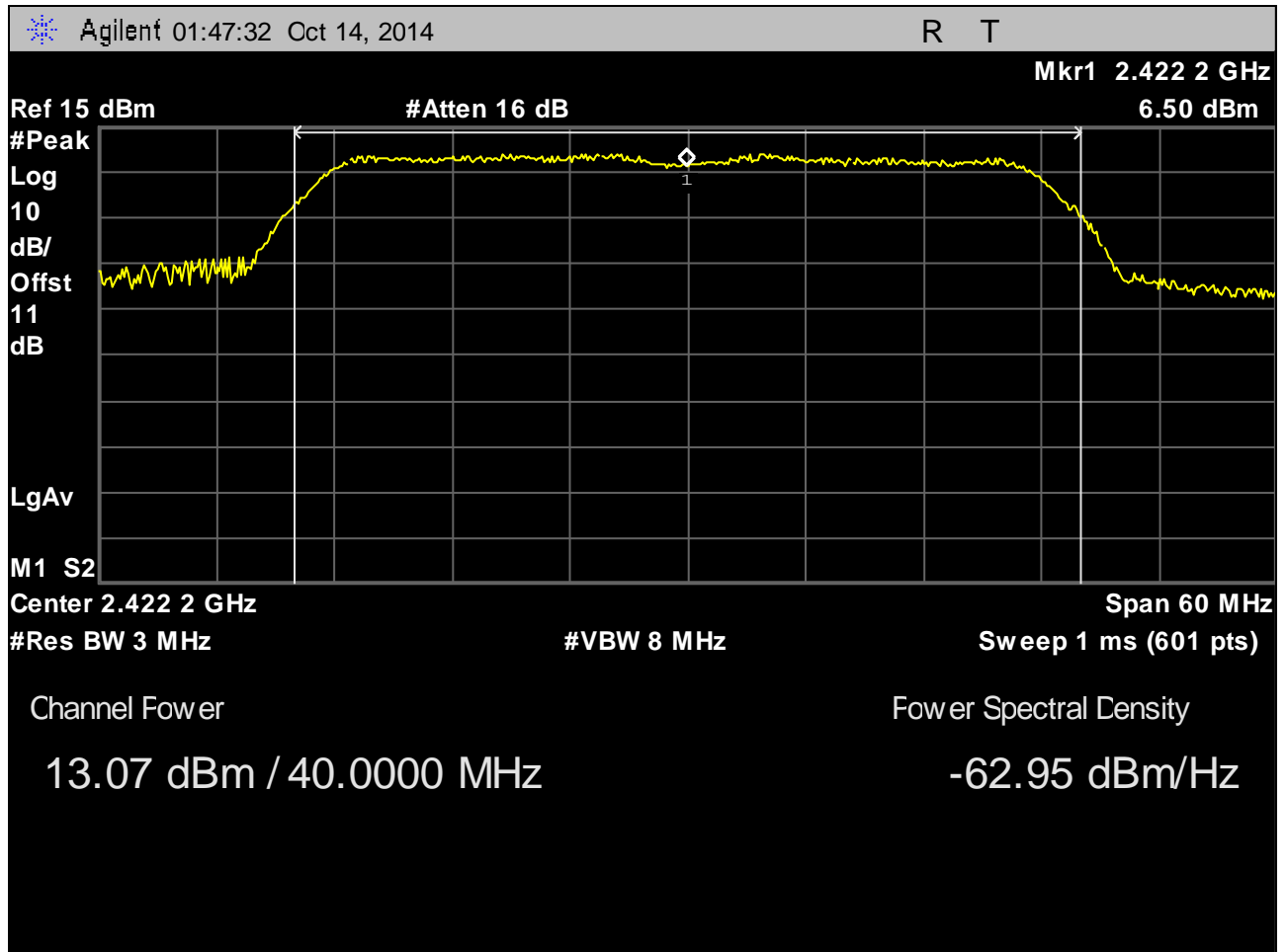
Plot 34. Peak Power Output, n Mode, 40 MHz, Low Channel
