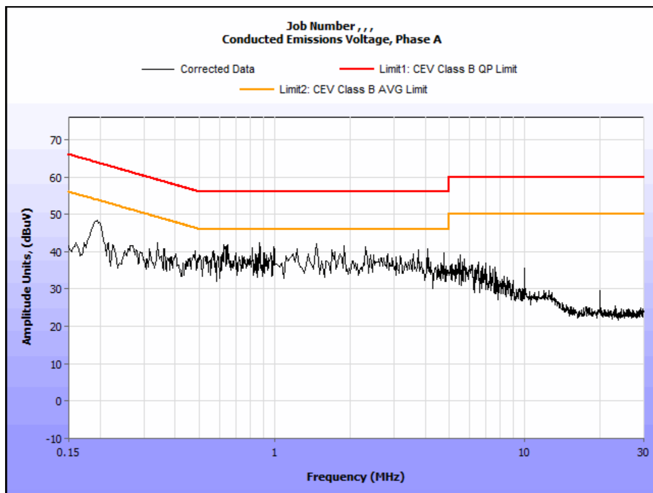
Plot 5. Conducted Emissions, 15.207(a), Phase Line
