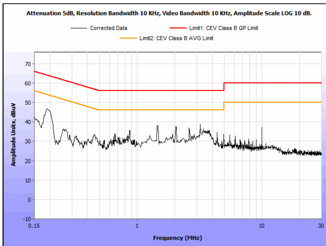
Plot 6. Conducted Emissions, 15.207(a), Neutral Line
