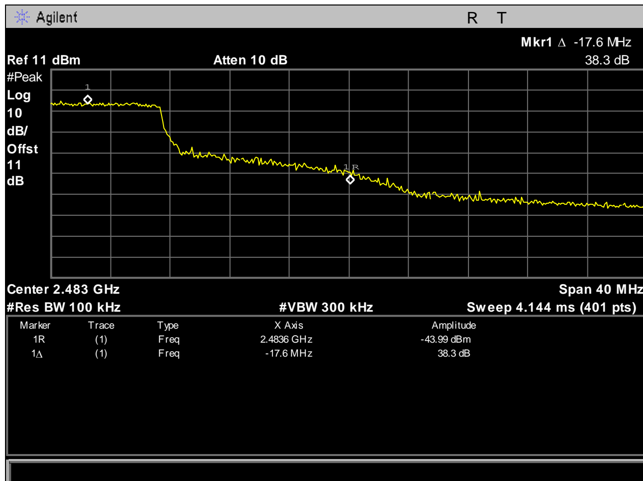
Plot 93. Conducted Band Edge, 2 mode (20 MHz) High
