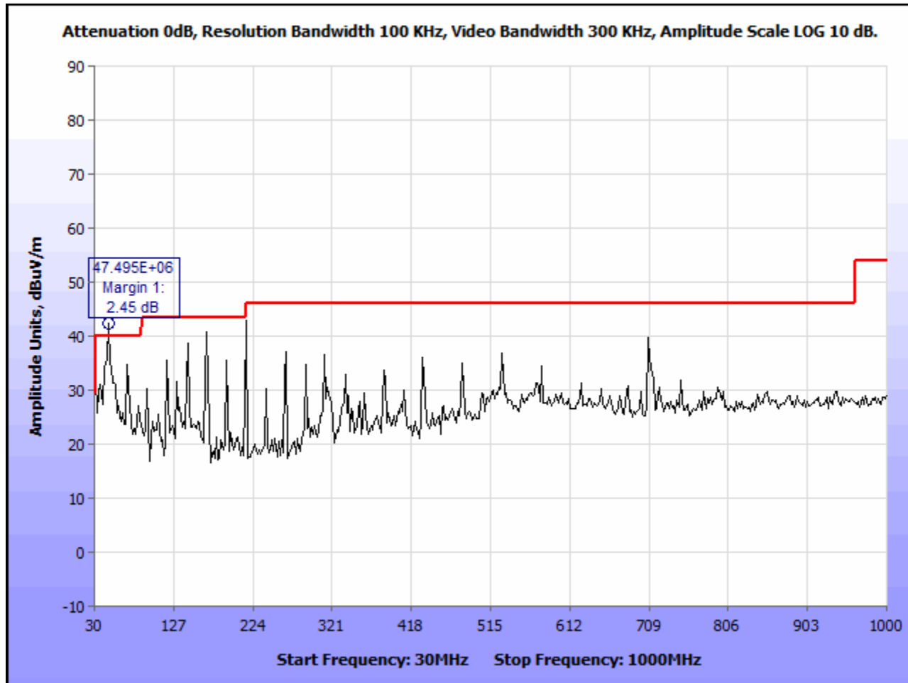
Plot 44. Radiated Spurious Emissions, Radio Off
