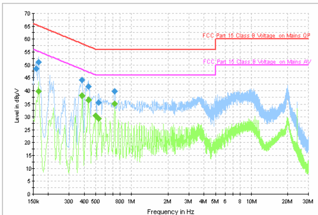
Figure A.6 Conducted Emission (Set.2, USB mode)
