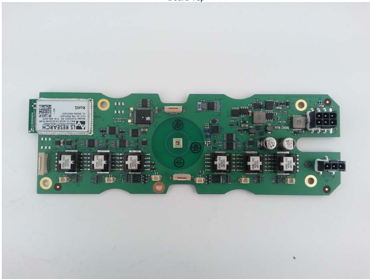
Board Top
