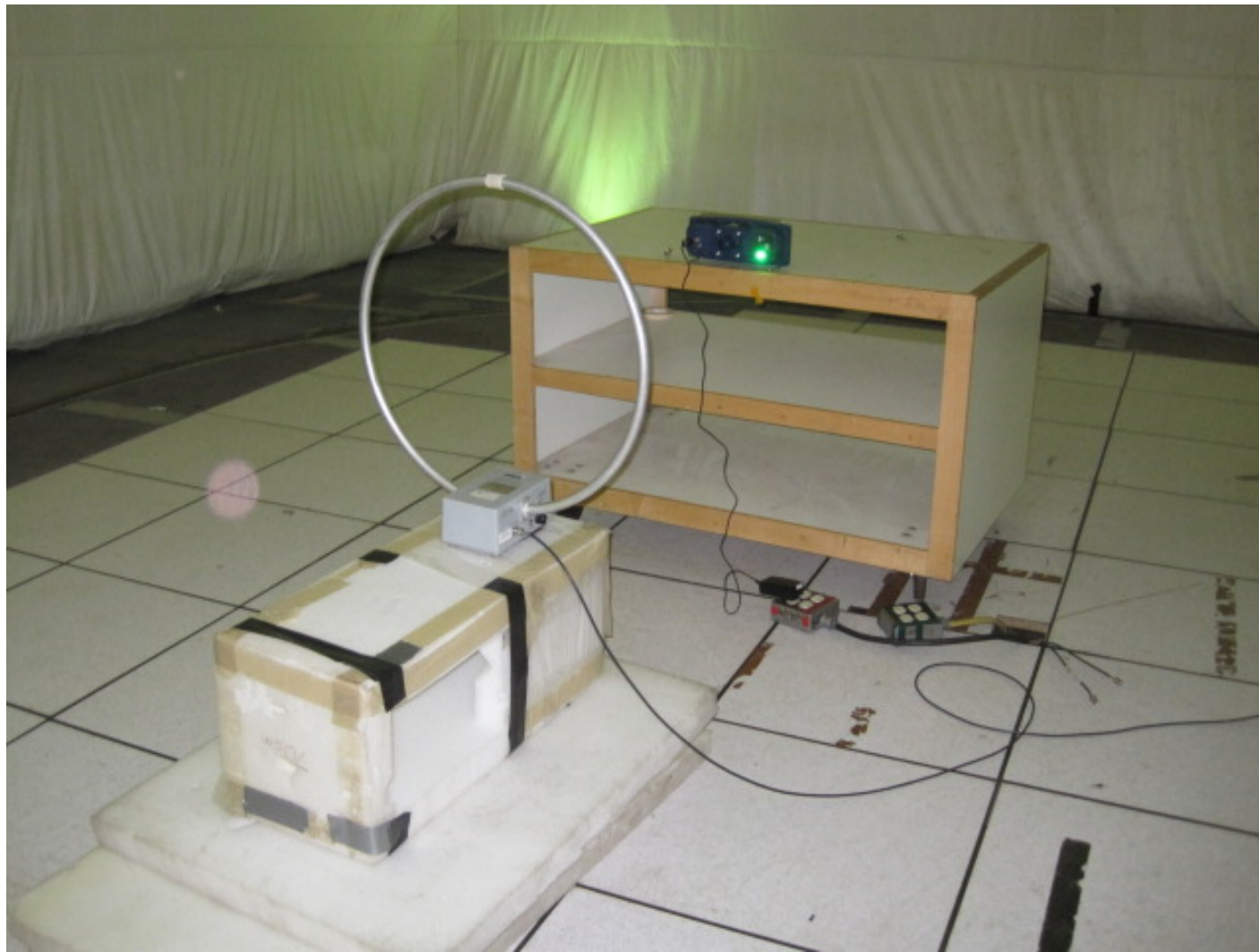
Test-setup photo(s):
