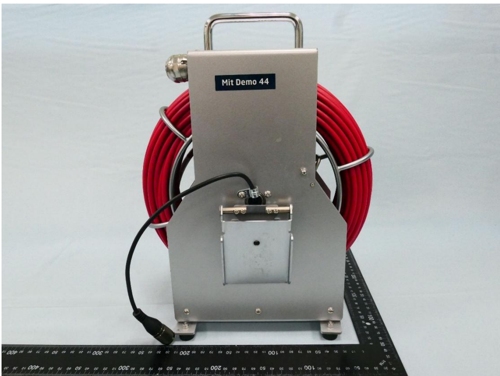
(26) EUT Photo - Probe(Vister series)
