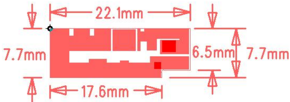
Chart 2 TYY-TX2506G-3 Antenna finished
