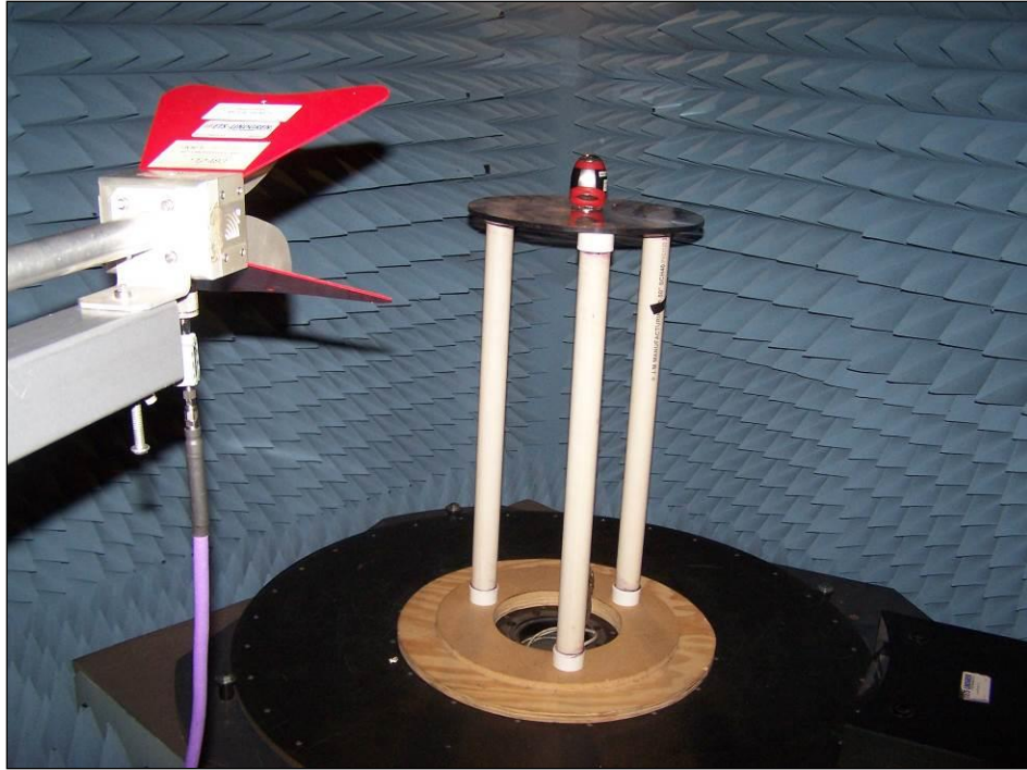
Photograph 4. Radiated Spurious Emissions, 1 GHz to 18 GHz, Test Setup
