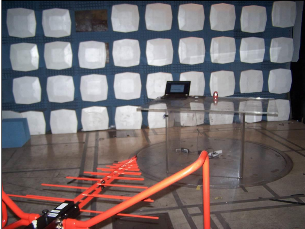
Photograph 6. Radiated Spurious Emissions, 30 MHz to 1 GHz, Test Setup
