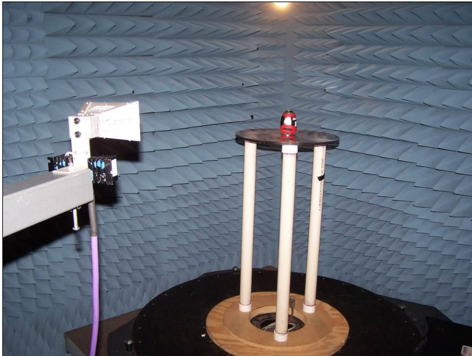
Photograph 5. Radiated Spurious Emissions, 18 GHz to 25 GHz, Test Setup
