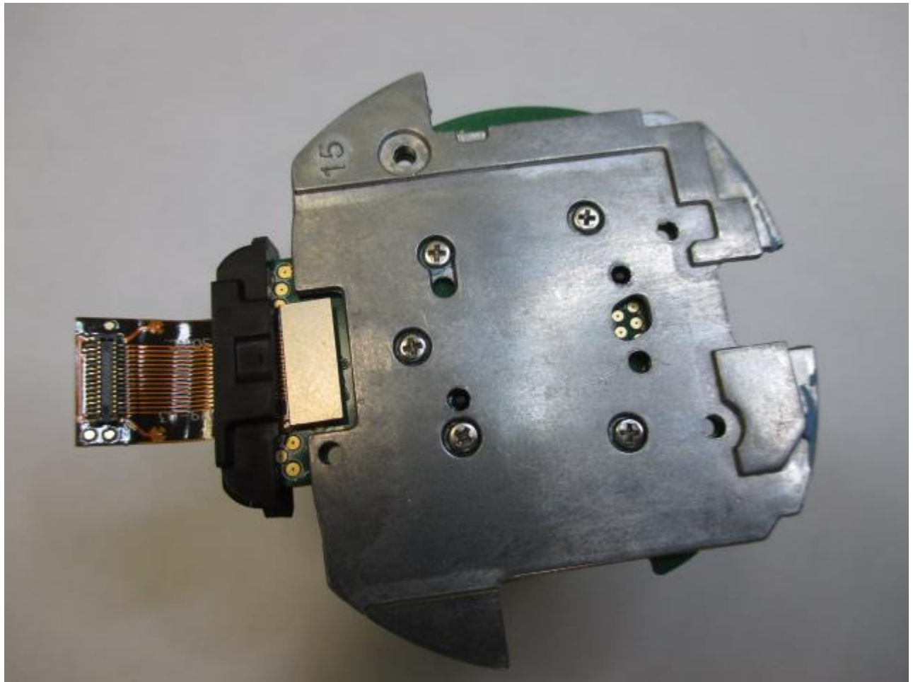
Photograph 7. Sensor & Lens Assy Bottom
