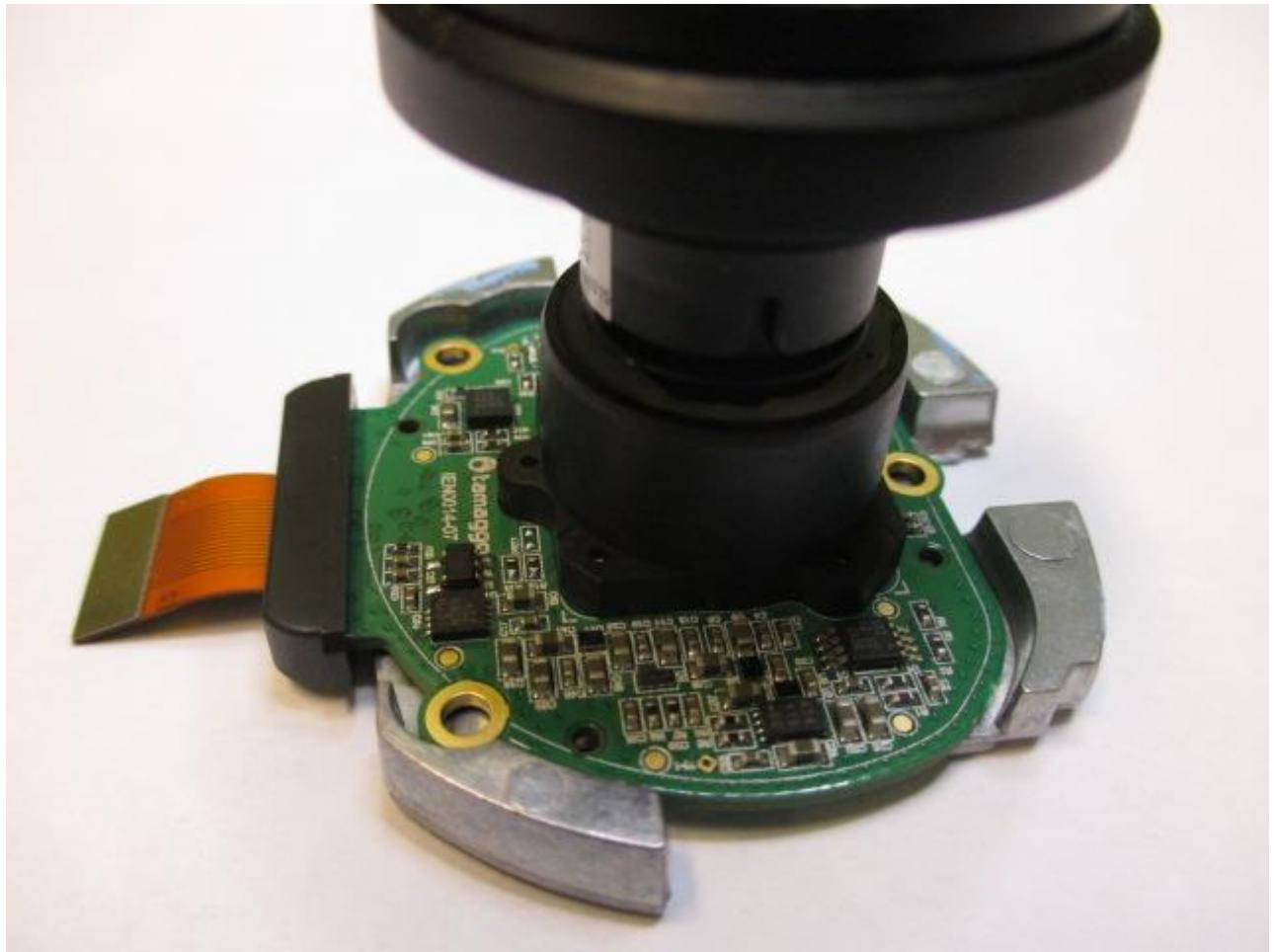
Photograph 8. Sensor & Lens Assy Top
