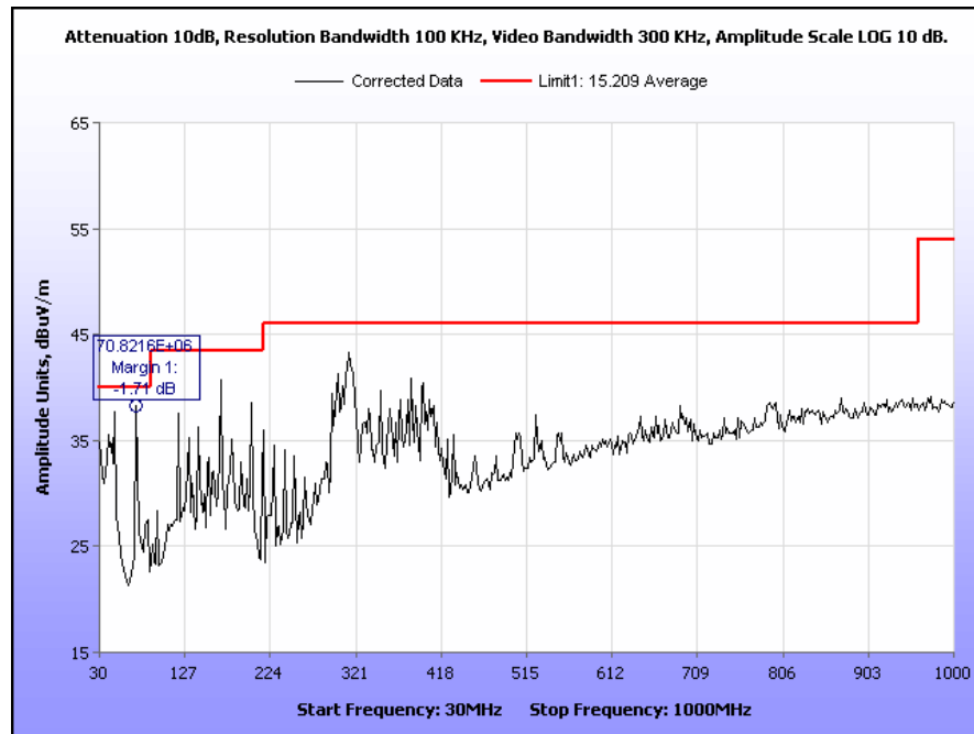
Plot 6. Radiated Emissions, 30 MHz - 1 GHz, FCC Limits, Mode 2- USB Connected to Power Supply
