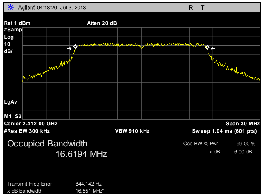
Plot 26. 99% Occupied Bandwidth, Low Channel g
