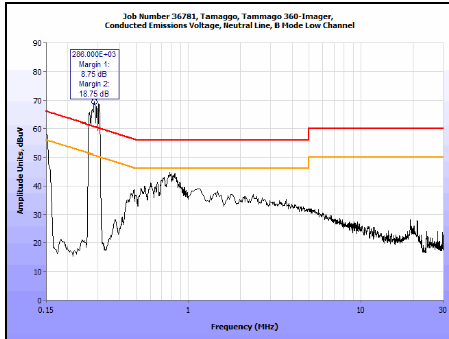
Plot 12. Conducted Emissions, 15.207(a), Low Channel b Neutral Line
