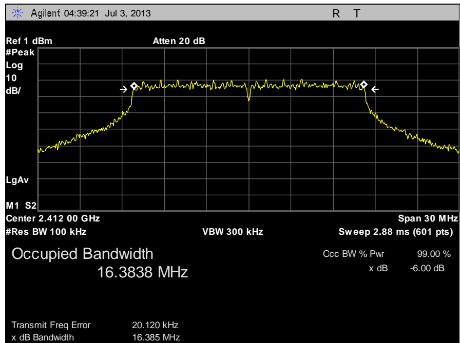
Plot 20. 6 dB Occupied Bandwidth, Low Channel g
