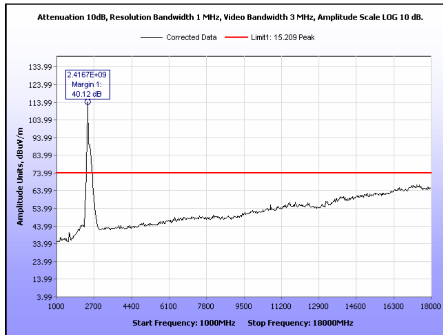
Plot 47. Radiated Spurious Emissions, Low Channel b, 1 GHz to 18 GHz
