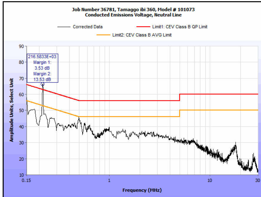
Plot 4. Conducted Emission, Neutral Line Plot
