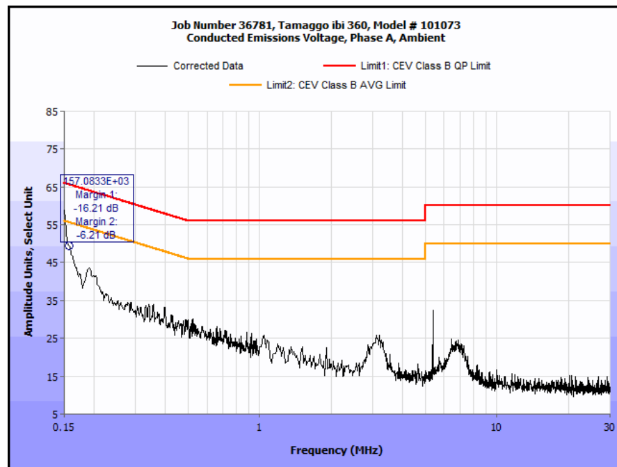
Plot 1. Conducted Emission, Phase Line Plot, Ambient
