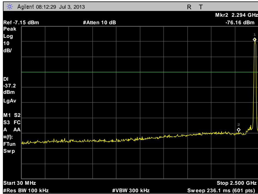
Plot 77. Conducted Spurious Emissions, High Channel g, 30 MHz to 2.5 GHz
