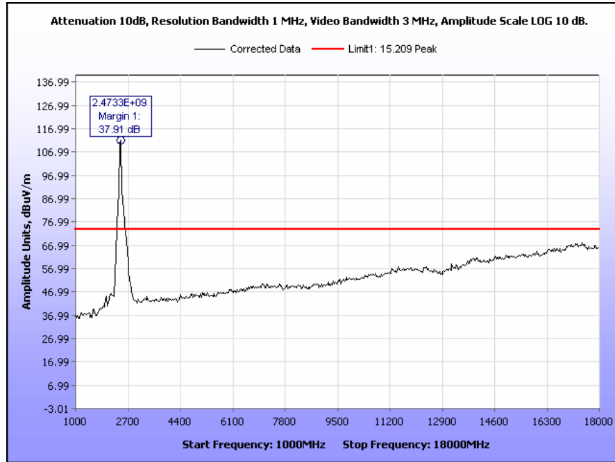
Plot 43. Radiated Spurious Emissions, High Channel b, 1 GHz to 18 GHz
