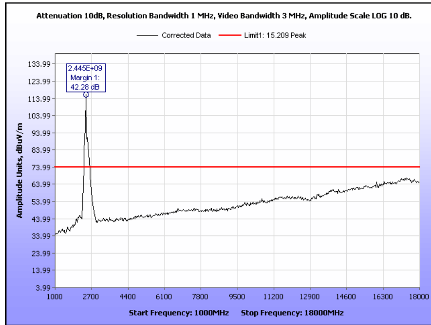
Plot 53. Radiated Spurious Emissions, Mid Channel g, 1 GHz to 18 GHz
