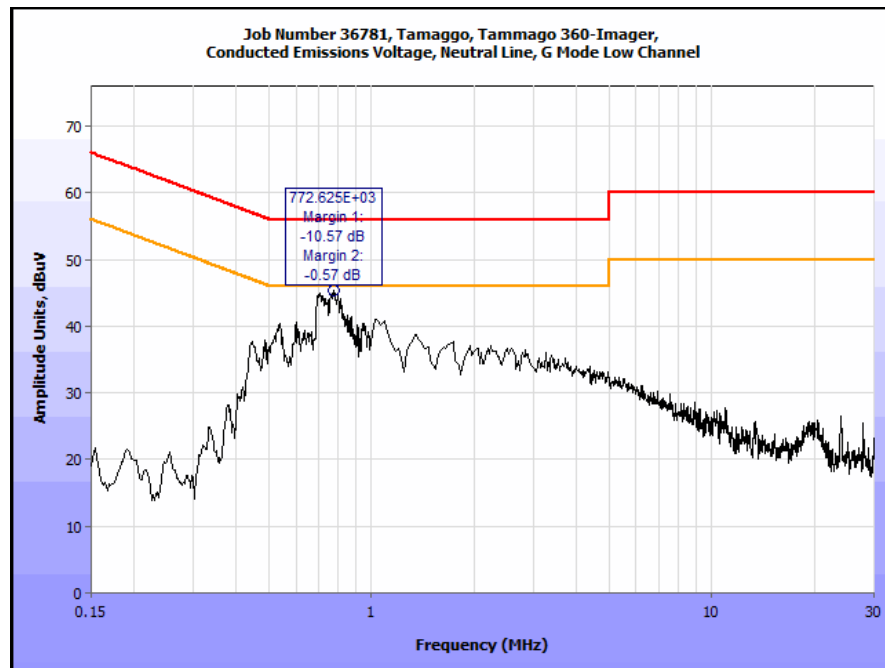
Plot 14. Conducted Emissions, 15.207(a), Low Channel g Neutral Line
