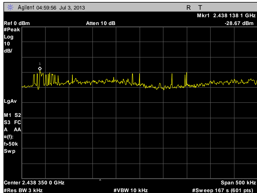
Plot 90. Peak Power Spectral Density, Mid Channel G
