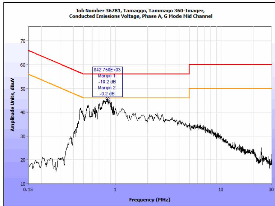
Plot 17. Conducted Emissions, 15.207(a), Mid Channel g Phase Line
