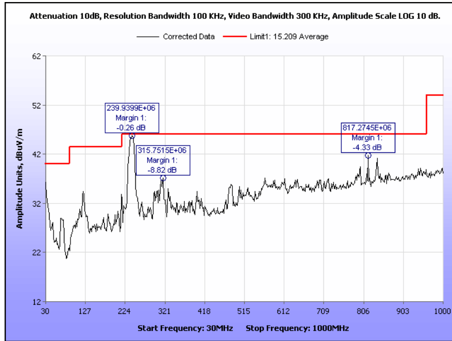
Plot 5. Radiated Emissions, 30 MHz – 1 GHz, FCC Limits, Mode 1-USB Connected to Laptop
