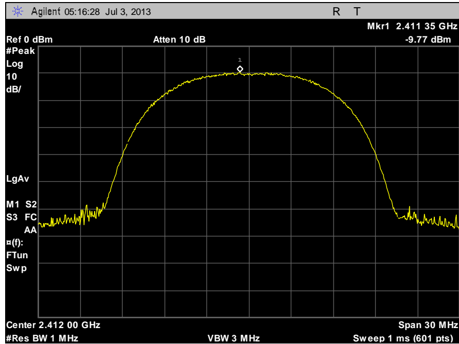
Plot 83. Peak Power Spectral Density, Low Channel B, Full Signal Peak
