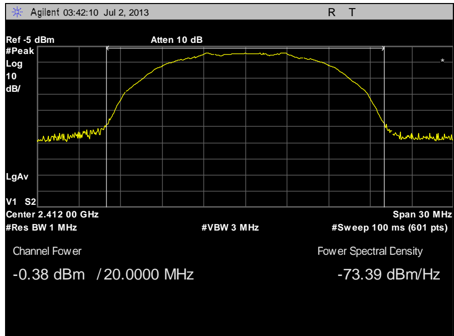
Plot 31. Peak Power Output, Channel 1 b
