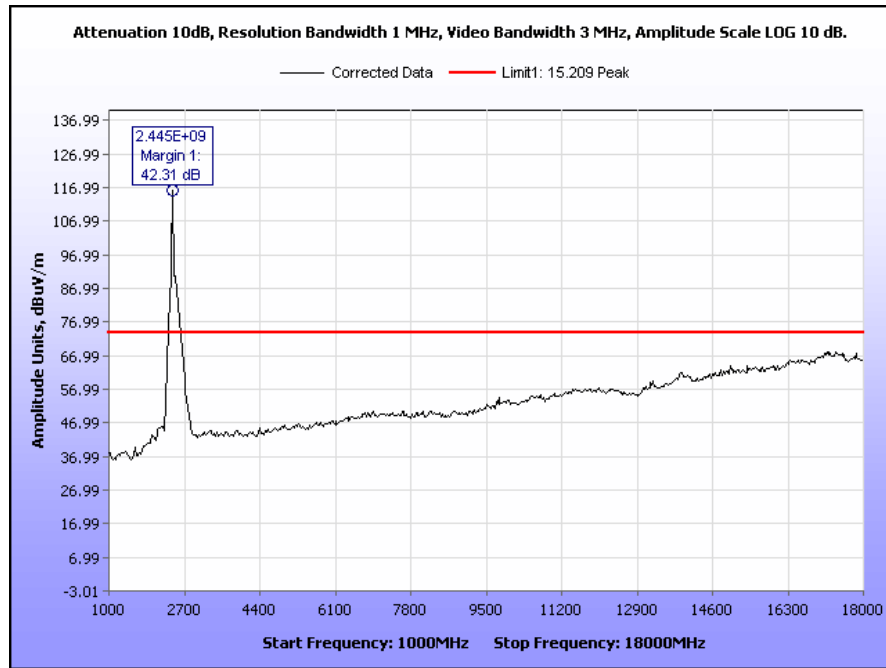
Plot 51. Radiated Spurious Emissions, Mid Channel b, 1 GHz to 18 GHz
