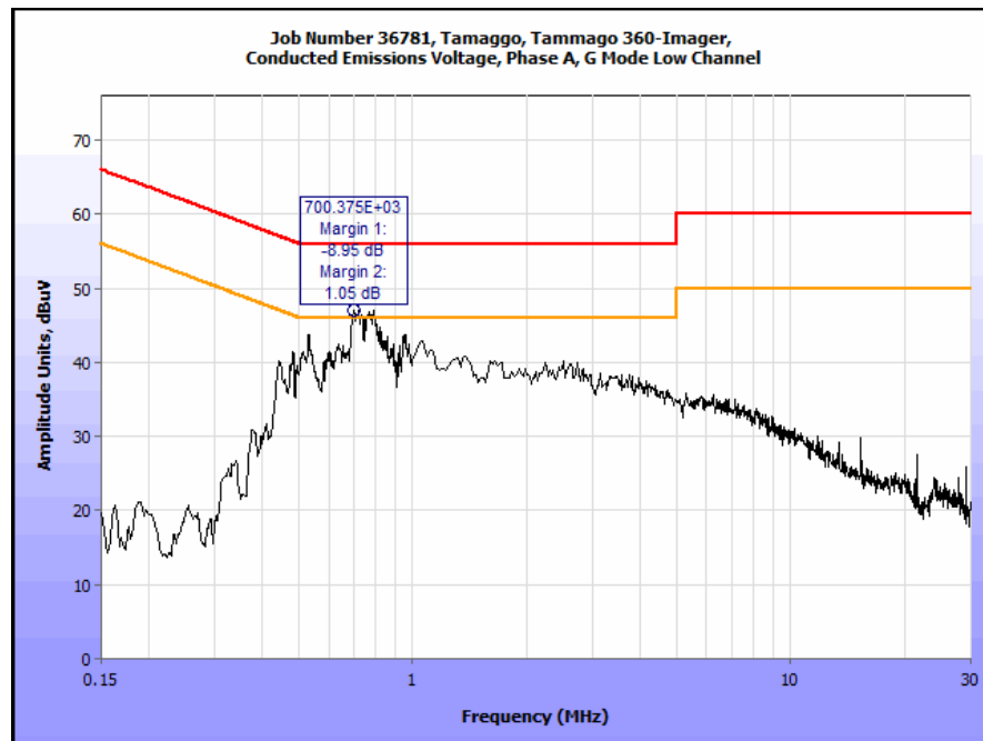
Plot 13. Conducted Emissions, 15.207(a), Low Channel g Phase Line
