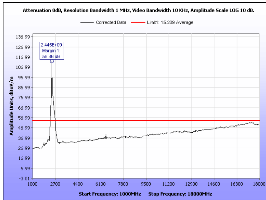
Plot 54. Radiated Spurious Emissions, Mid Channel g, 1 GHz to 18 GHz Average
