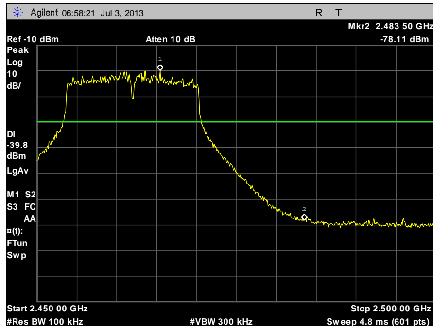
Plot 80. Conducted Spurious Emissions, High Channel g, Band Edge
