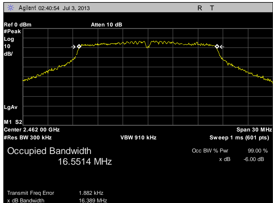
Plot 24. 6 dB Occupied Bandwidth, High Channel g
