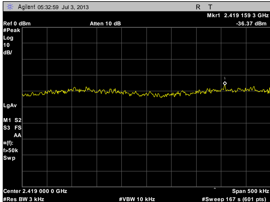
Plot 86. Peak Power Spectral Density, Low Channel G
