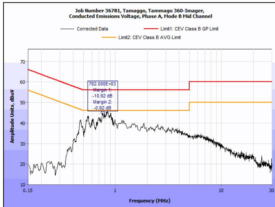
Plot 15. Conducted Emissions, 15.207(a), Mid Channel b Phase Line
