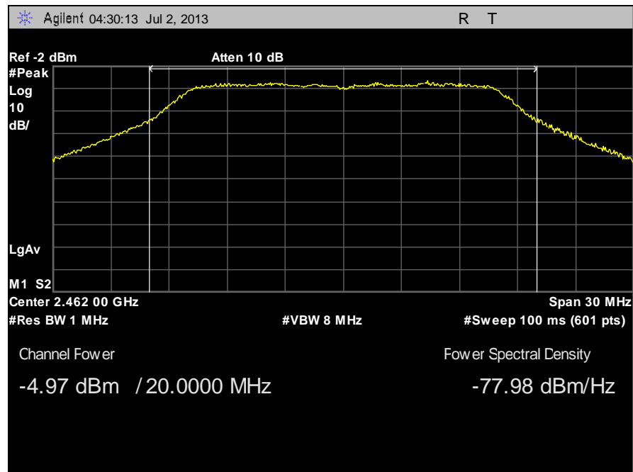
Plot 36. Peak Power Output, Channel 11 g
