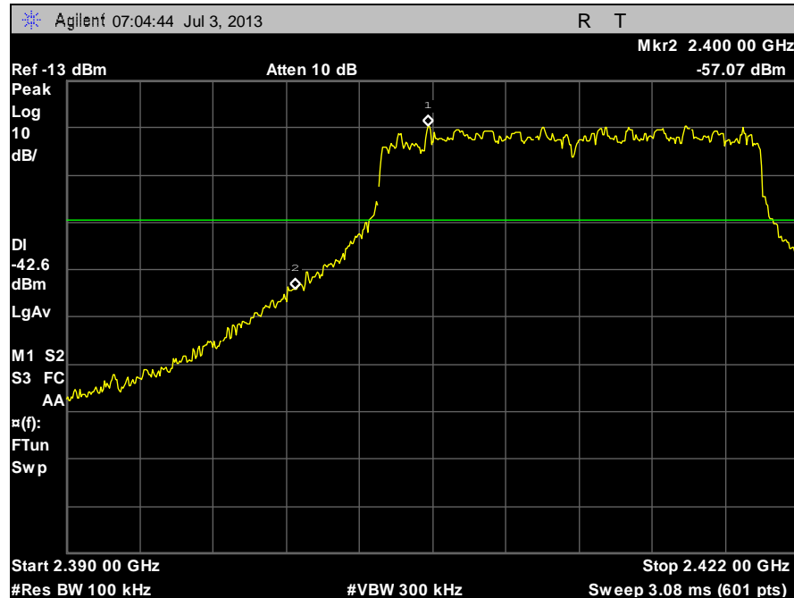
Plot 82. Conducted Spurious Emissions, Low Channel g, Band Edge
