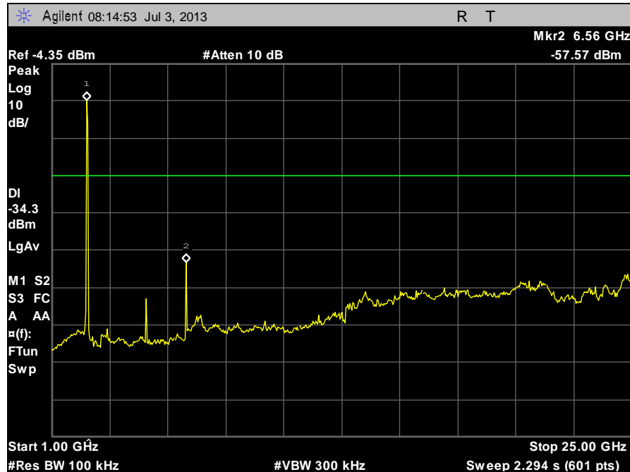
Plot 78. Conducted Spurious Emissions, High Channel b, 1 GHz to 25 GHz
