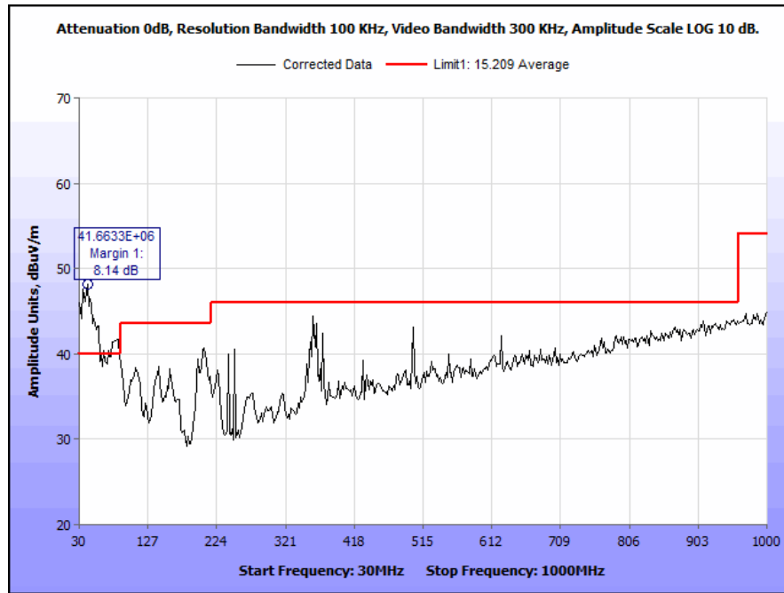
Plot 39. Radiated Spurious Emissions, Low Channel b, 30 MHz to 1 GHz
