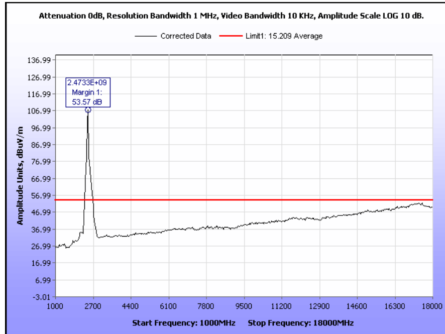
Plot 46. Radiated Spurious Emissions, High Channel g, 1 GHz to 18 GHz Average
