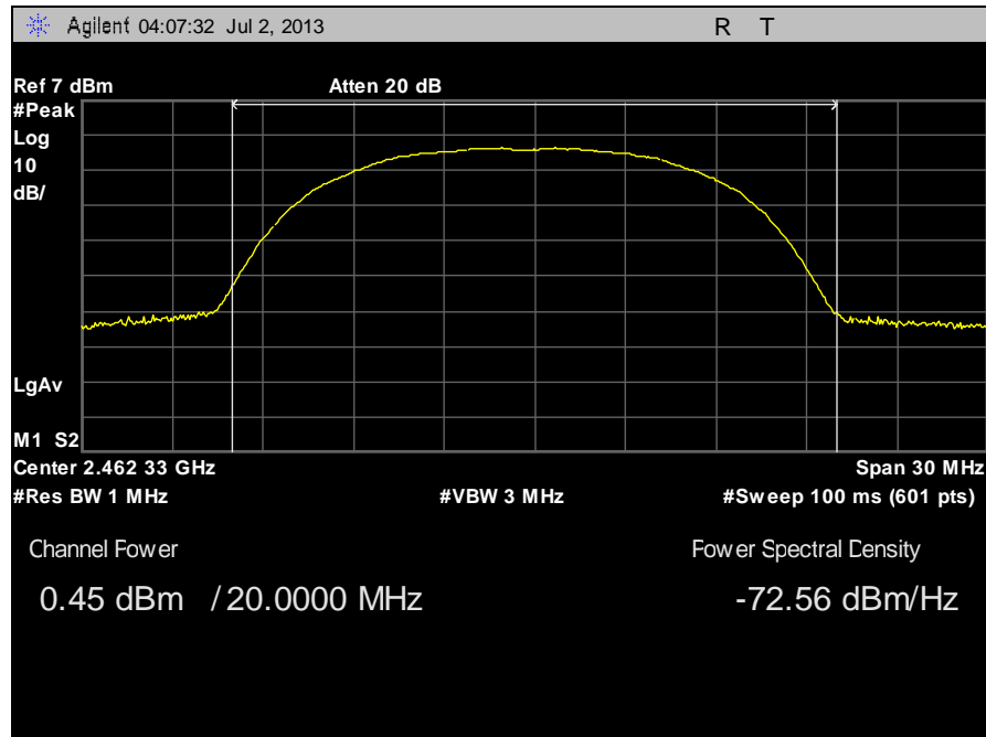
Plot 35. Peak Power Output, Channel 11 b
