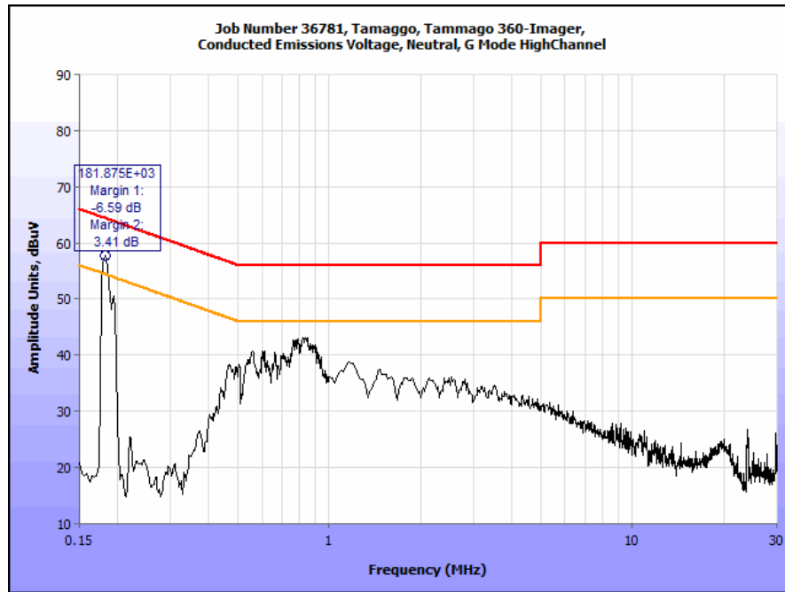
Plot 10. Conducted Emissions, 15.207(a), High Channel g Neutral Line
