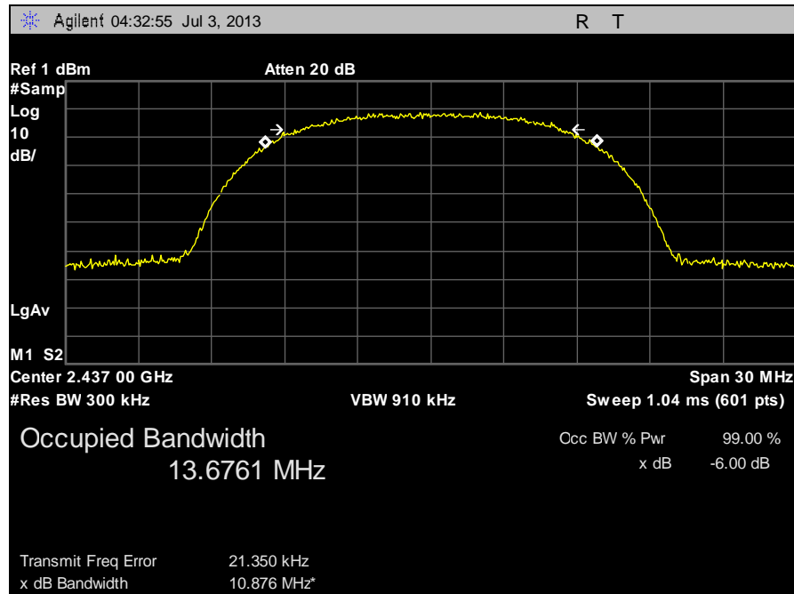
Plot 27. 99% Occupied Bandwidth, Mid Channel b
