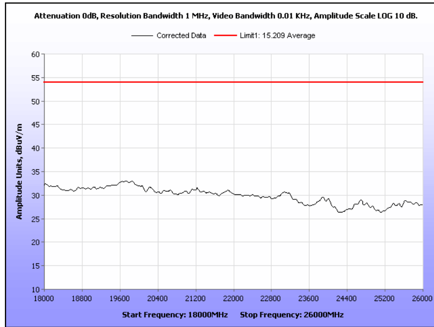
Plot 55. Radiated Spurious Emissions, High Channel b, 18 GHz to 26 GHz Average
