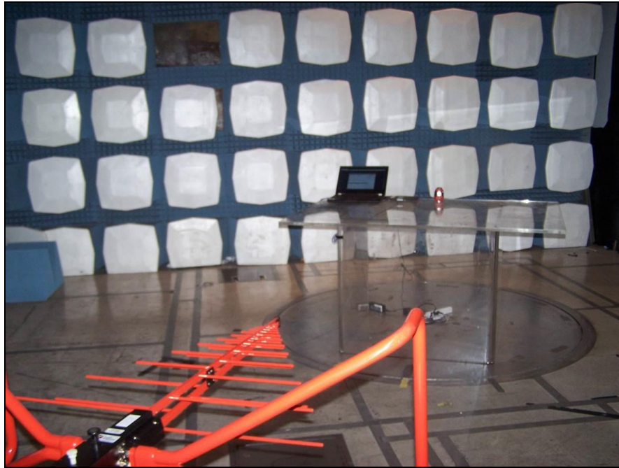
Photograph 7. Radiated Spurious Emissions, 30 MHz to 1 GHz, Test Setup
