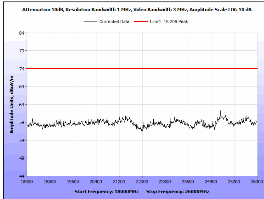
Plot 65. Radiated Spurious Emissions, Mid Channel b, 18 GHz to 26 GHz Peak
