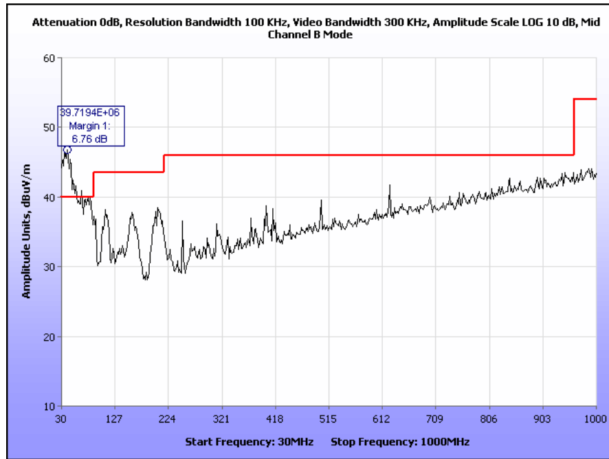
Plot 41. Radiated Spurious Emissions, Mid Channel b, 30 MHz to 1 GHz
