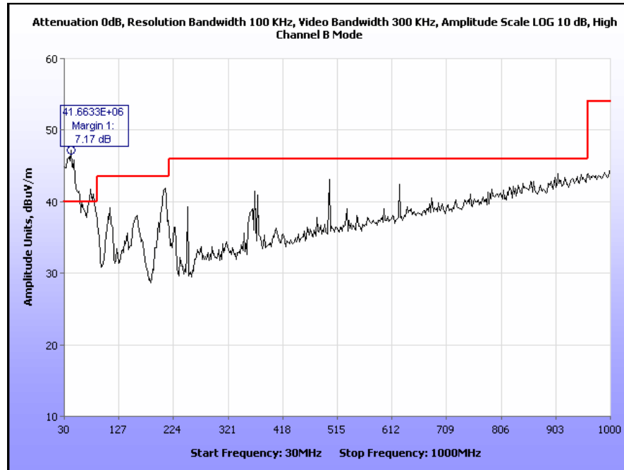
Plot 37. Radiated Spurious Emissions, High Channel B, 30 MHz to 1 GHz
