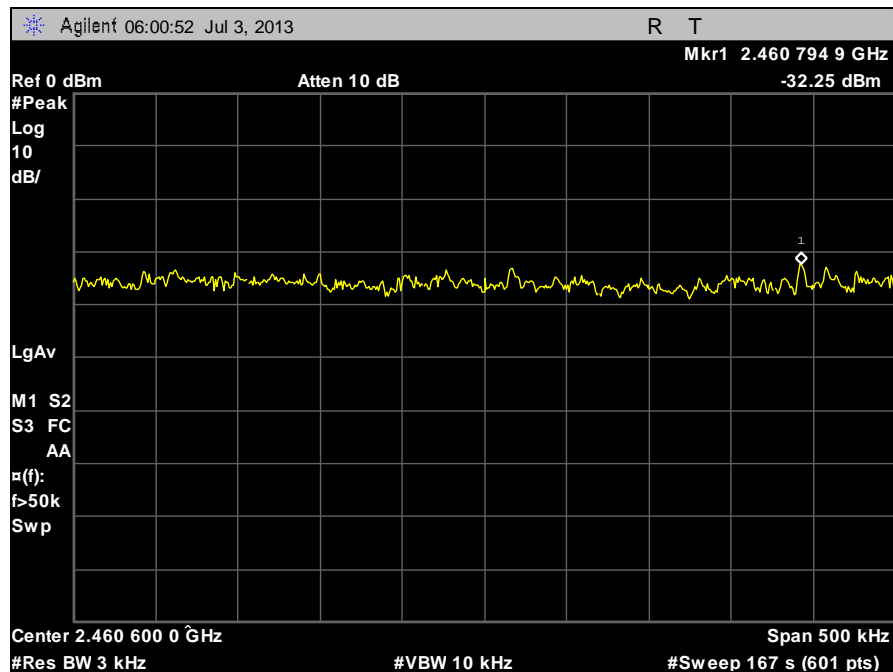
Plot 92. Peak Power Spectral Density, High Channel B
