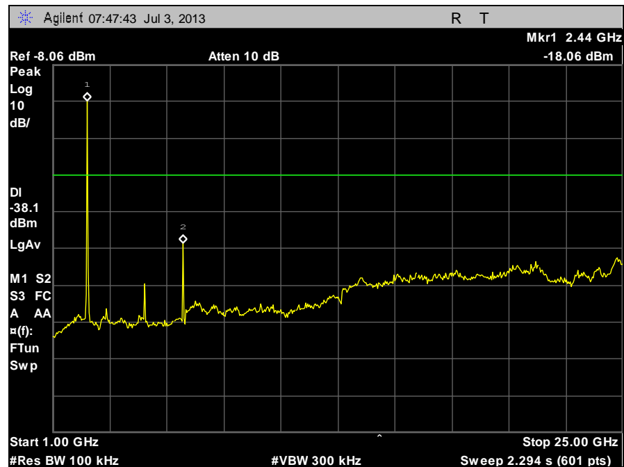
Plot 74. Conducted Spurious Emissions, Mid Channel g, 1 GHz – 25 GHz
