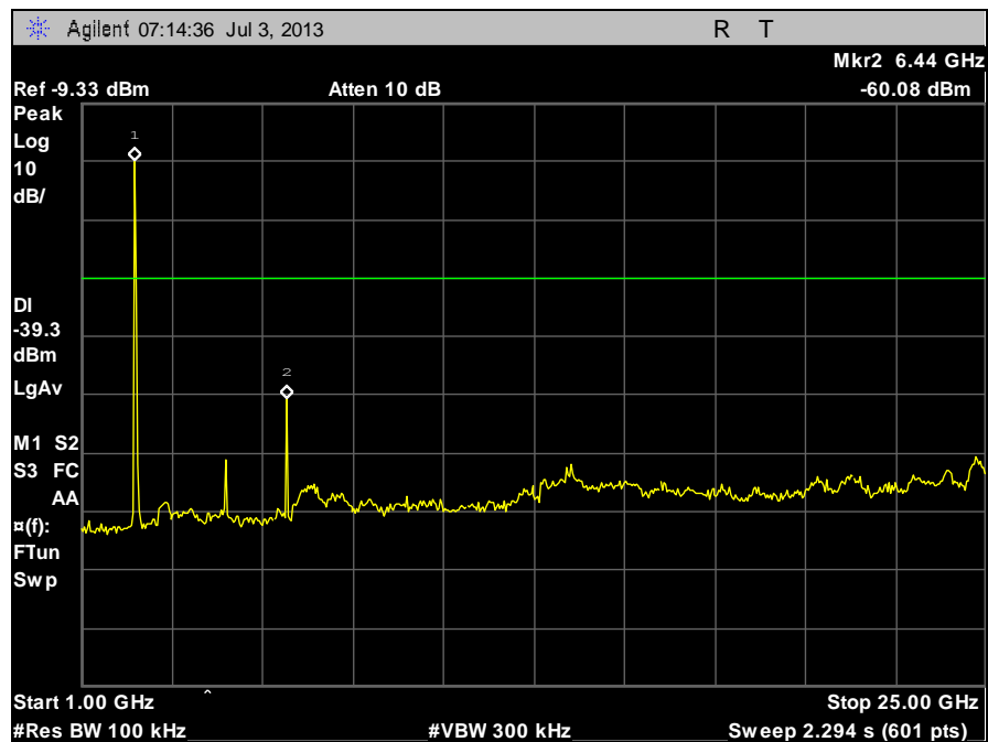
Plot 68. Conducted Spurious Emissions, Low Channel b, 1 GHz – 25 GHz
