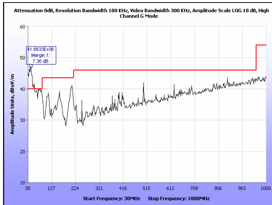
Plot 38. Radiated Spurious Emissions, High Channel g, 30 MHz to 1 GHz
