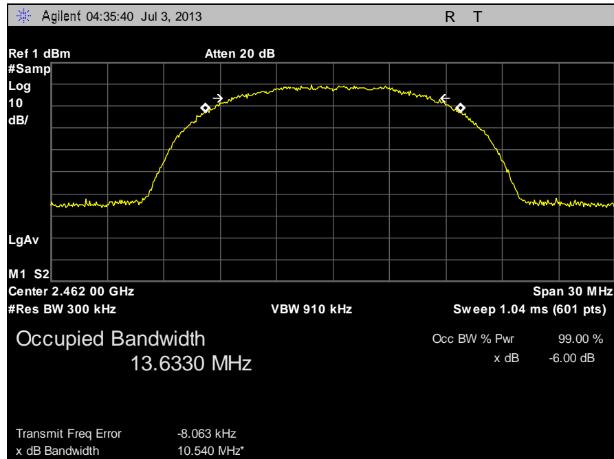
Plot 29. 99% Occupied Bandwidth, High Channel b
