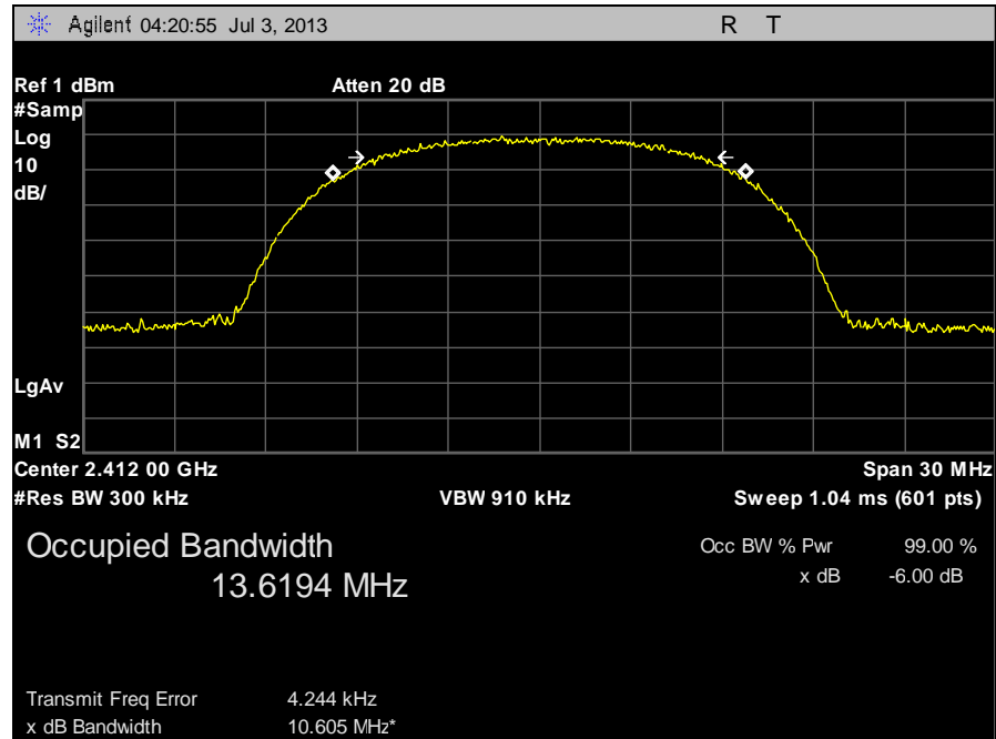
Plot 25. 99% Occupied Bandwidth, Low Channel b
