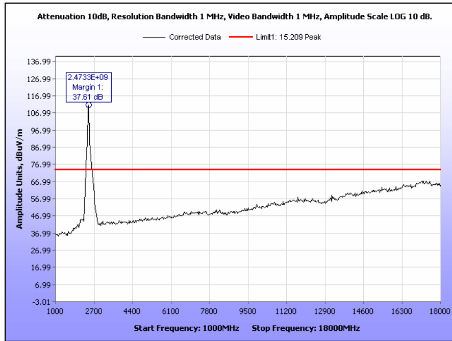
Plot 45. Radiated Spurious Emissions, High Channel g, 1 GHz to 18 GHz
