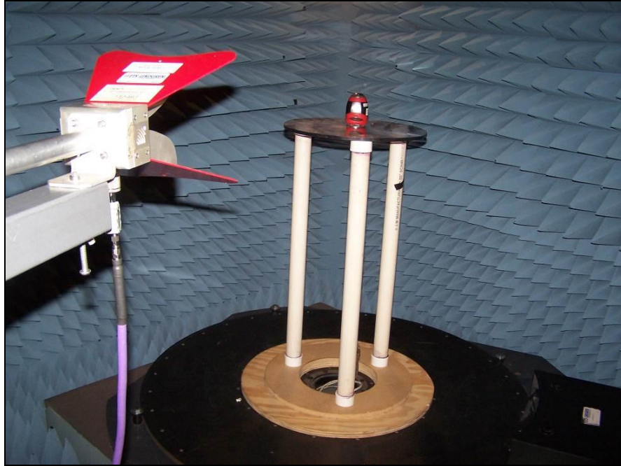
Photograph 5. Radiated Spurious Emissions, 1 GHz to 18 GHz, Test Setup
