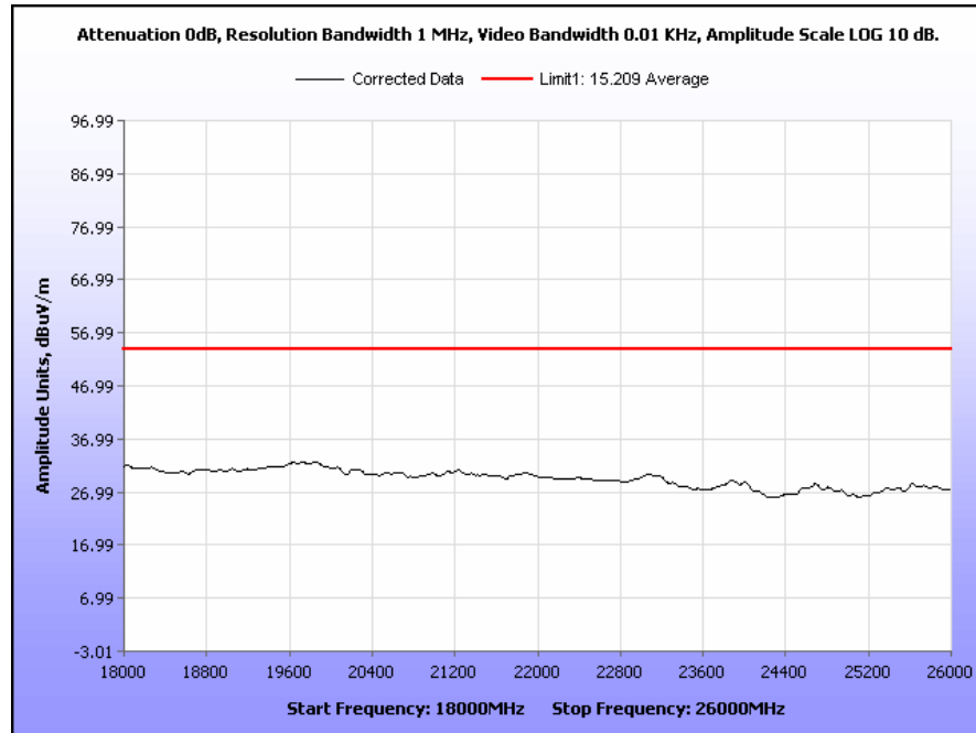
Plot 58. Radiated Spurious Emissions, Low Channel g, 18 GHz to 26 GHz Average
