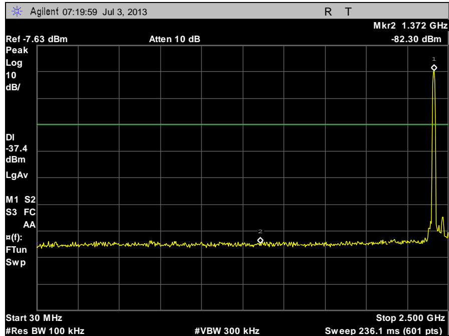
Plot 67. Conducted Spurious Emissions, Low Channel b, 30 MHz – 2.5 GHz
