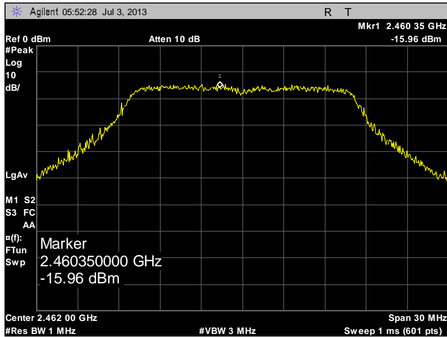
Plot 93. Peak Power Spectral Density, High Channel G, Full Signal Peak
