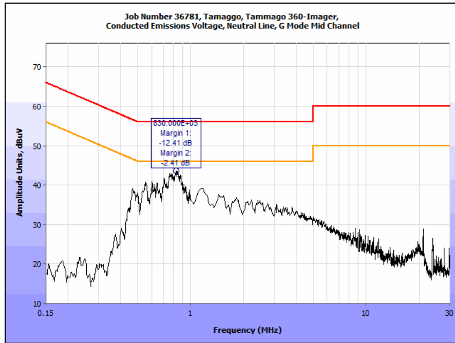
Plot 18. Conducted Emissions, 15.207(a), Mid Channel g Neutral Line
