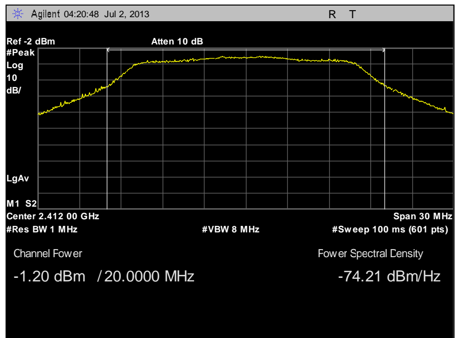
Plot 32. Peak Power Output, Channel 1 g
