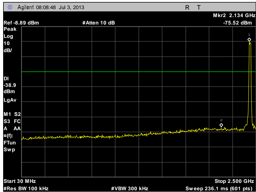
Plot 73. Conducted Spurious Emissions, Mid Channel g, 30 MHz – 2.5 GHz
