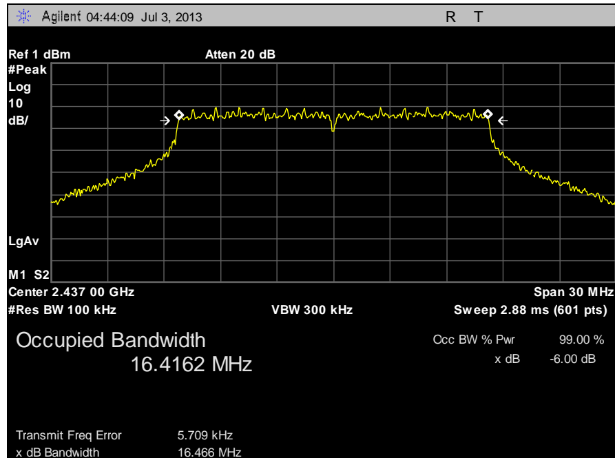
Plot 22. 6 dB Occupied Bandwidth, Mid Channel g
