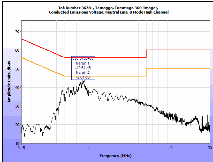
Plot 8. Conducted Emissions, 15.207(a), High Channel b Neutral Line
