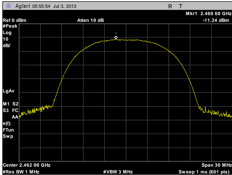
Plot 91. Peak Power Spectral Density, High Channel B, Full Signal Peak
