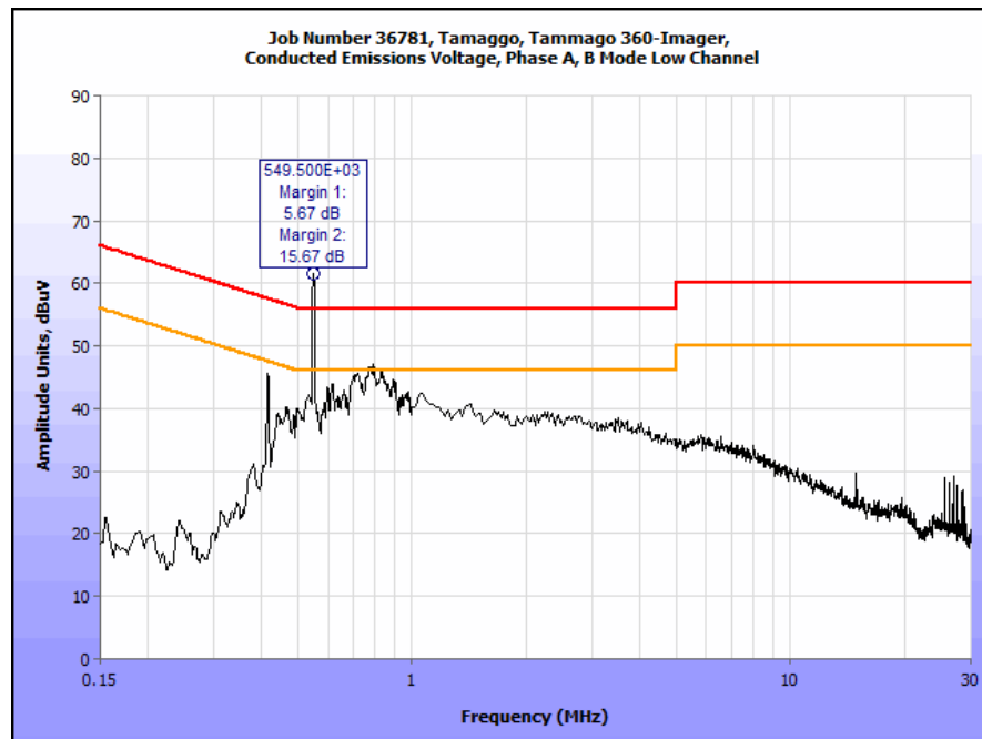
Plot 11. Conducted Emissions, 15.207(a), Low Channel g Phase Line
