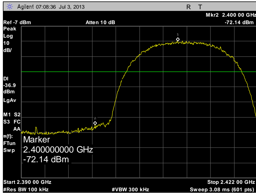
Plot 81. Conducted Spurious Emissions, Low Channel b, Band Edge
