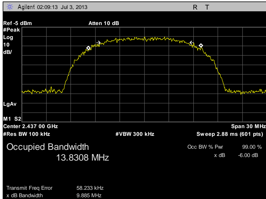
Plot 21. 6 dB Occupied Bandwidth, Mid Channel b
