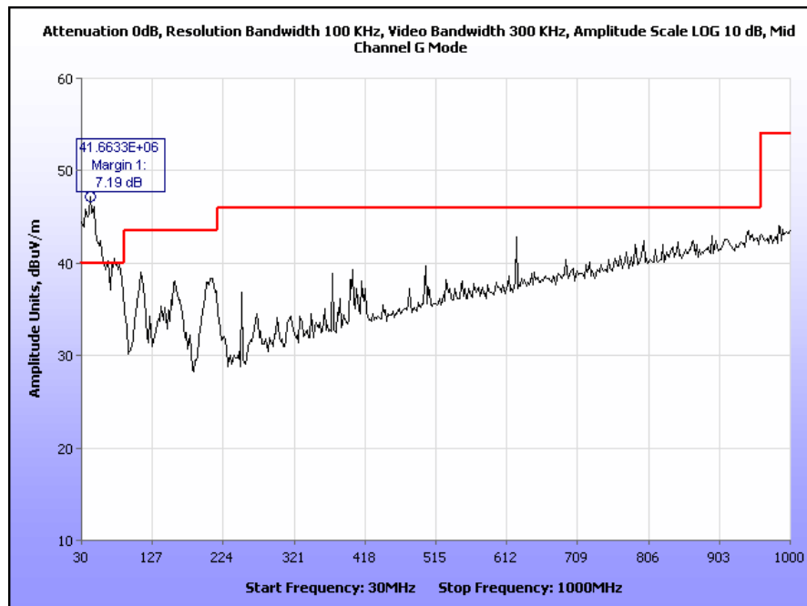
Plot 42. Radiated Spurious Emissions, Mid Channel g, 30 MHz to 1 GHz
