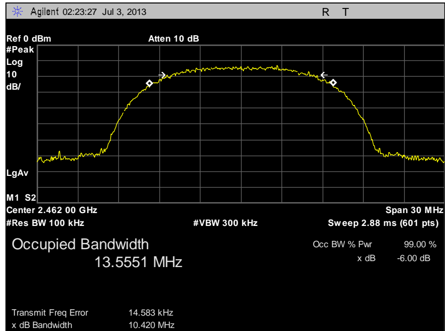
Plot 23. 6 dB Occupied Bandwidth, High Channel b
