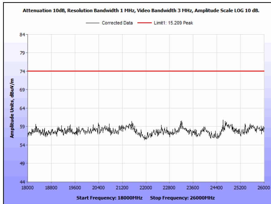
Plot 64. Radiated Spurious Emissions, Low Channel g, 18 GHz to 26 GHz Peak
