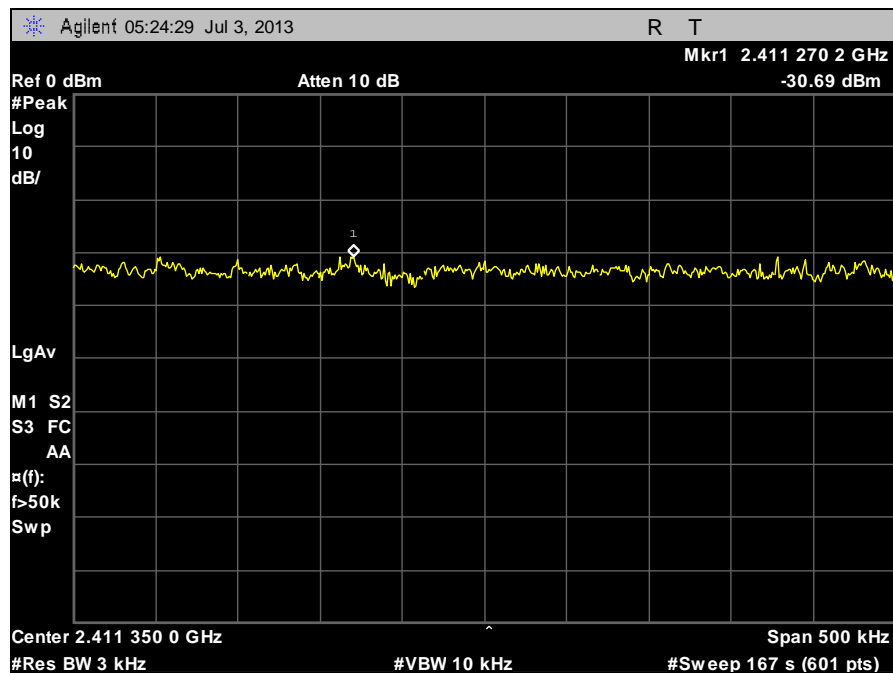
Plot 84. Peak Power Spectral Density, Low Channel B
