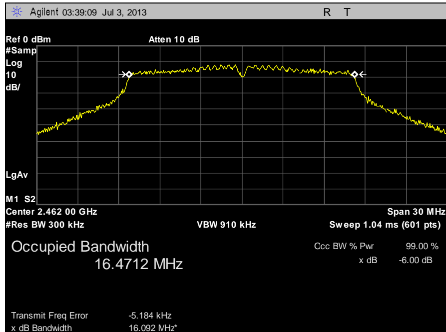
Plot 30. 99% Occupied Bandwidth, High Channel g
