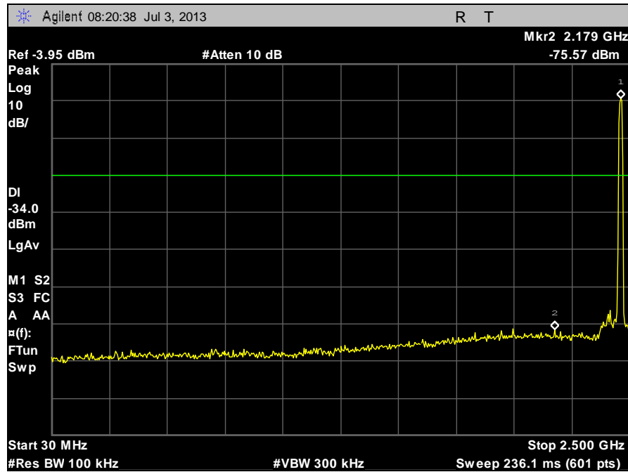
Plot 75. Conducted Spurious Emissions, High Channel b, 30 MHz to 2.5 GHz
