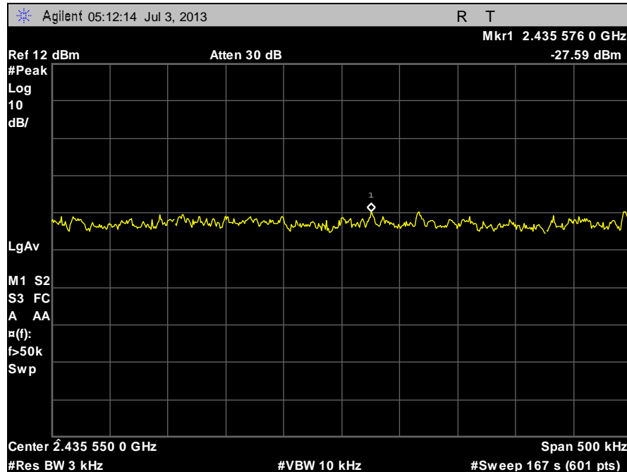
Plot 88. Peak Power Spectral Density, Mid Channel B
