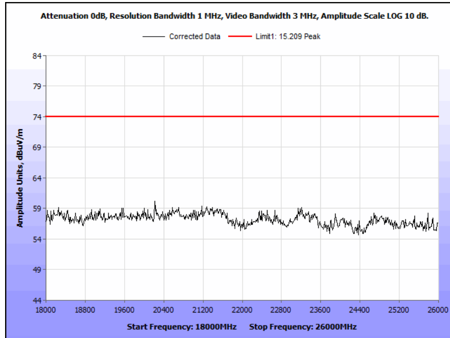
Plot 62. Radiated Spurious Emissions, High Channel g, 18 GHz to 26 GHz Peak
