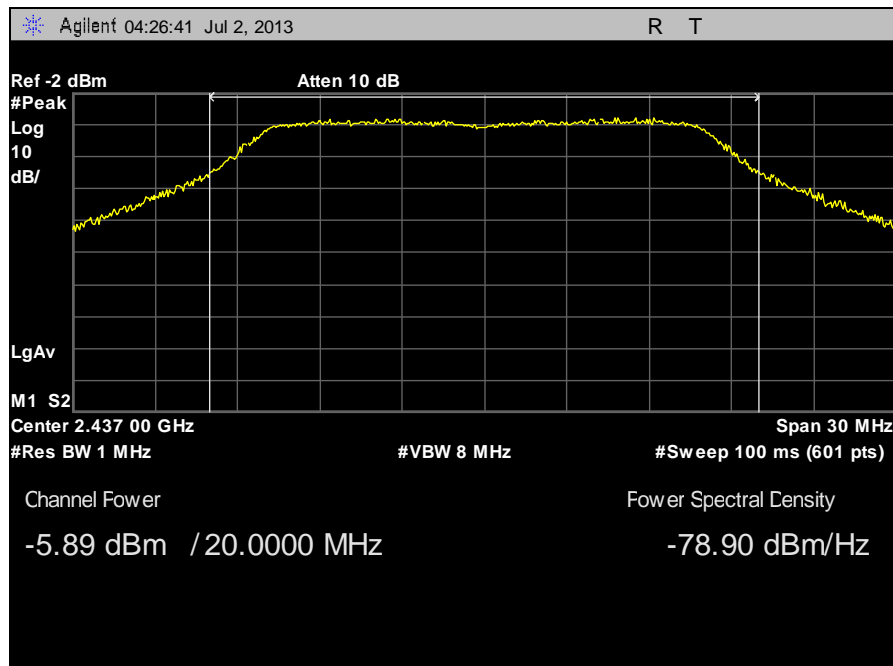
Plot 34. Peak Power Output, Channel 6 g
