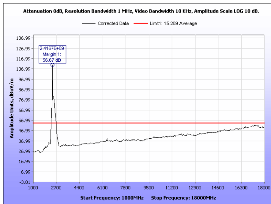
Plot 48. Radiated Spurious Emissions, Low Channel b, 1 GHz to 18 GHz Average
