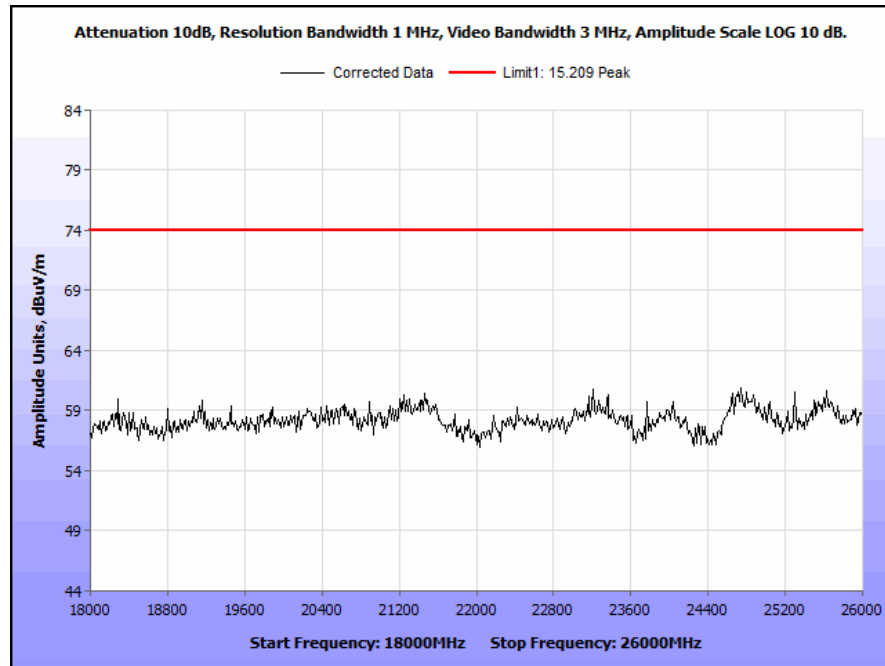
Plot 63. Radiated Spurious Emissions, Low Channel b, 18 GHz to 26 GHz Peak
