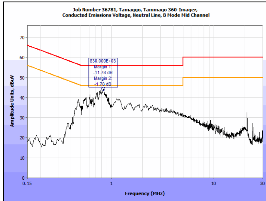
Plot 16. Conducted Emissions, 15.207(a), Mid Channel b Neutral Line
