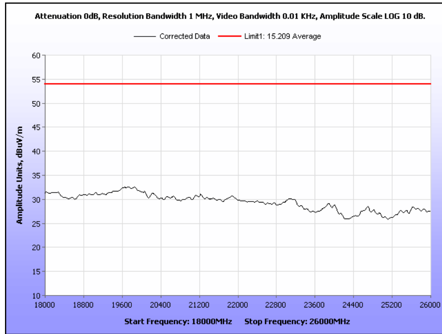
Plot 57. Radiated Spurious Emissions, Low Channel b, 18 GHz to 26 GHz Average
