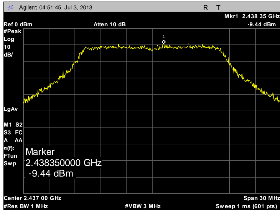
Plot 89. Peak Power Spectral Density, Mid Channel G, Full Signal Peak
