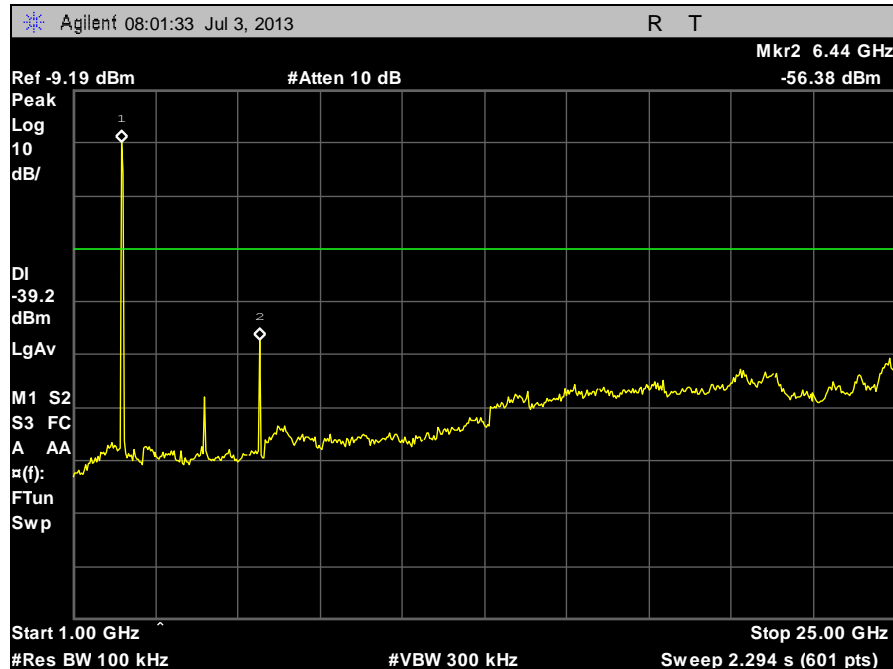
Plot 70. Conducted Spurious Emissions, Low Channel g, 1 GHz – 25 GHz
