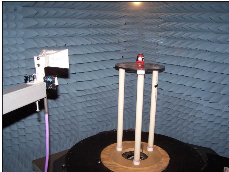
Photograph 6. Radiated Spurious Emissions, 18 GHz to 25 GHz, Test Setup
