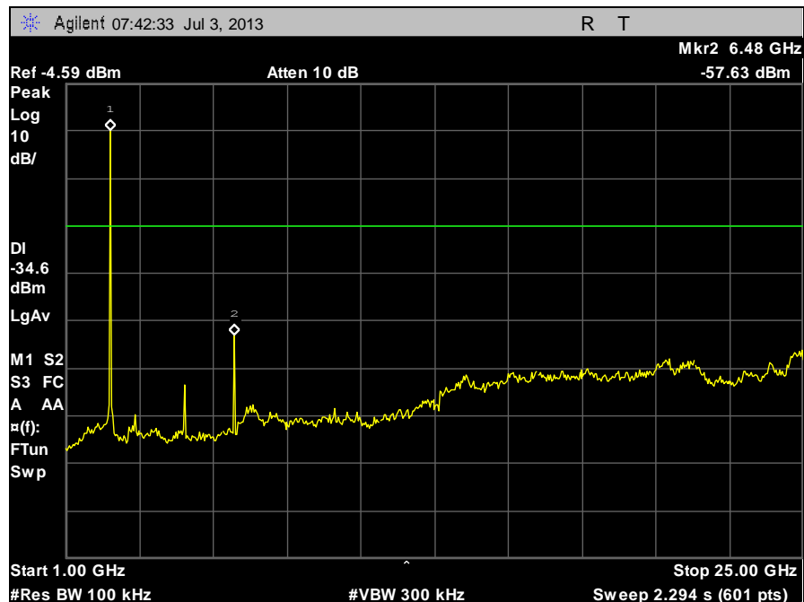
Plot 72. Conducted Spurious Emissions, Mid Channel b, 1 GHz – 25 GHz
