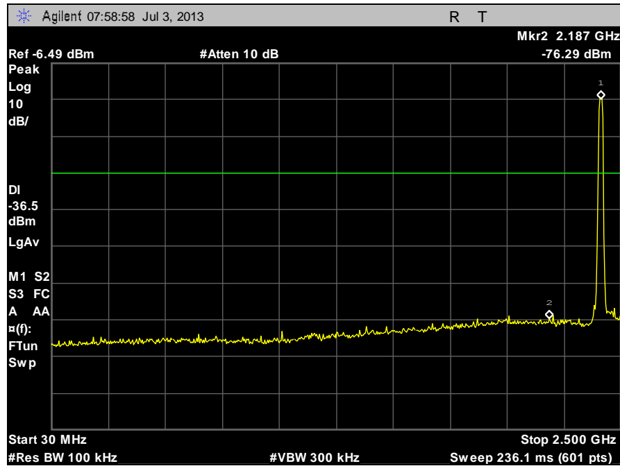
Plot 69. Conducted Spurious Emissions, Low Channel g, 30 MHz – 2.5 GHz
