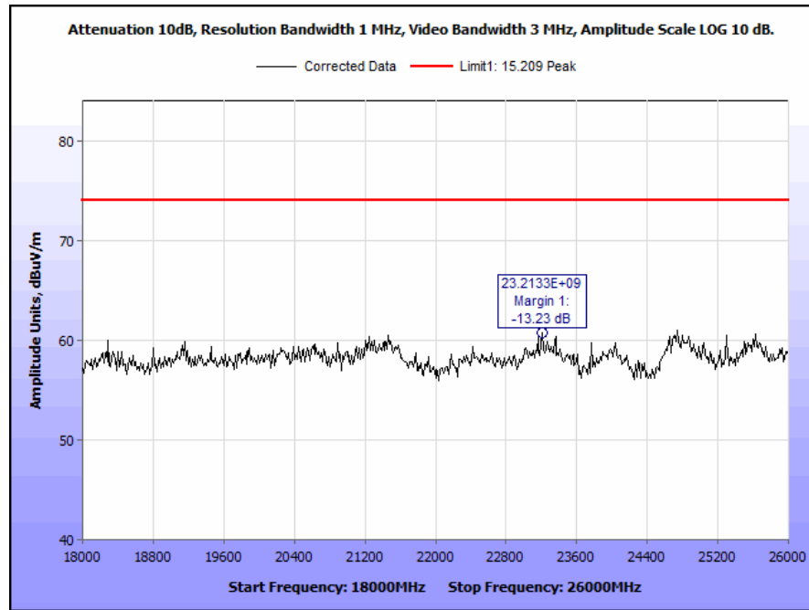
Plot 61. Radiated Spurious Emissions, High Channel b, 18 GHz to 26 GHz Peak
