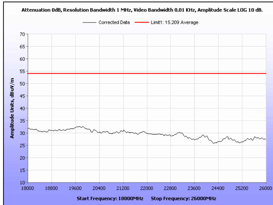
Plot 56. Radiated Spurious Emissions, High Channel g, 18 GHz to 26 GHz Average
