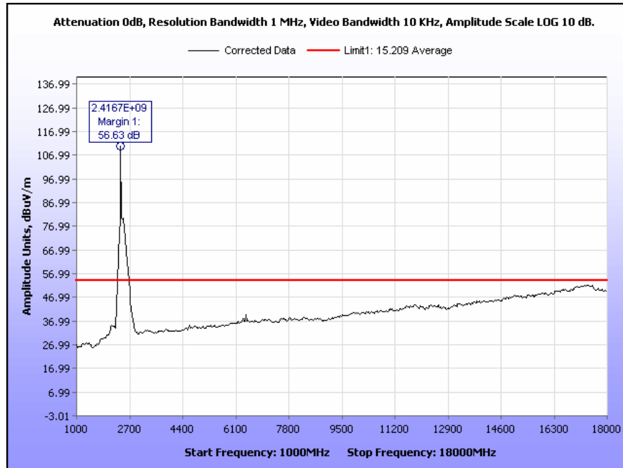
Plot 50. Radiated Spurious Emissions, Low Channel g, 1 GHz to 18 GHz Average
