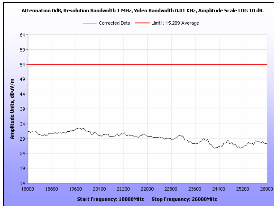
Plot 60. Radiated Spurious Emissions, Mid Channel g, 18 GHz to 26 GHz Average
