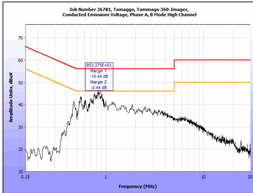
Plot 7. Conducted Emissions, 15.207(a), High Channel b Phase Line
