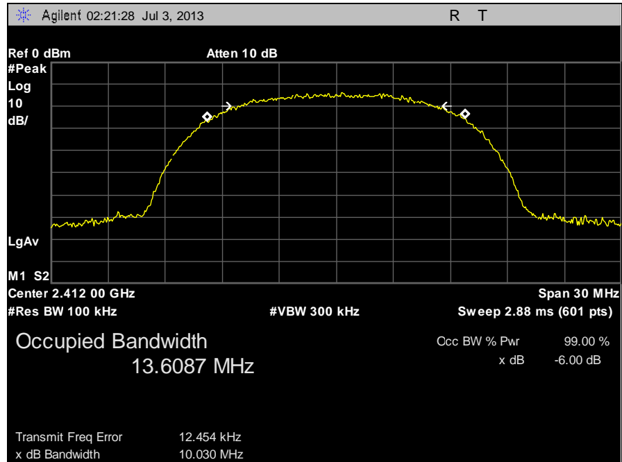
Plot 19. 6 dB Occupied Bandwidth, Low Channel b
