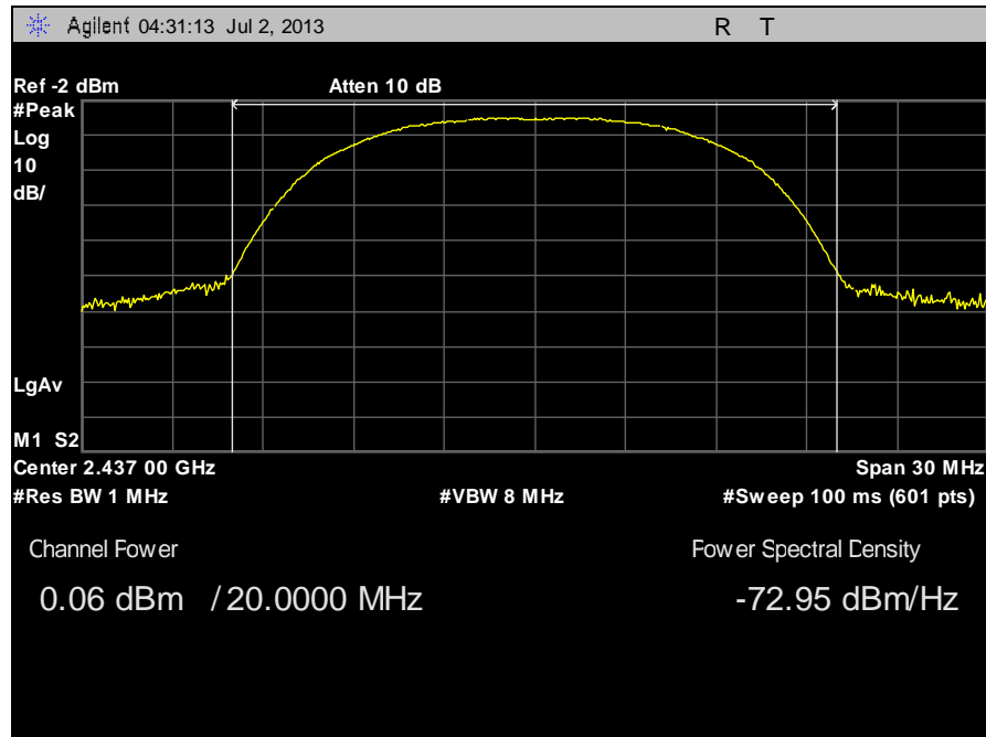
Plot 33. Peak Power Output, Channel 6 b
