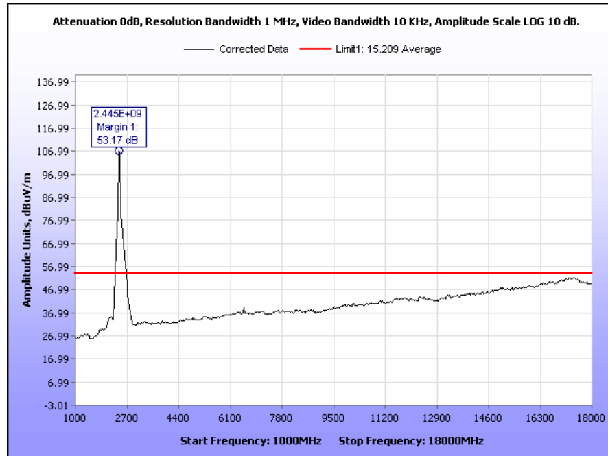
Plot 44. Radiated Spurious Emissions, High Channel b, 1 GHz to 18 GHz Average
