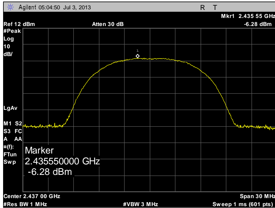
Plot 87. Peak Power Spectral Density, Mid Channel B, Full Signal Peak
