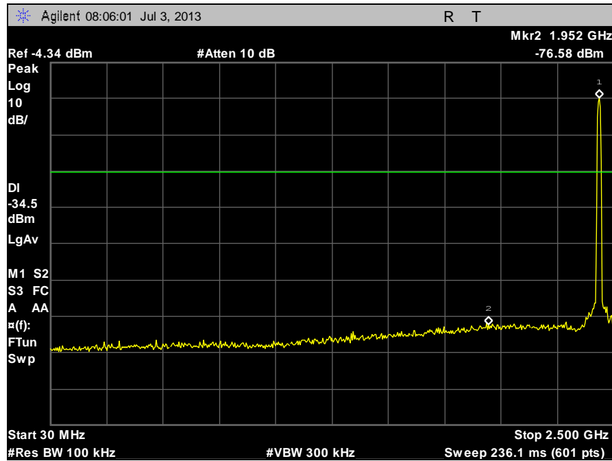
Plot 71. Conducted Spurious Emissions, Mid Channel b, 30 MHz – 2.5 GHz
