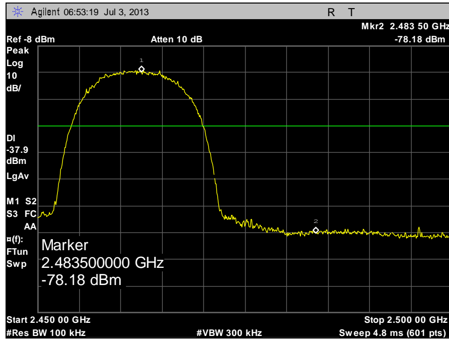
Plot 79. Conducted Spurious Emissions, High Channel b, Band Edge
