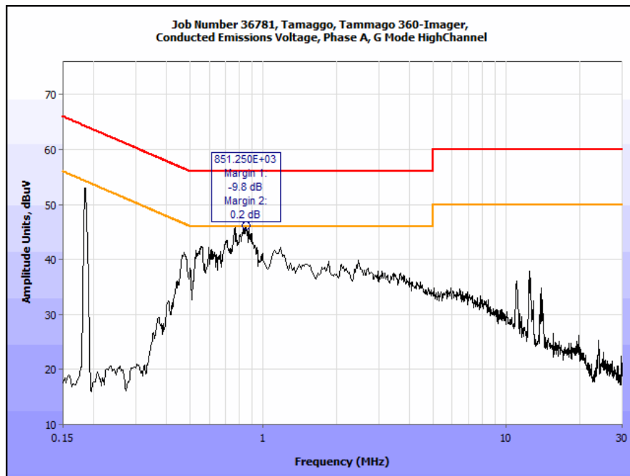
Plot 9. Conducted Emissions, 15.207(a), High Channel g Phase Line
