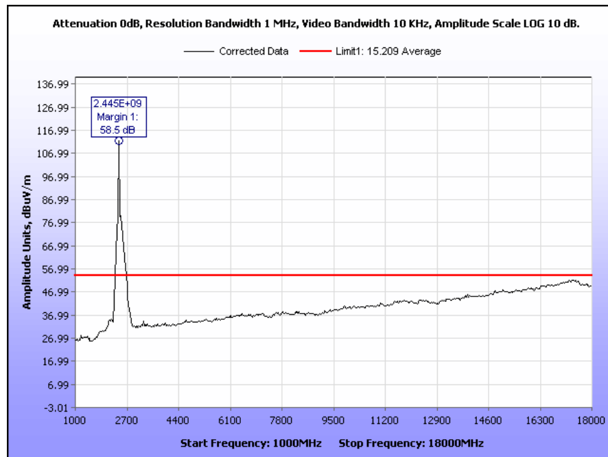
Plot 52. Radiated Spurious Emissions, Mid Channel b, 1 GHz to 18 GHz Average
