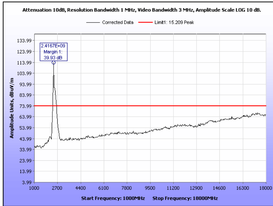
Plot 49. Radiated Spurious Emissions, Low Channel g, 1 GHz to 18 GHz
