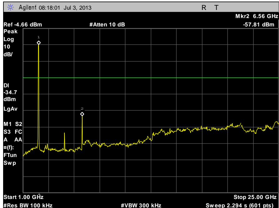
Plot 76. Conducted Spurious Emissions, High Channel b, 1 GHz to 25 GHz
