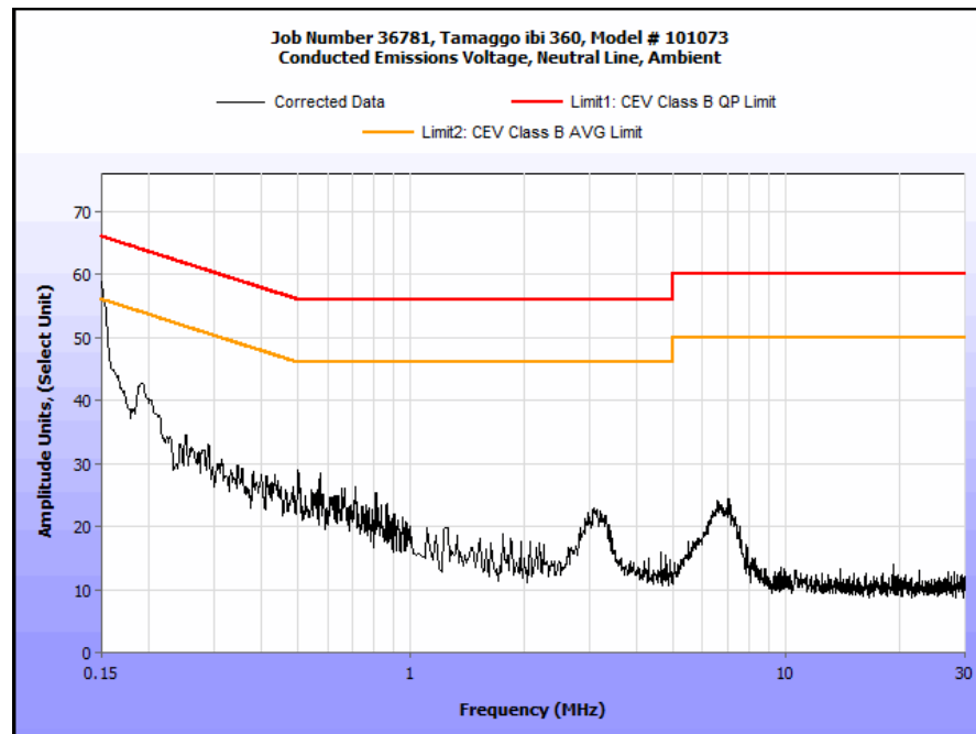
Plot 3. Conducted Emission, Neutral Line Plot, Ambient
