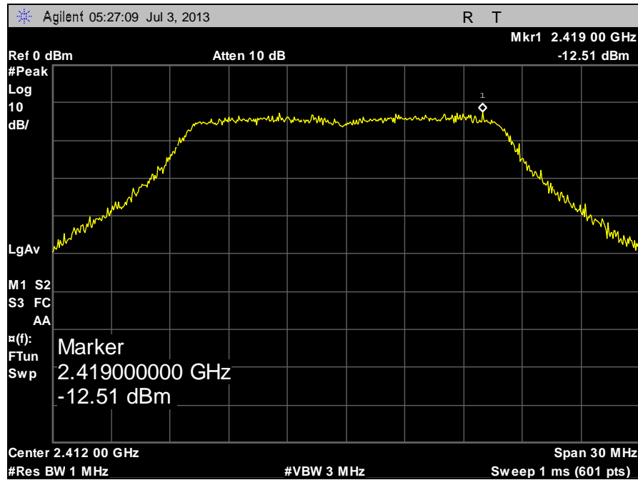
Plot 85. Peak Power Spectral Density, Low Channel G, Full Signal Peak
