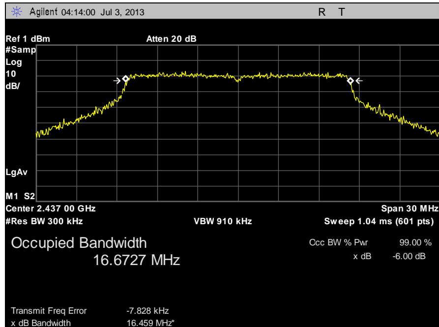
Plot 28. 99% Occupied Bandwidth, Mid Channel g
