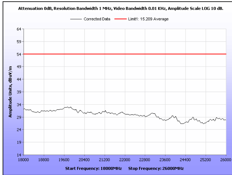
Plot 59. Radiated Spurious Emissions, Mid Channel b, 18 GHz to 26 GHz Average
