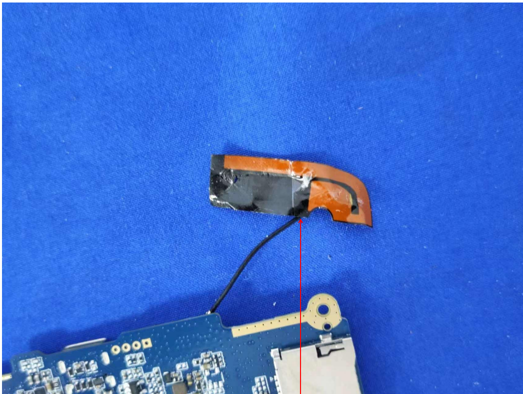
FPC Antenna
