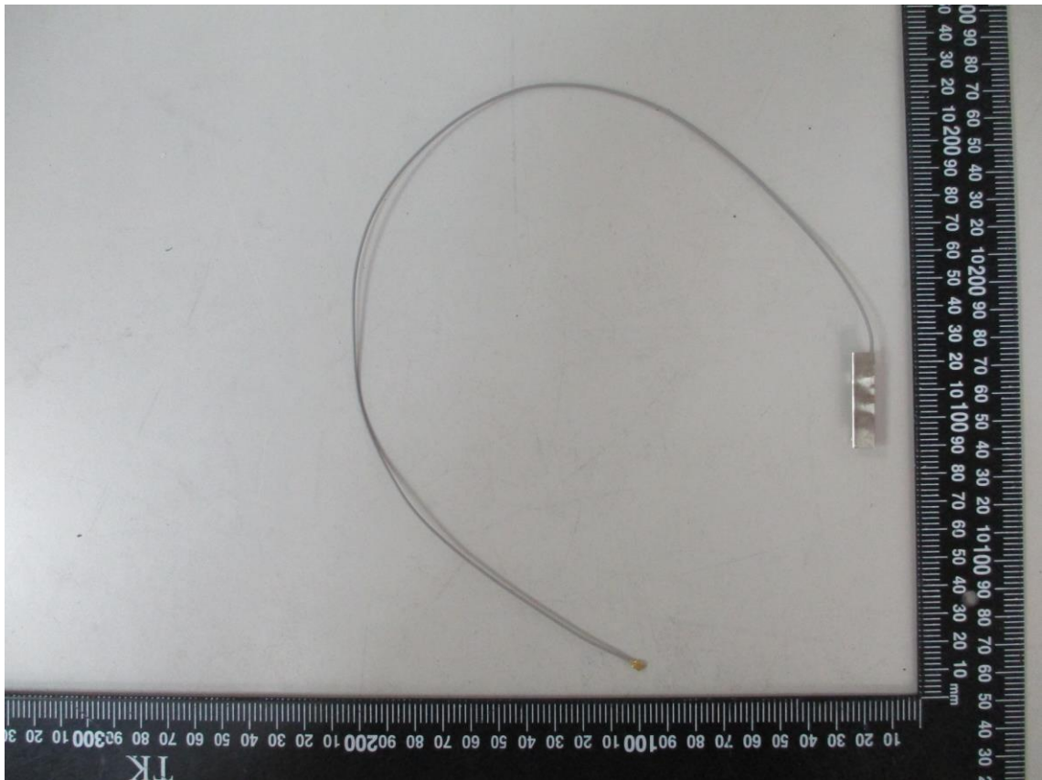
ANT+ Antenna
