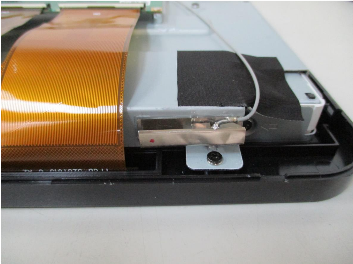
ANT+ Antenna
