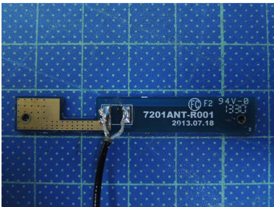
RX Antenna
