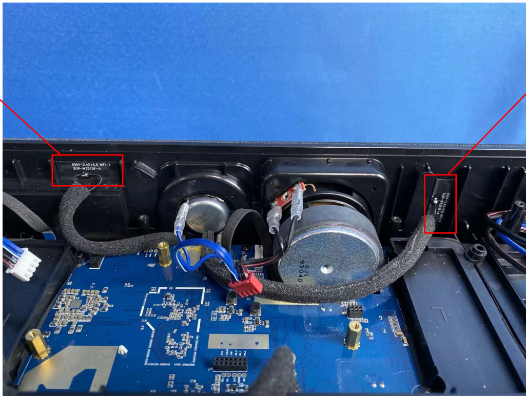
Bluetooth&2.4G& 5G WiFi Antenna
