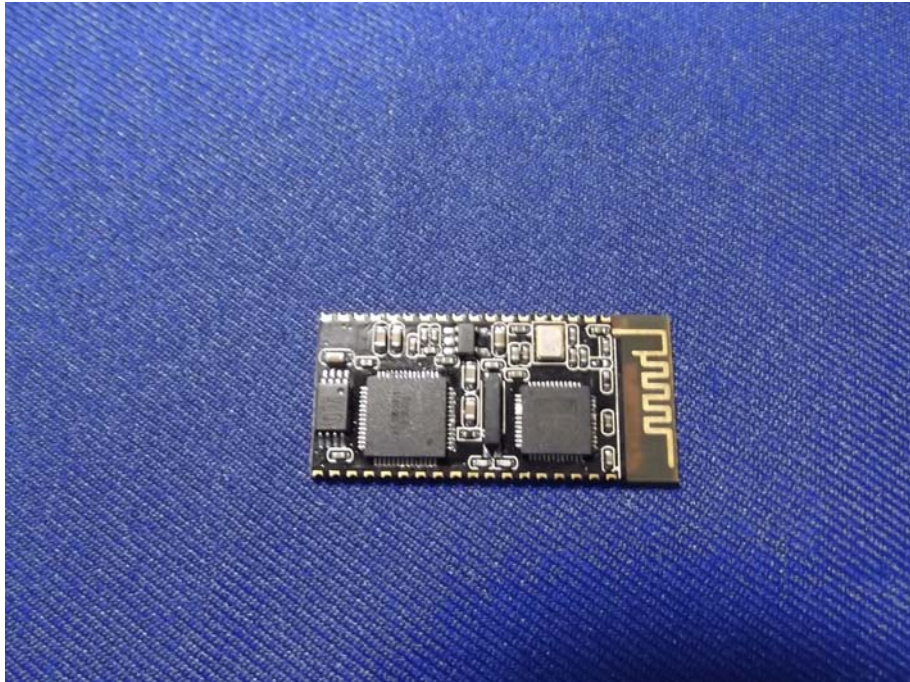
Figure 12 PCB of the BT Module-Front View
