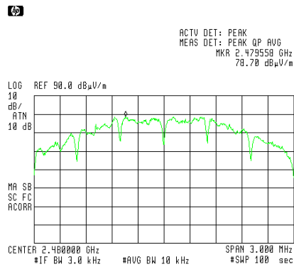
Figure 33 — High channel
