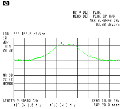
Figure 16 , Low channel , Vertical
