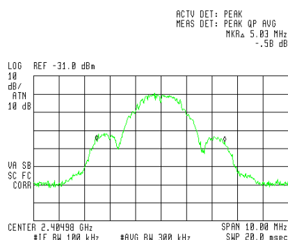
Figure 11 — Low Channel
