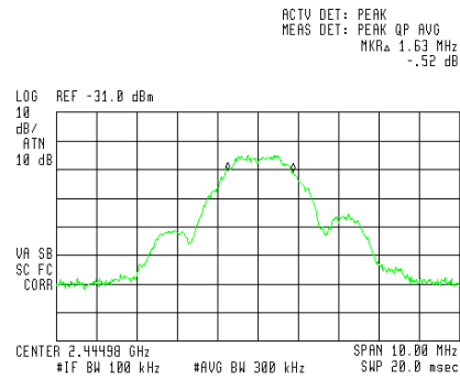
Figure 7 — Mid Channel
