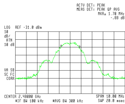
Figure 8 — High Channel
