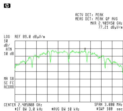
Figure 31 — Low Channel
