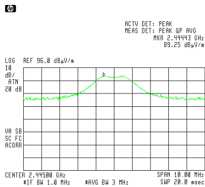
Figure 17, Mid channel , Vertical
