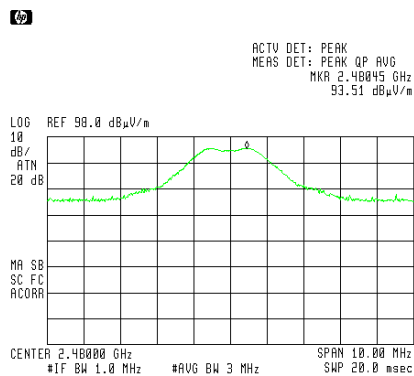
Figure 18 , High Channel, Vertical
