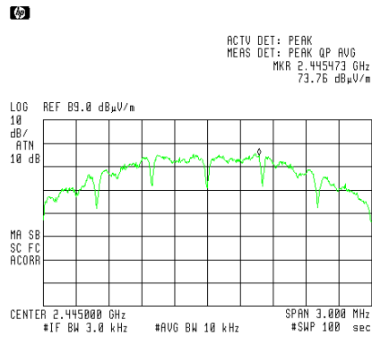
Figure 32 — Mid channel
