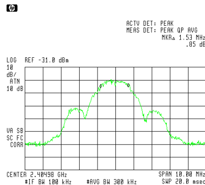
Figure 6 — Low Channel
