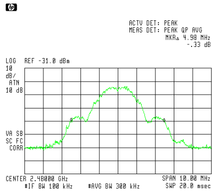
Figure 13 — High Channel
