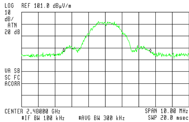
Figure 18 — High Channel
