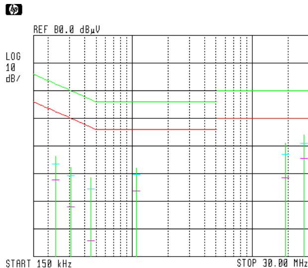
Figure 10 Detectors: Quasi-peak, Average
