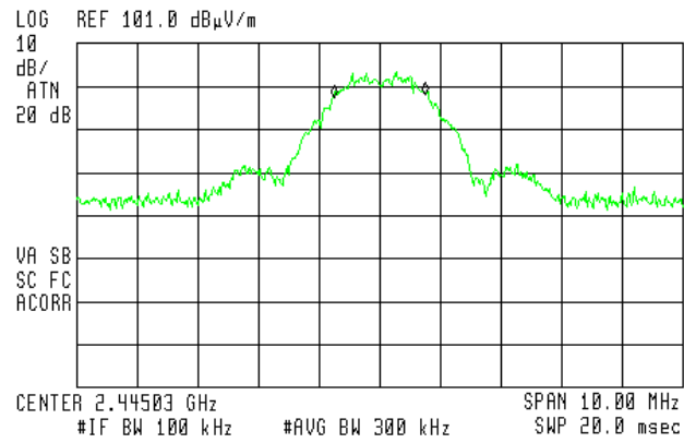
Figure 12 — Mid Channel
