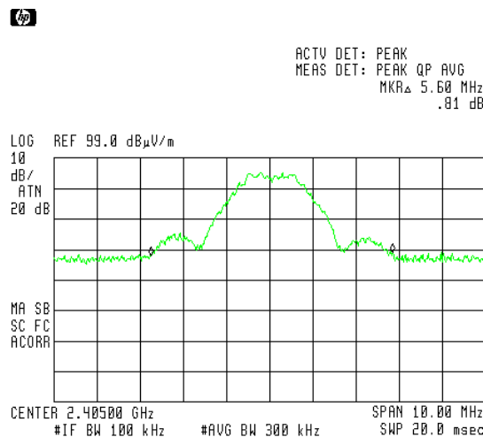
Figure 16 — Low Channel
