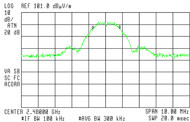
Figure 13 — High Channel
