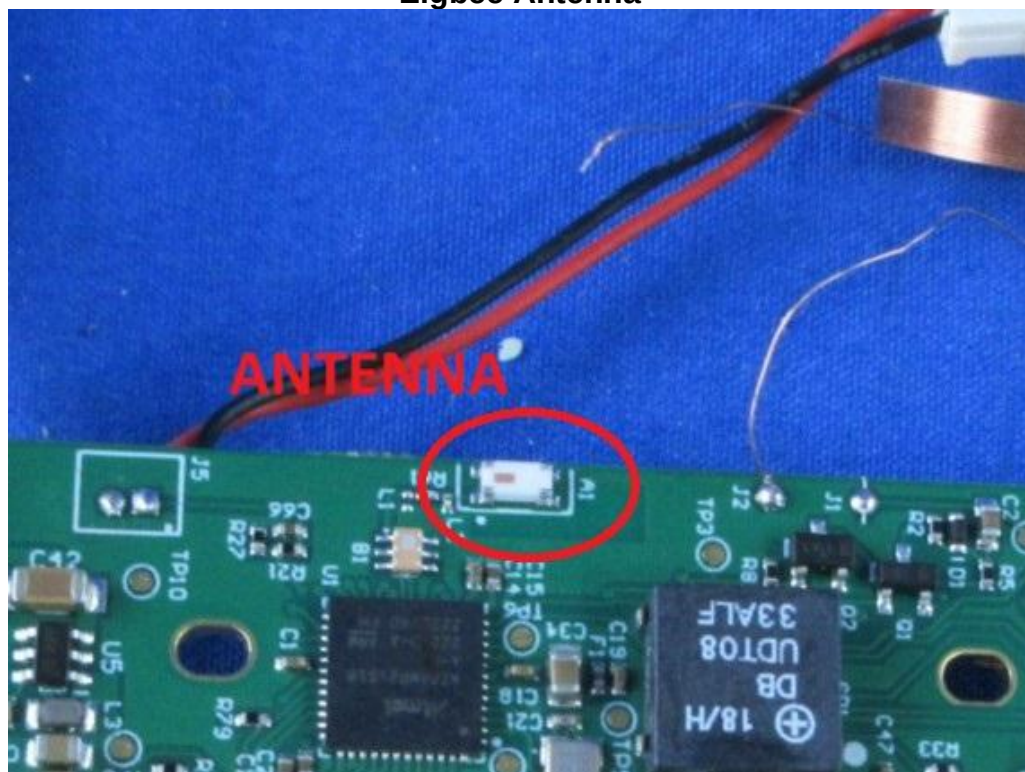
Zigbee Antenna
