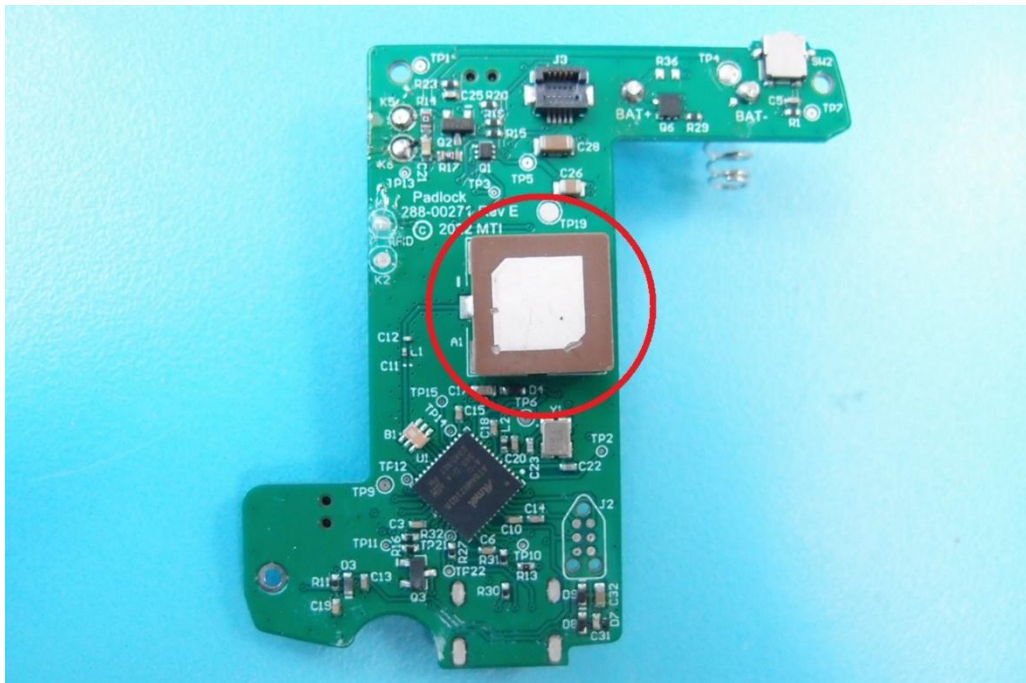
Zigbee Antenna
