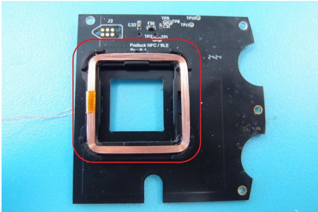
125 kHz Antenna
