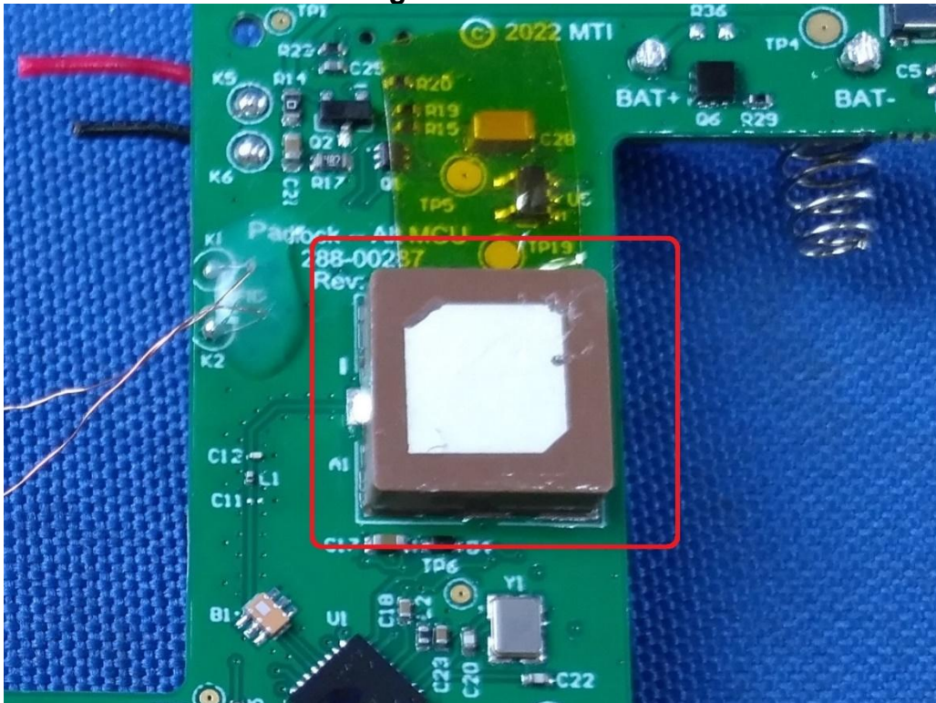
Zigbee Antenna
