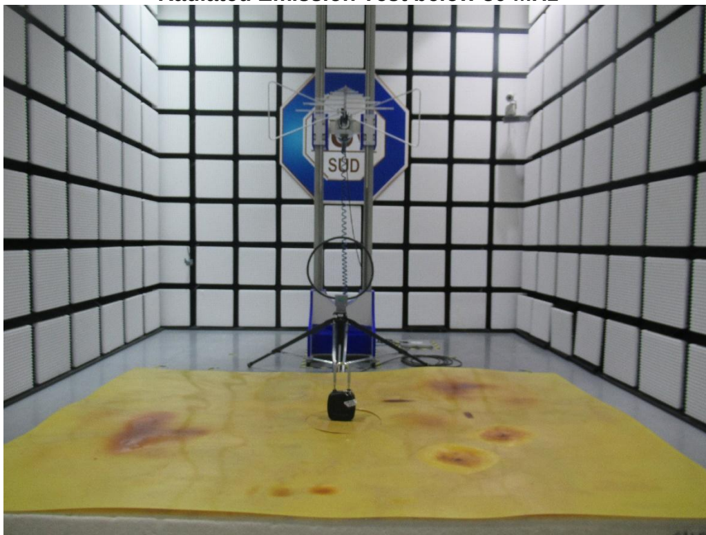
Radiated Emission Test below 30 MHz
