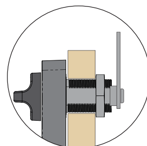
Straight Cam
