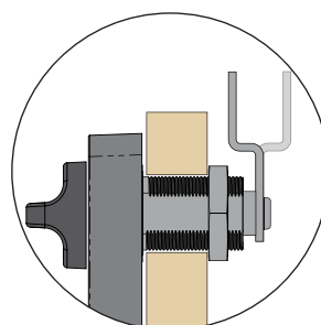
Offset Cam
