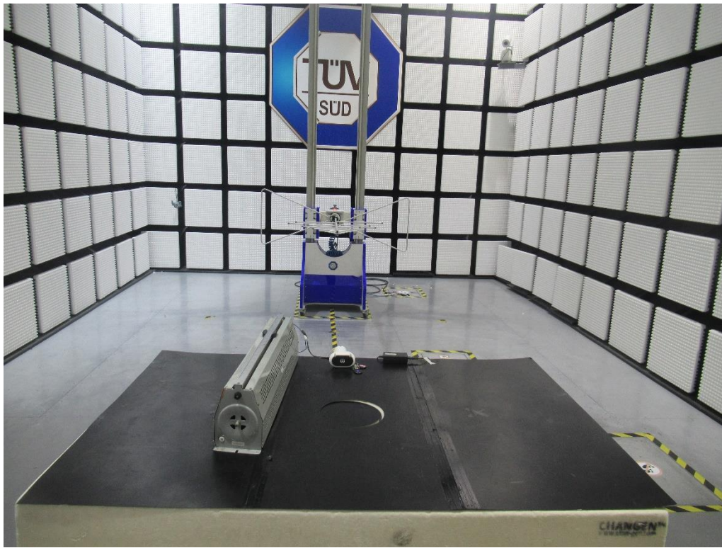
Radiated Emission Between 30MHz to 1GHz
