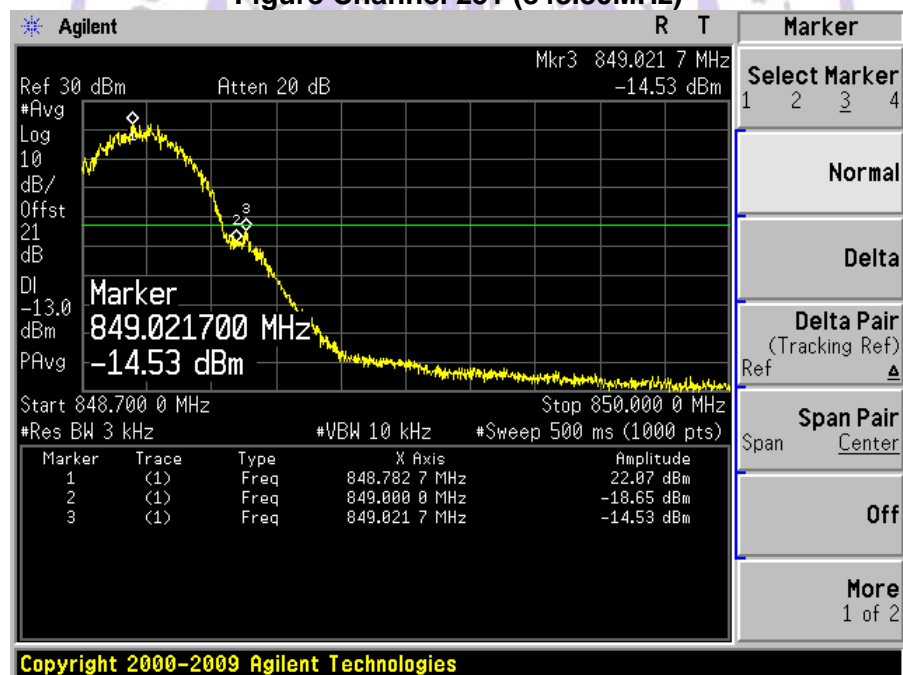
Figure Channel 251 (848.80MHz)
