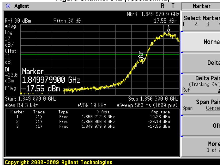
Figure Channel 512 (1850.20MHz)
