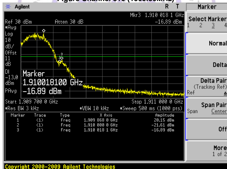
Figure Channel 810 (1909.80MHz)
