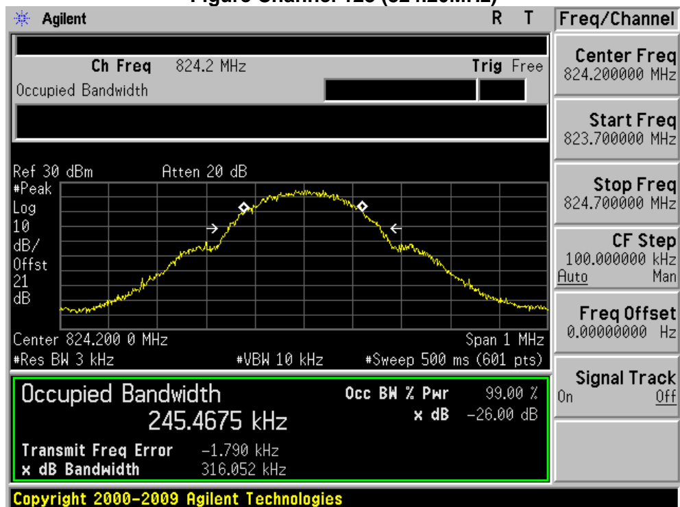
Figure Channel 128 (824.20MHz)
