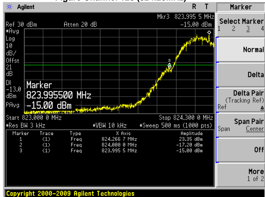
Figure Channel 128 (824.20MHz)
